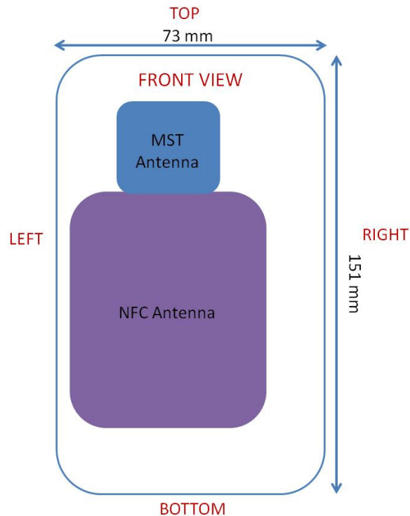
Figure F-2 NFC, MST Antenna Locations
