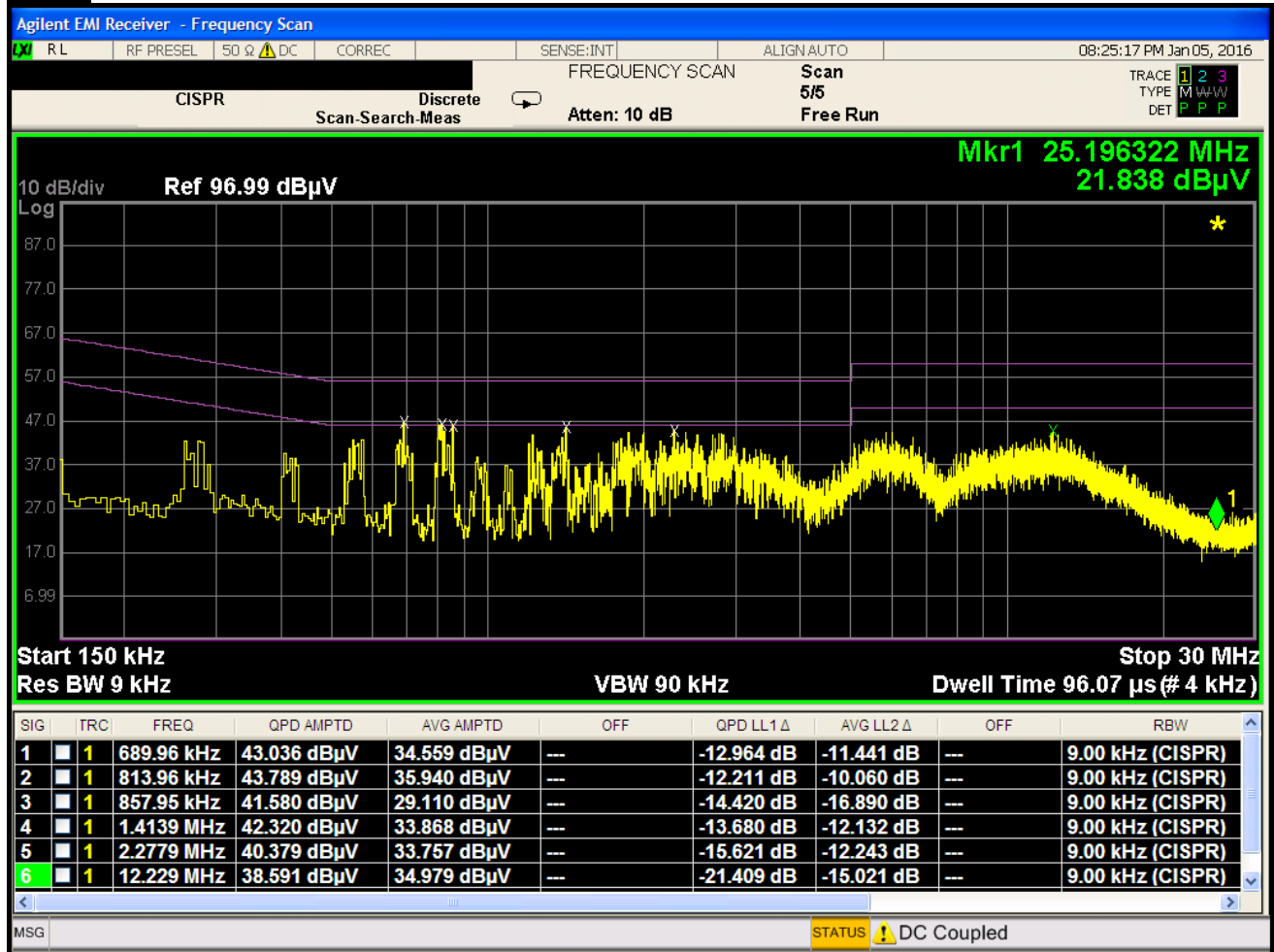
Plot 8-3. Line-Conducted Test Plot with RFID Antenna Terminated in 50Ω (L1)
