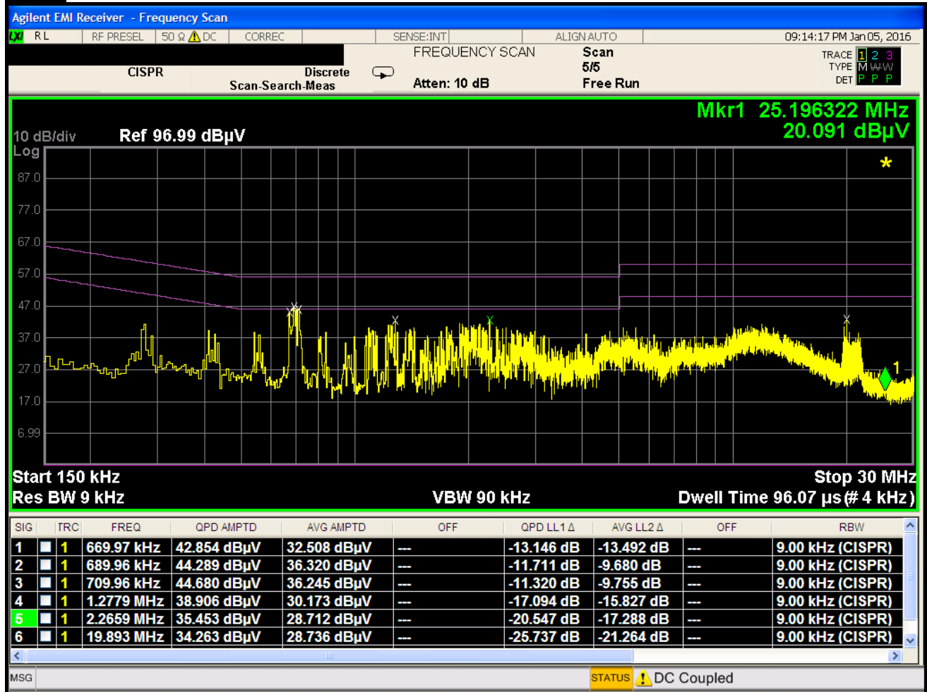
Plot 8-4. Line-Conducted Test Plot with RFID Antenna Terminated in 50Ω (N)
