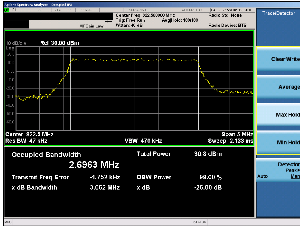
Plot 7-7. Occupied Bandwidth Plot (3MHz QPSK – RB Size 15– L High Channel)
