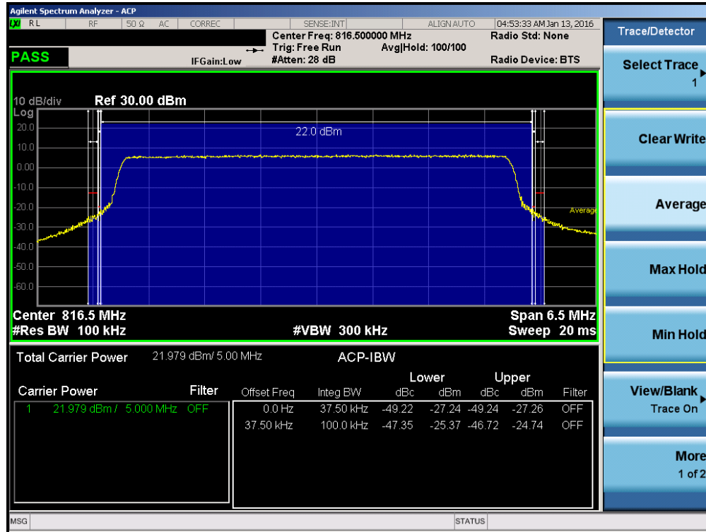
Plot 7-23. Channel Edge Plot (5MHz – RB Size 25– Low Channel)
