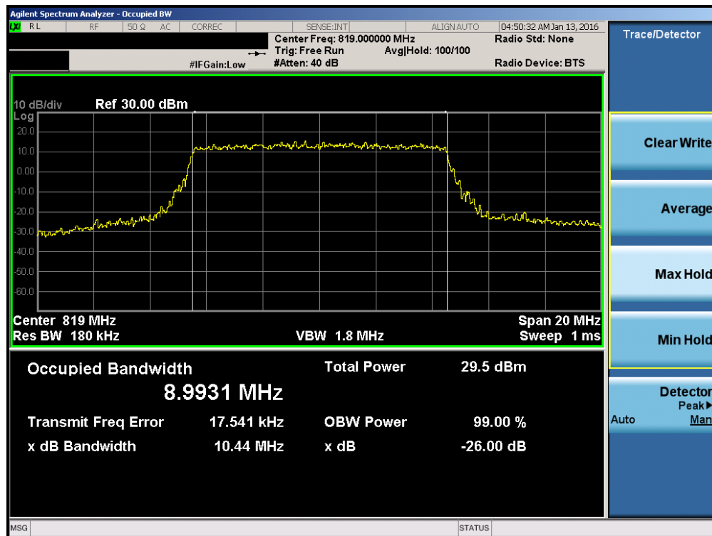
Plot 7-14. Occupied Bandwidth Plot (10MHz 16-QAM – RB Size 50)
