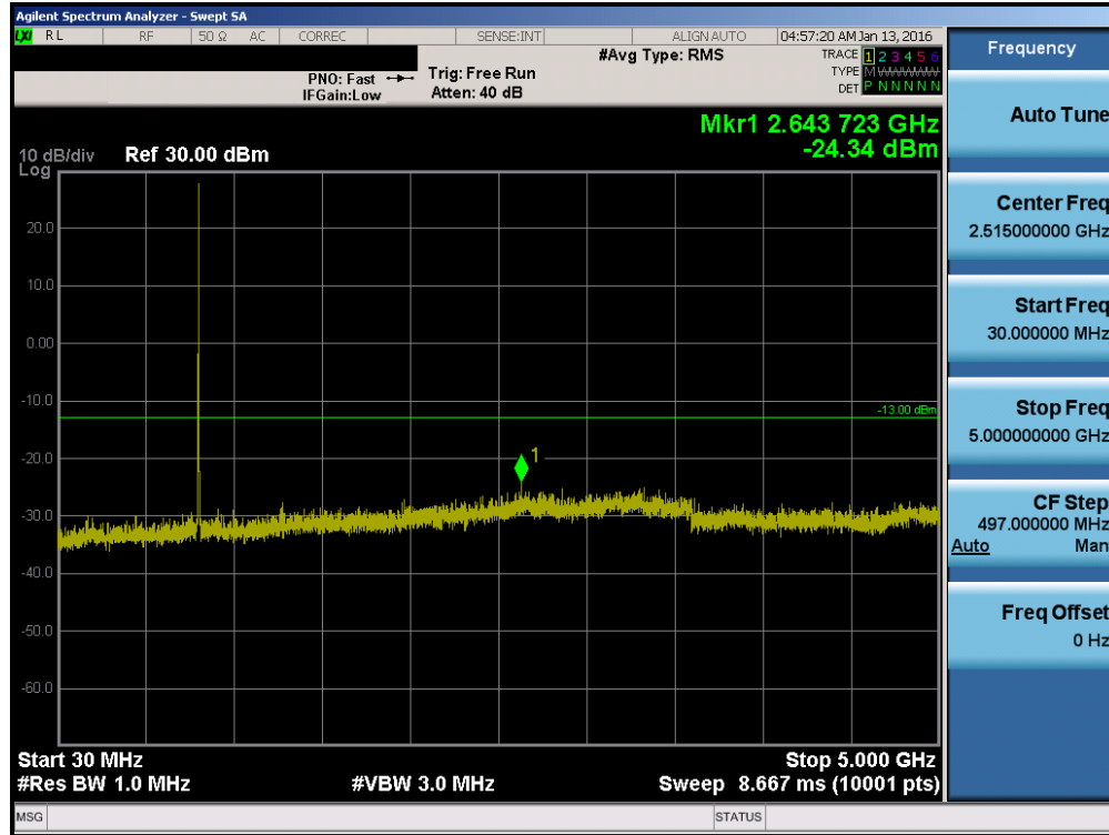
Plot 7-17. Conducted Spurious Plot (5.0MHz QPSK – RB Size 1, RB Offset 0 – High Channel)
