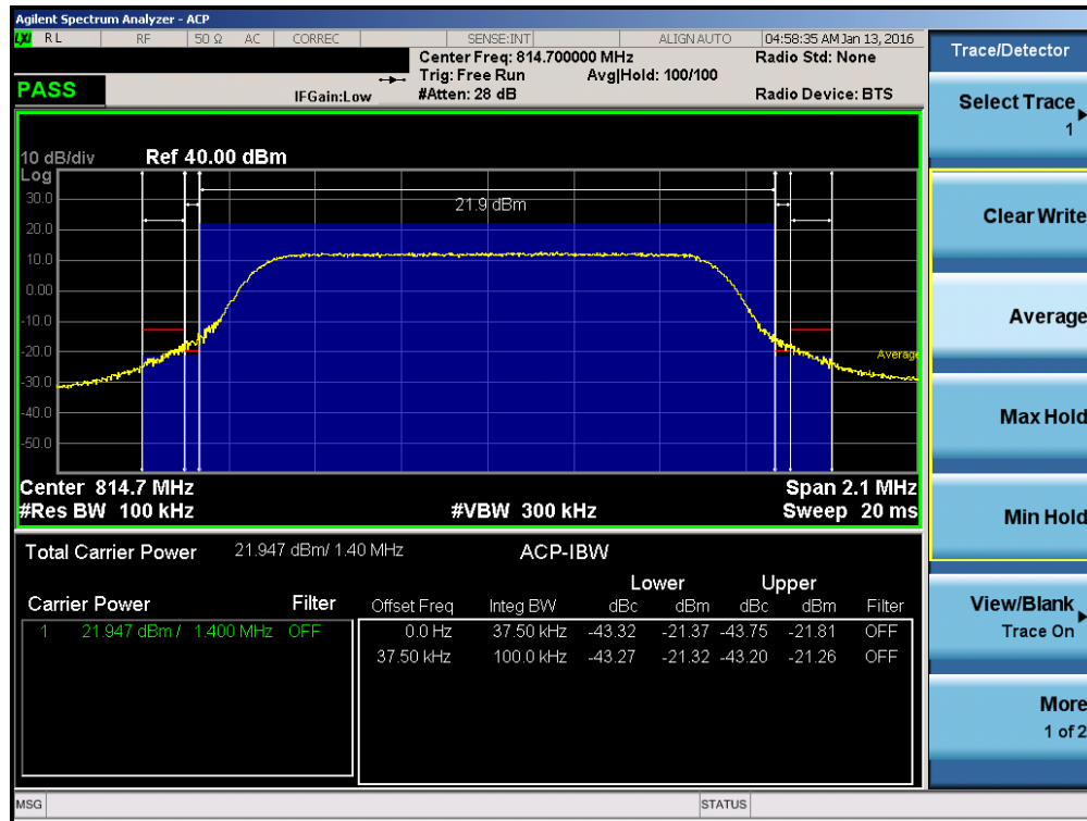
Plot 7-19. Channel Edge Plot (1.4MHz – RB Size 6– Low Channel)
