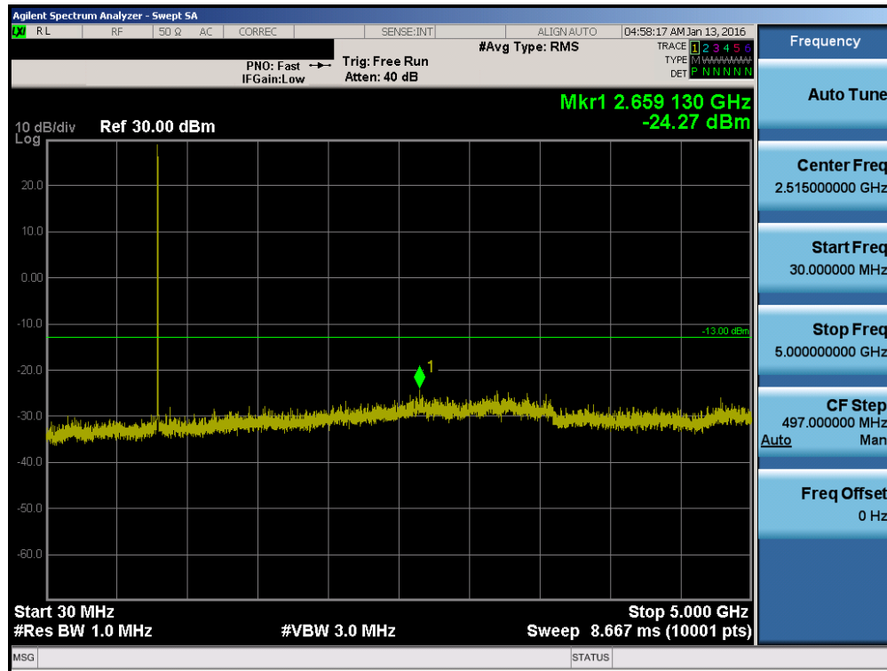
Plot 7-15. Conducted Spurious Plot (5.0MHz QPSK – RB Size 1, RB Offset 0 – Low Channel)
