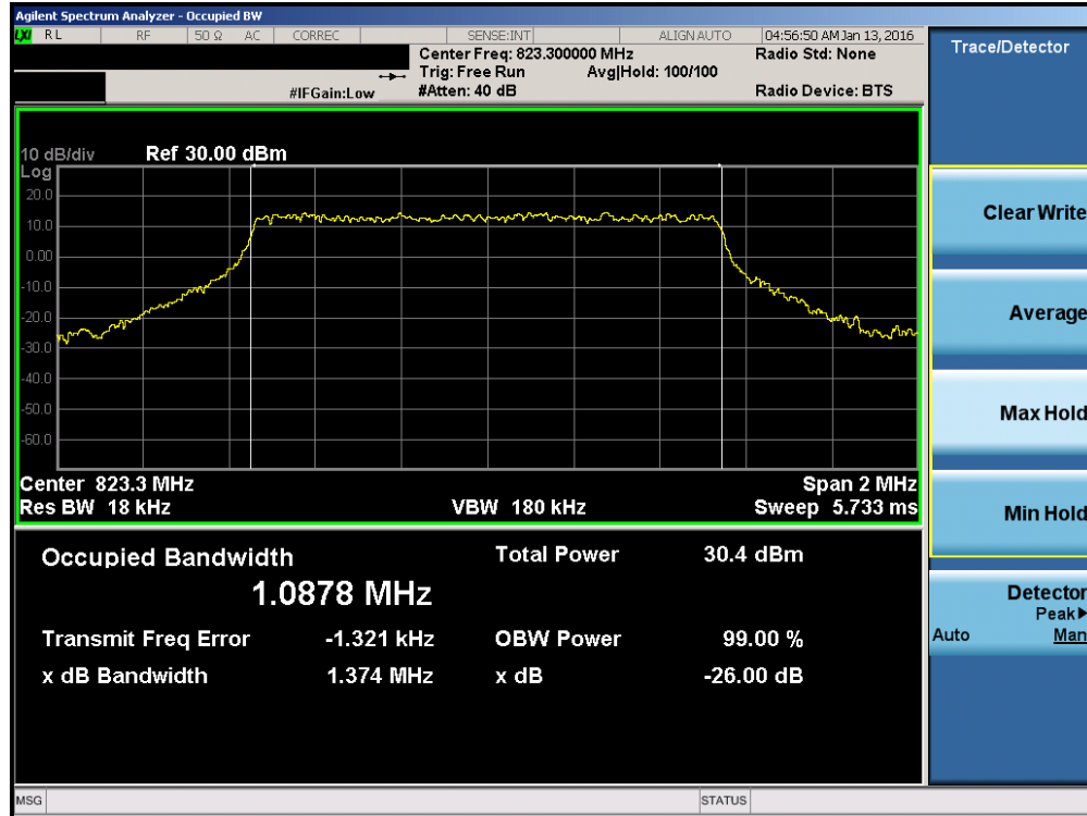
Plot 7-3. Occupied Bandwidth Plot (1.4MHz QPSK – RB Size 6– High Channel)
