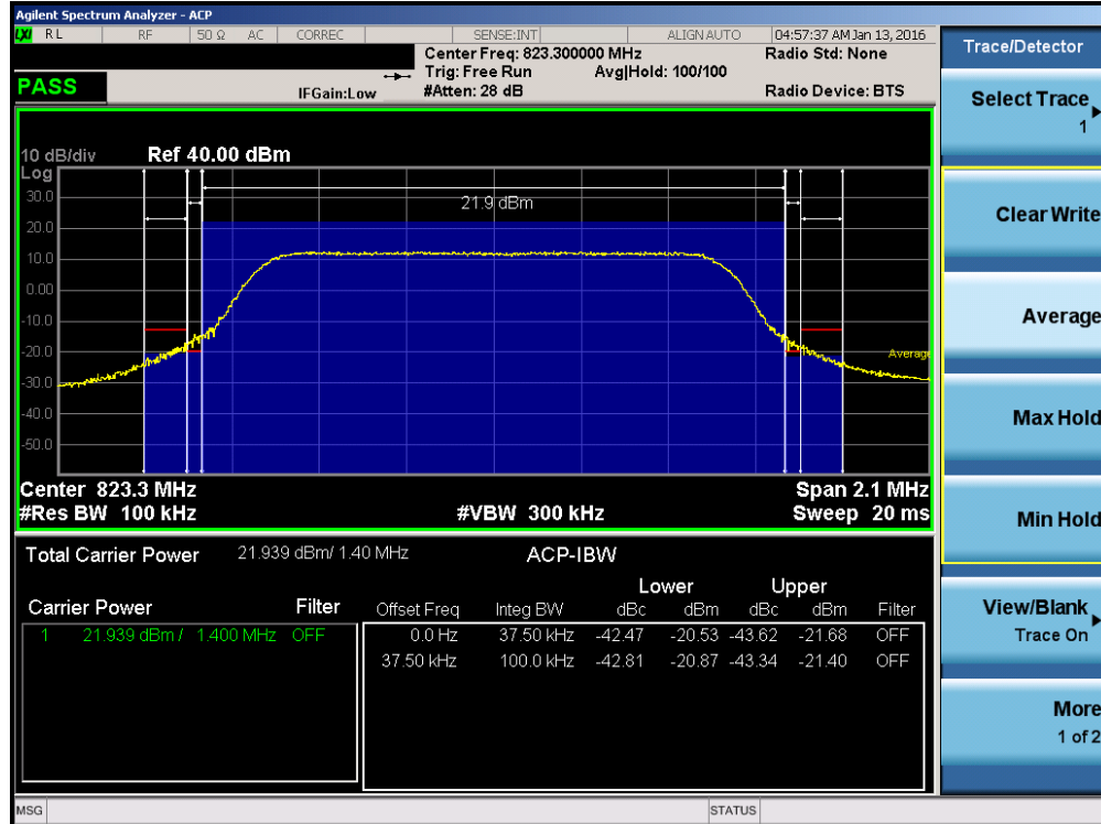
Plot 7-20. Channel Edge Plot (1.4MHz – RB Size 6 – High Channel)
