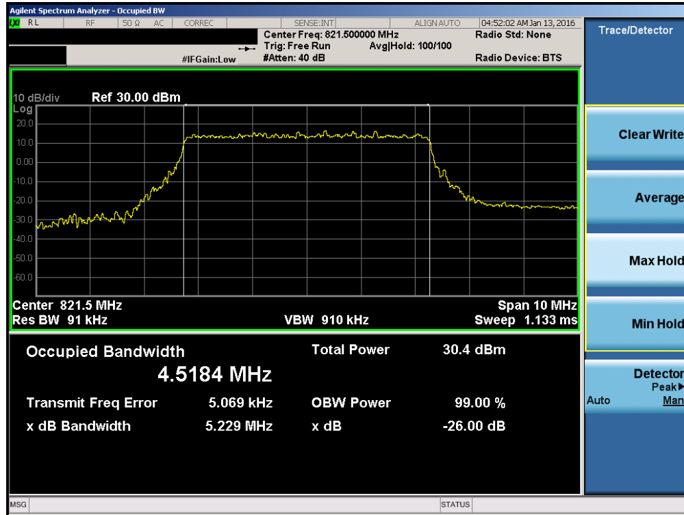
Plot 7-11. Occupied Bandwidth Plot (5MHz QPSK – RB Size 25– High Channel)
