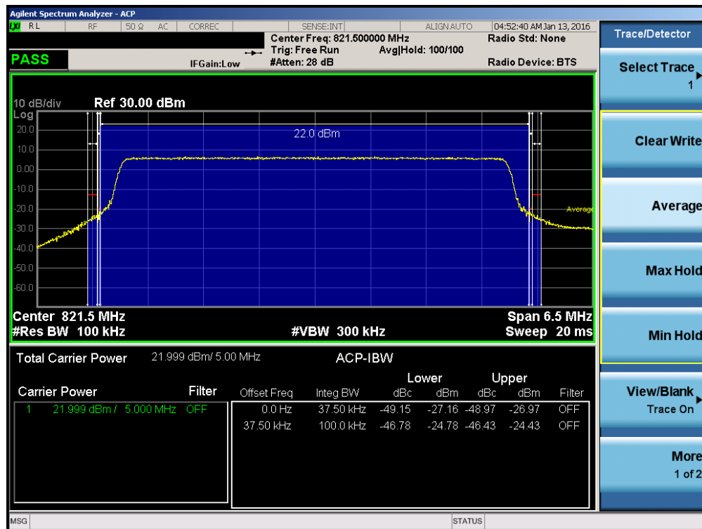
Plot 7-24. Channel Edge Plot (5MHz – RB Size 25 – High Channel)
