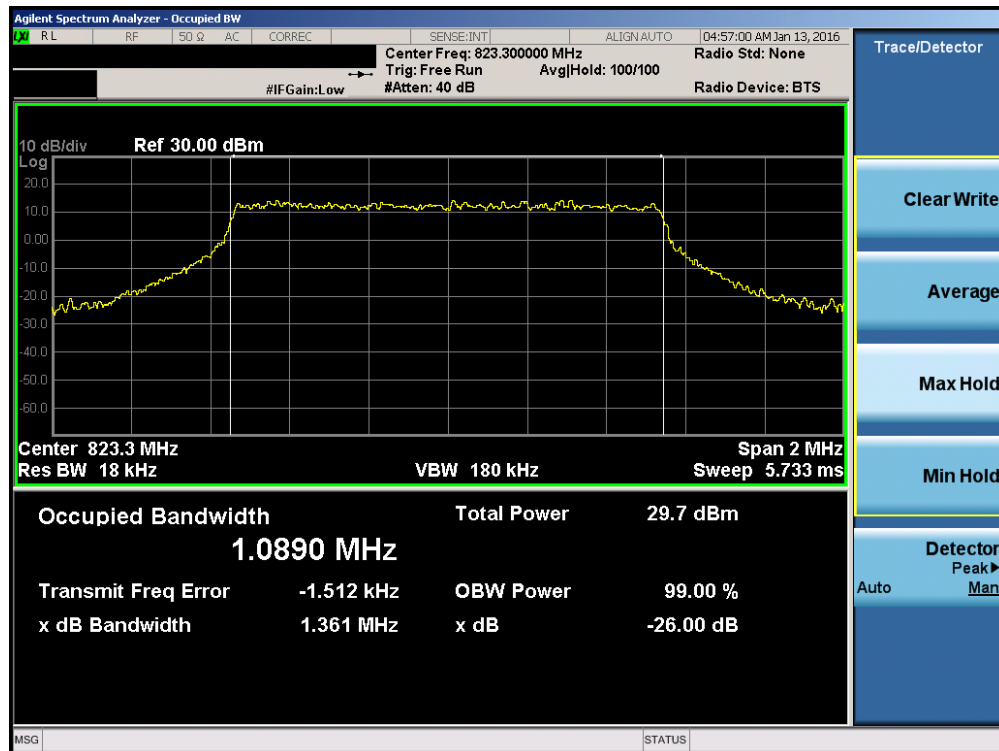
Plot 7-4. Occupied Bandwidth Plot (1.4MHz 16-QAM – RB Size 6– High Channel)
