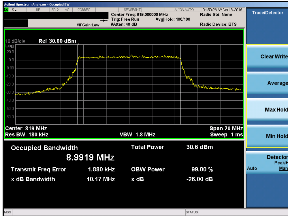
Plot 7-13. Occupied Bandwidth Plot (10MHz QPSK – RB Size 50)
