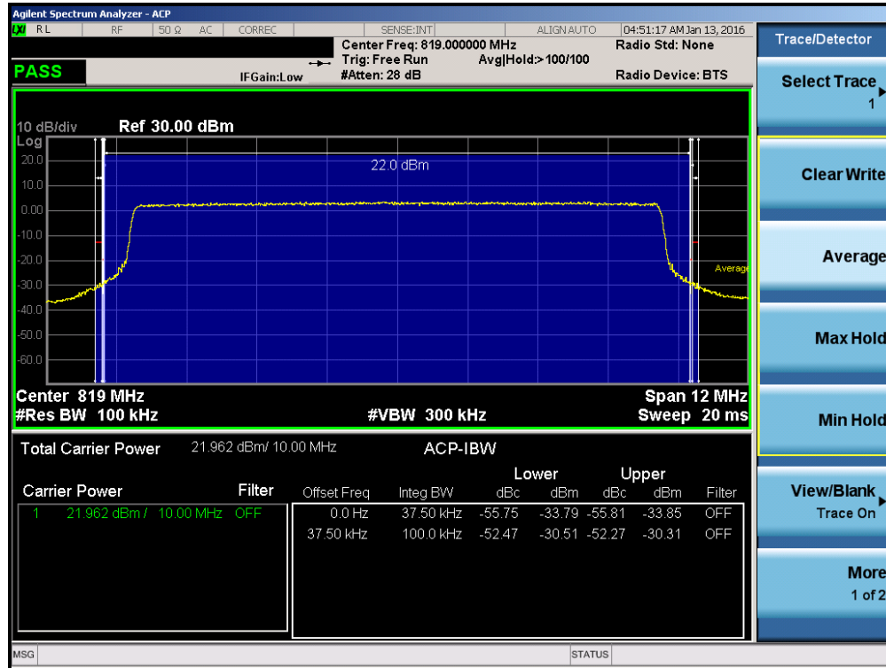
Plot 7-25. Channel Edge Plot (10MHz – RB Size 50)
