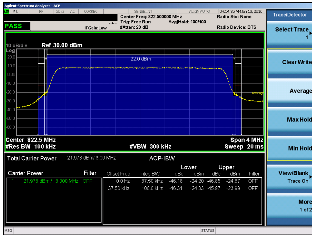
Plot 7-22. Channel Edge Plot (3MHz – RB Size 15 – High Channel)
