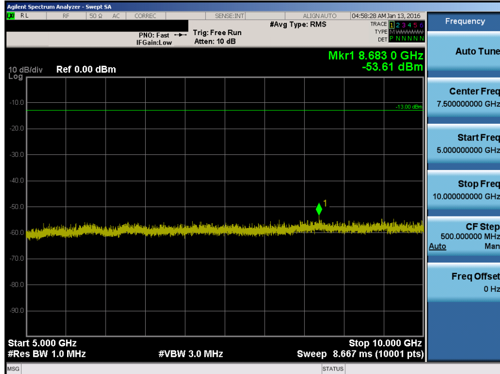
Plot 7-16. Conducted Spurious Plot (5.0MHz QPSK – RB Size 1, RB Offset 0 – Low Channel)
