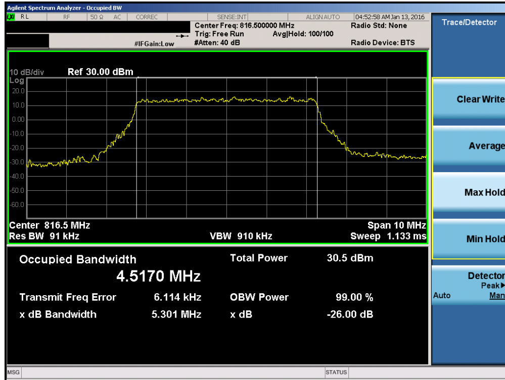
Plot 7-9. Occupied Bandwidth Plot (5MHz QPSK – RB Size 25– Low Channel)
