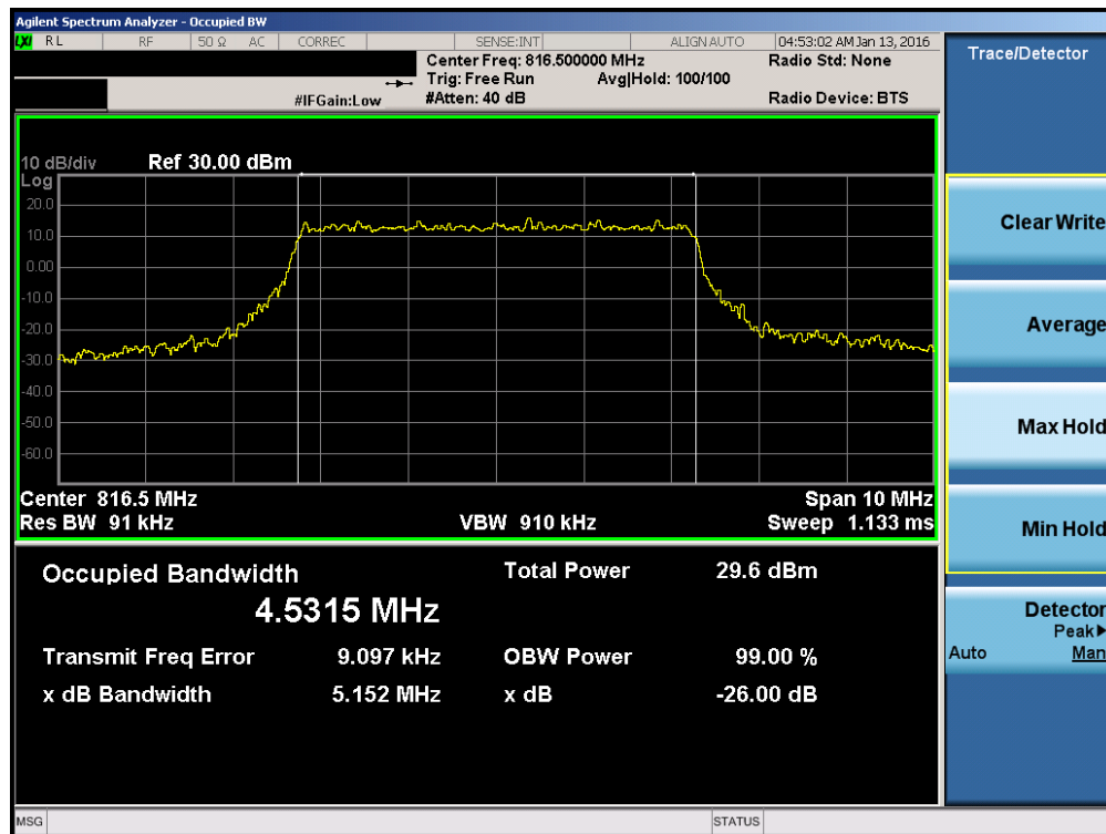
Plot 7-10. Occupied Bandwidth Plot (5MHz 16-QAM – RB Size 25– Low Channel)
