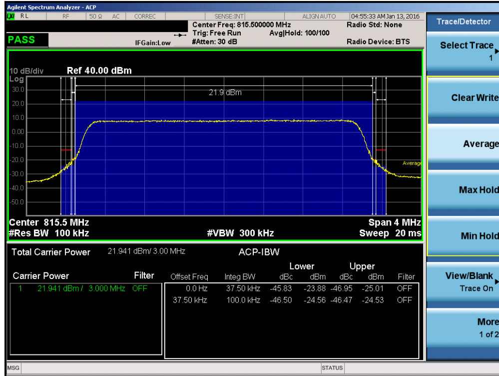
Plot 7-21. Channel Edge Plot (3MHz – RB Size 15– Low Channel)
