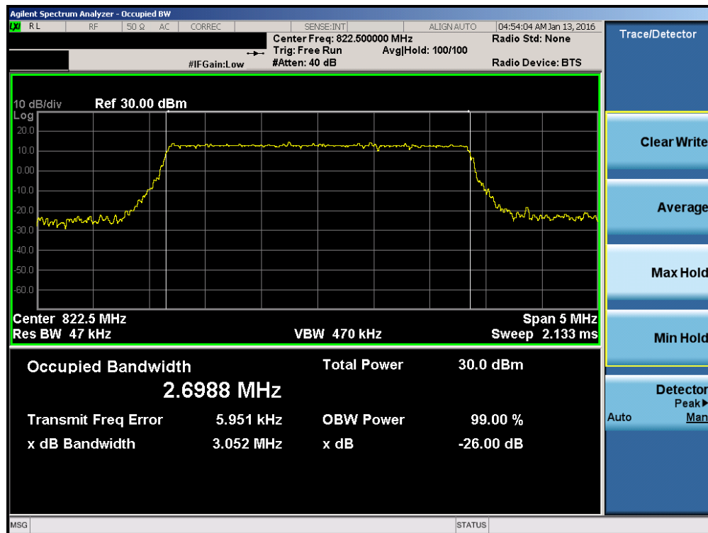
Plot 7-8. Occupied Bandwidth Plot (3MHz 16-QAM – RB Size 15– High Channel)
