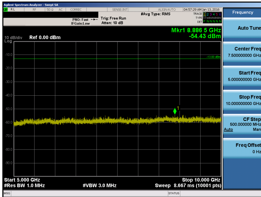
Plot 7-18. Conducted Spurious Plot (5.0MHz QPSK – RB Size 1, RB Offset 0 – High Channel)
