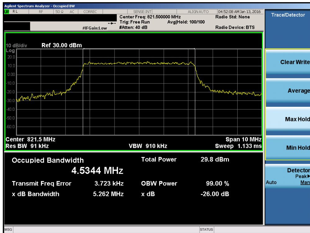
Plot 7-12. Occupied Bandwidth Plot (5MHz 16-QAM – RB Size 25– High Channel)
