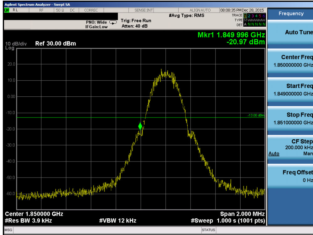
Plot 7-32. Band Edge Plot (PCS GSM Mode – Ch. 512)
