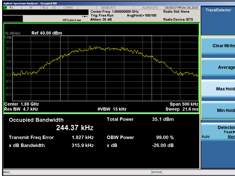
Plot 7-1. Occupied Bandwidth Plot (PCS GSM Mode – Ch. 661)
