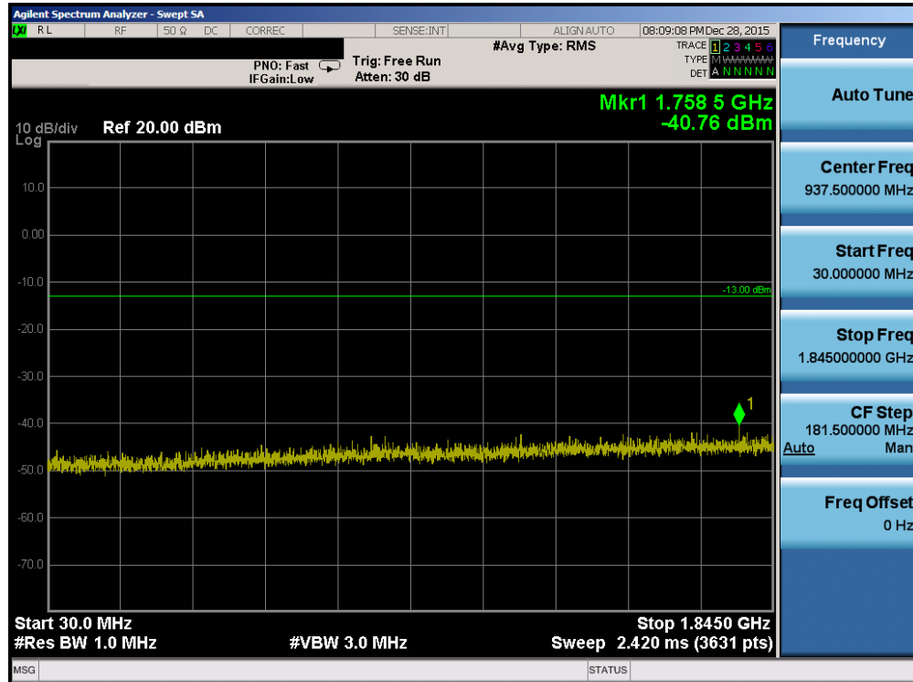
Plot 7-5. Conducted Spurious Plot (PCS GSM Mode – Ch. 512)
