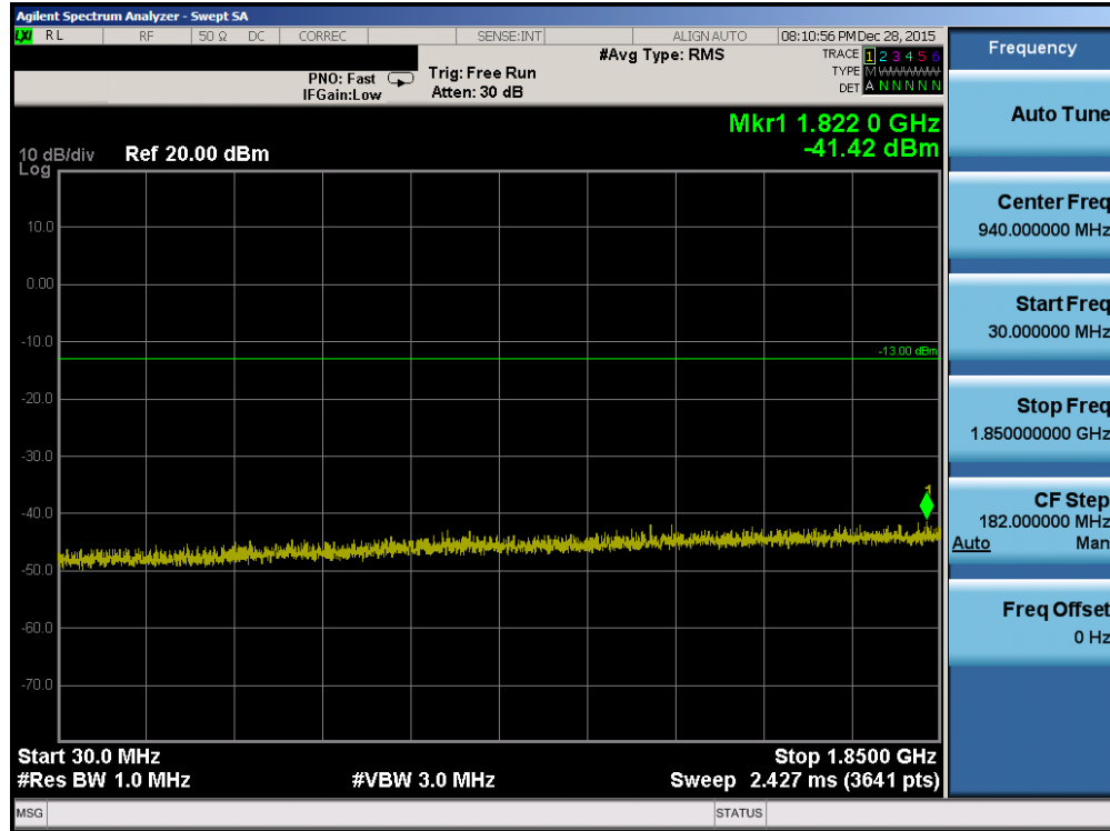
Plot 7-11. Conducted Spurious Plot (PCS GSM Mode – Ch. 810)
