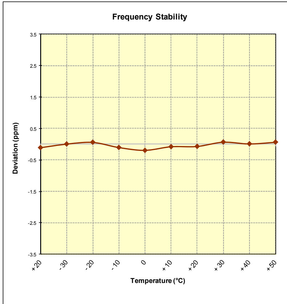
Figure 7-9. Frequency Stability Graph (PCS GSM Mode – Ch. 661)
