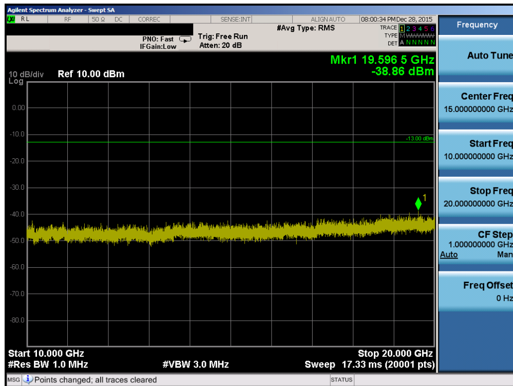
Plot 7-10. Conducted Spurious Plot (PCS GSM Mode – Ch. 661)
