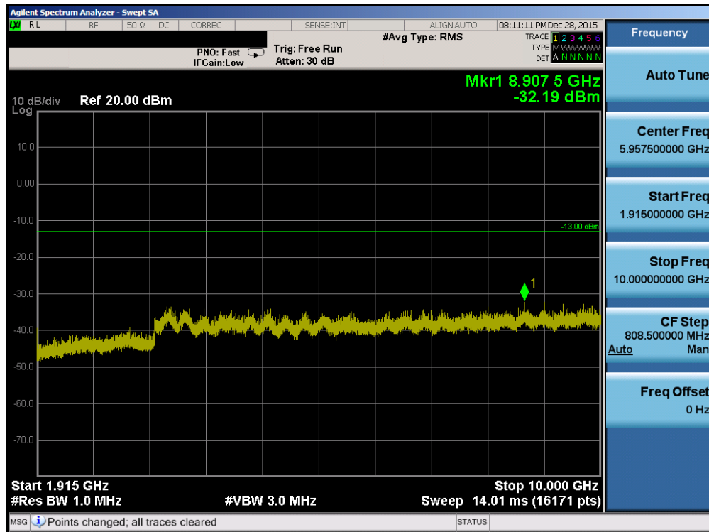
Plot 7-12. Conducted Spurious Plot (PCS GSM Mode – Ch. 810)
