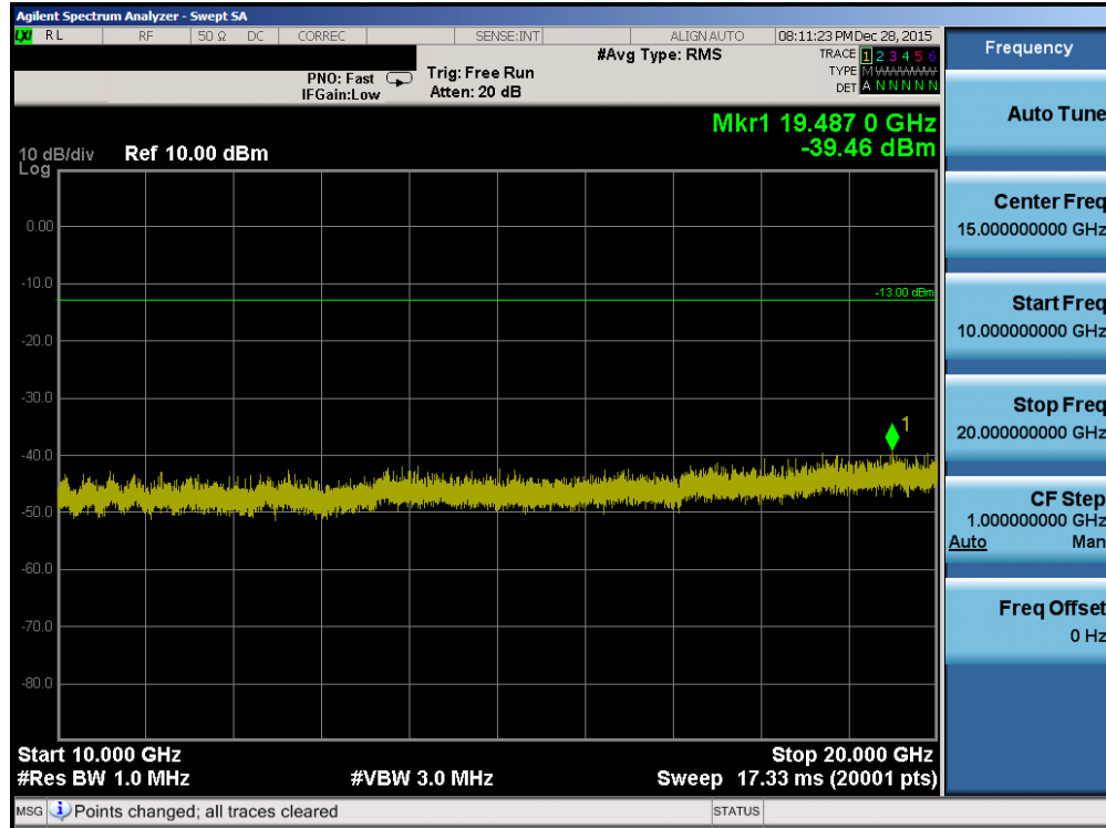
Plot 7-13. Conducted Spurious Plot (PCS GSM Mode – Ch. 810)
