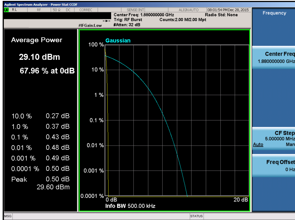
Plot 7-42. Peak-Average Ratio Plot (PCS GSM Mode – Ch. 661)
