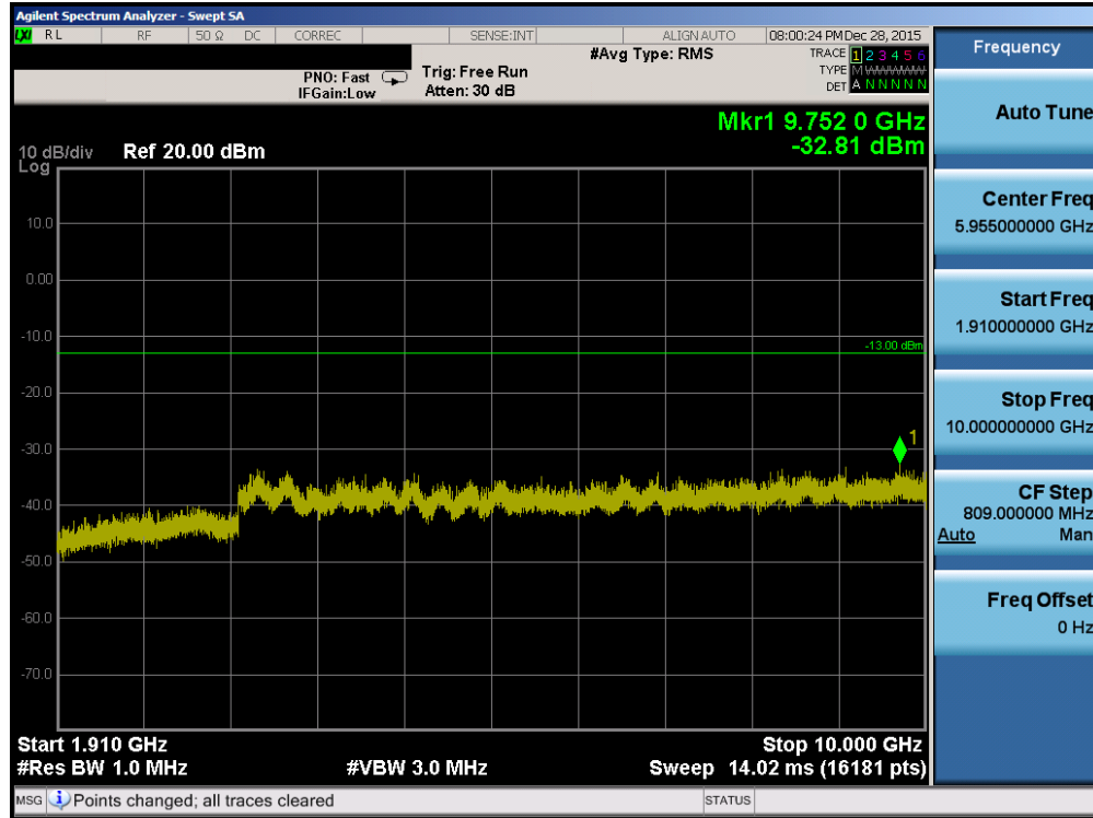
Plot 7-9. Conducted Spurious Plot (PCS GSM Mode – Ch. 661)
