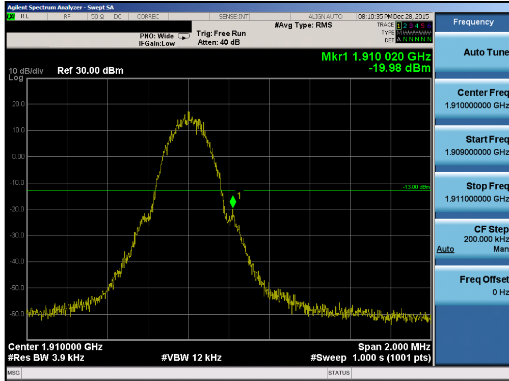
Plot 7-34. Band Edge Plot (PCS GSM Mode – Ch. 810)
