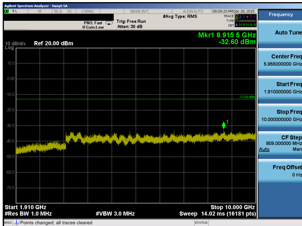
Plot 7-6. Conducted Spurious Plot (PCS GSM Mode – Ch. 512)
