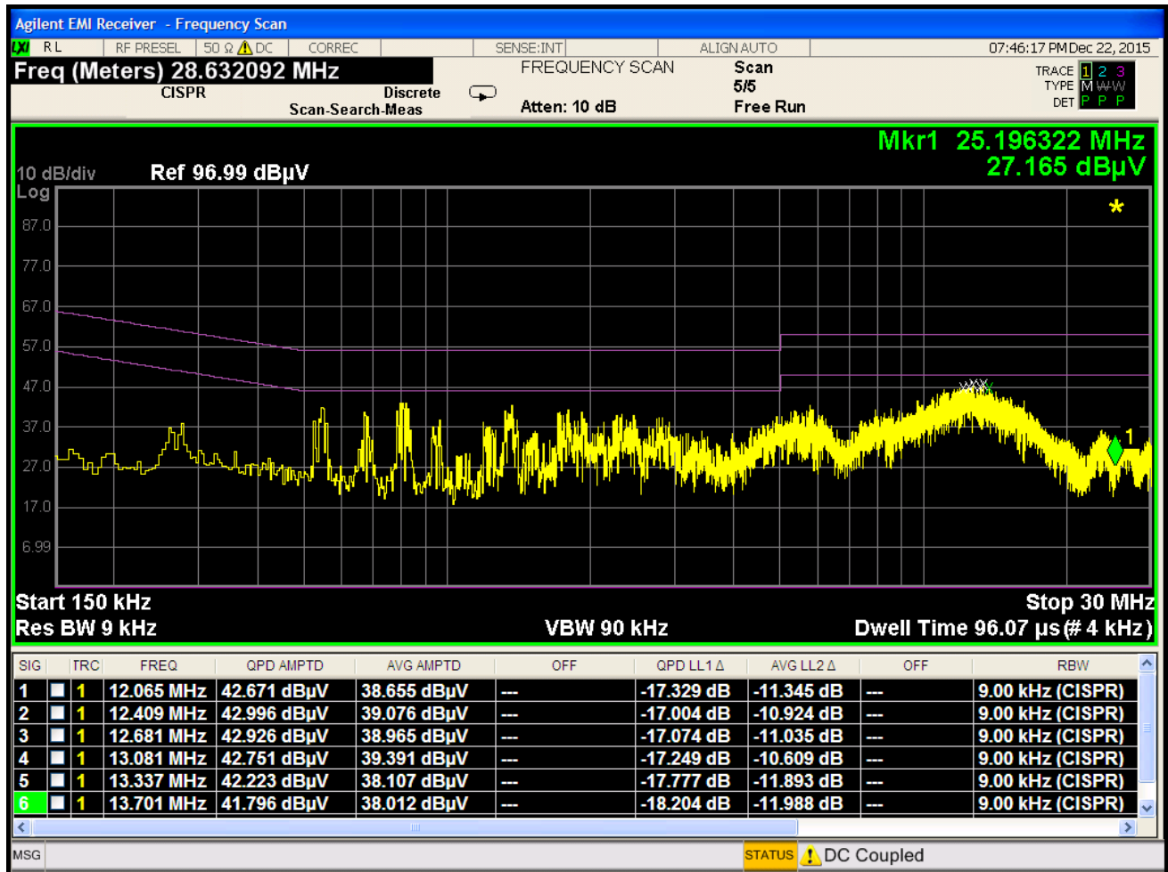
Plot 7-91. Line Conducted Plot with 802.11b (L1)
