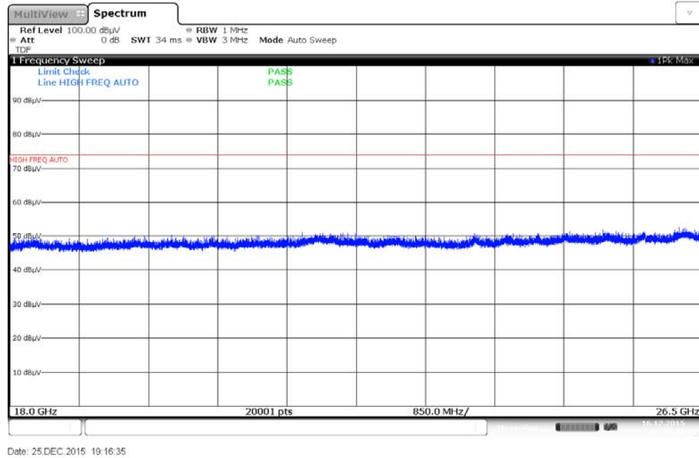
Plot 7-75. Radiated Spurious Plot above 18GHz (Pol. H)
