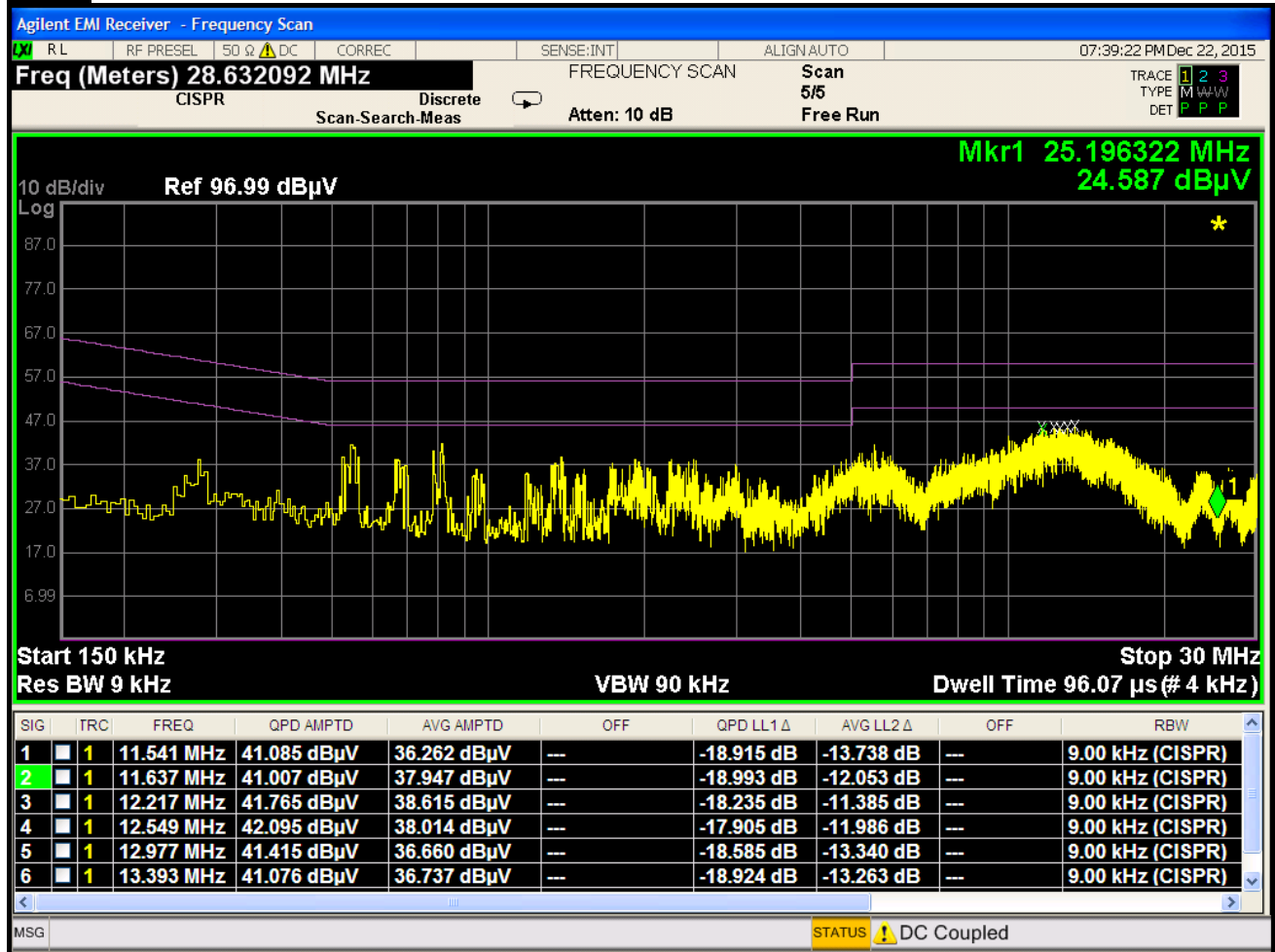
Plot 7-92. Line Conducted Plot with 802.11b (N)
