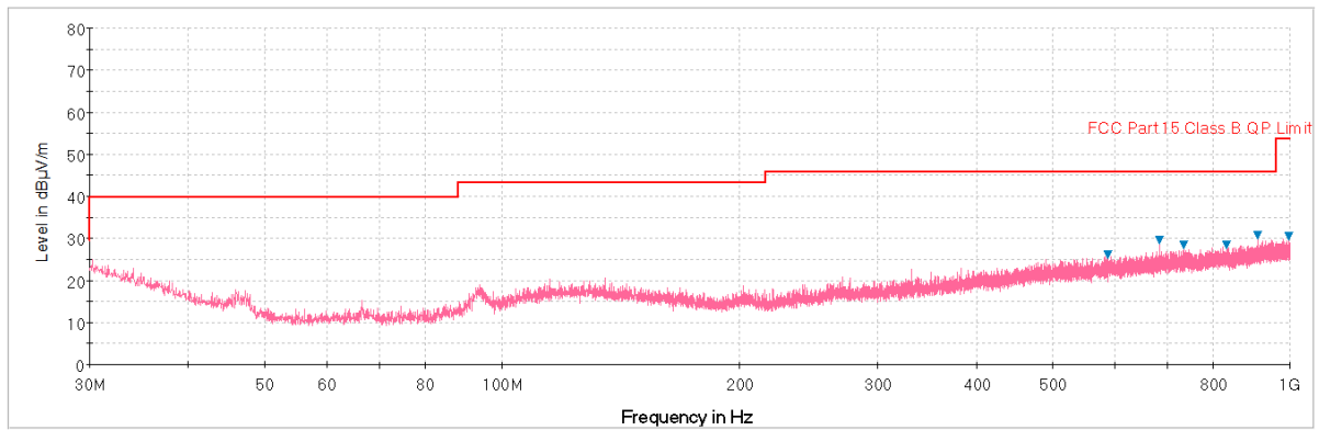
Plot 7-88. Radiated Spurious Plot below 1GHz (Pol. V)
