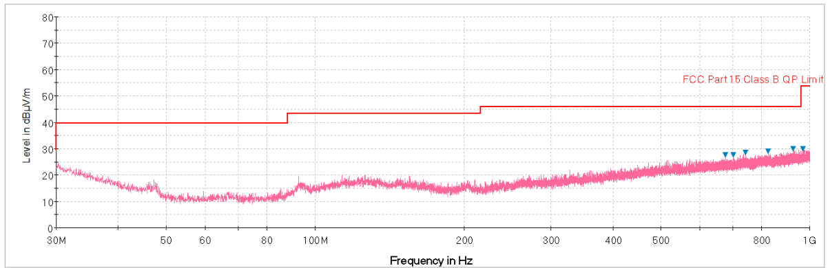
Plot 7-87. Radiated Spurious Plot below 1GHz (Pol. H)
