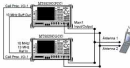
Figure 9-4 Power Measurement Setup
