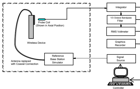
Figure 5-12 Audio Magnetic Field Test Setup
