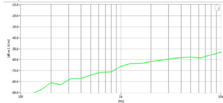
Noise Spectrum
