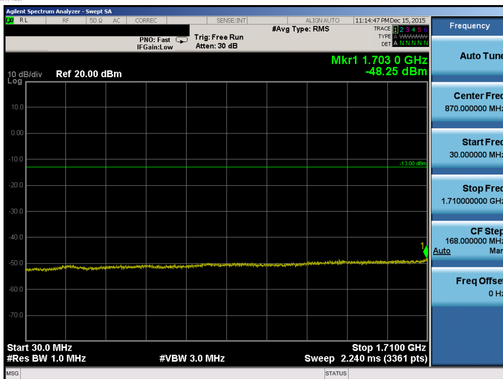
Plot 7-83. Conducted Spurious Plot (Band 4 – 15.0MHz QPSK – RB Size 1, RB Offset 0 – Mid Channel)
