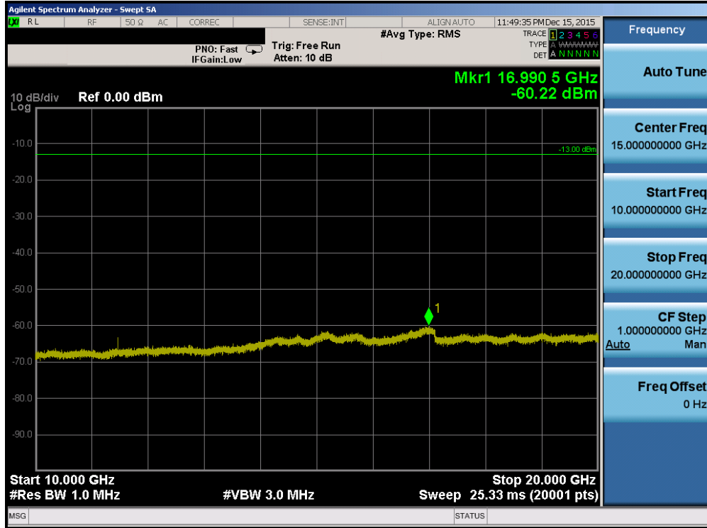
Plot 7-97. Conducted Spurious Plot (Band 2/25 – 5.0MHz QPSK – RB Size 1, RB Offset 0 – High Channel)
