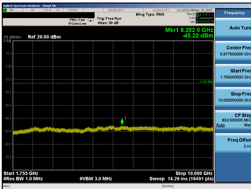
Plot 7-81. Conducted Spurious Plot (Band 4 – 15.0MHz QPSK – RB Size 1, RB Offset 0 – Low Channel)
