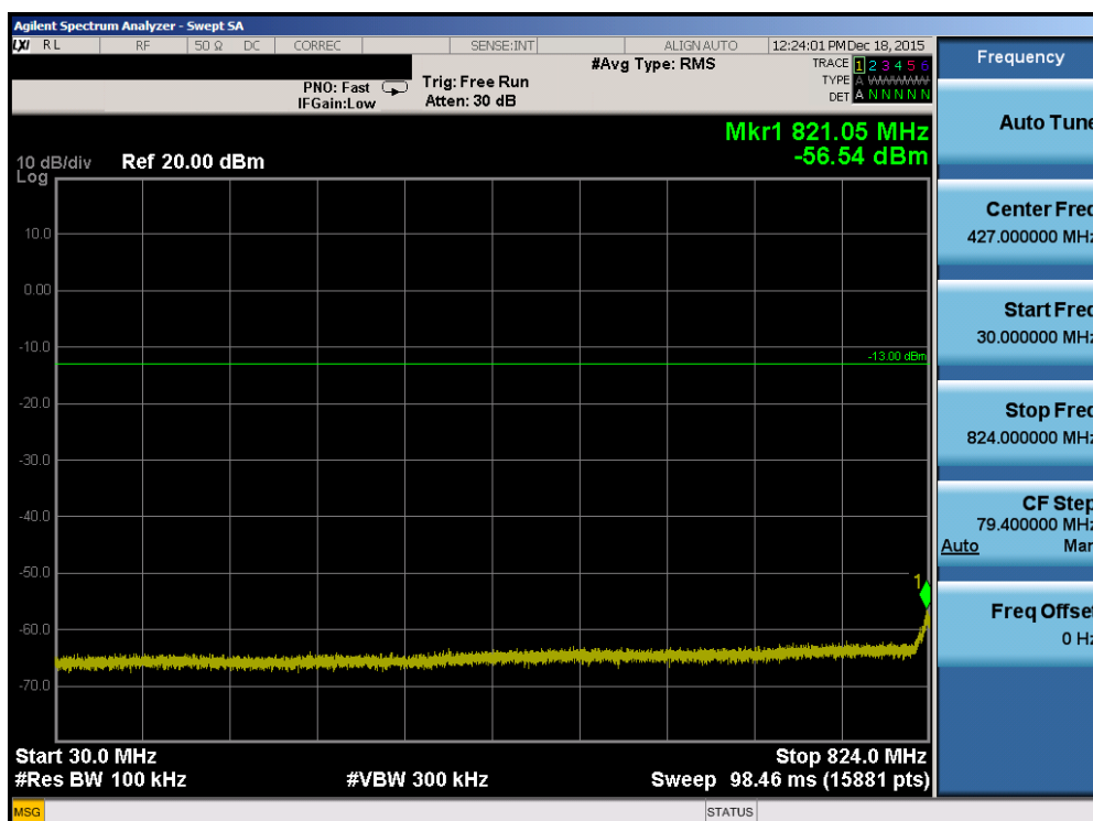
Plot 7-74. Conducted Spurious Plot (Band 5/26 – 5.0MHz QPSK – RB Size 1, RB Offset 0 – Mid Channel)
