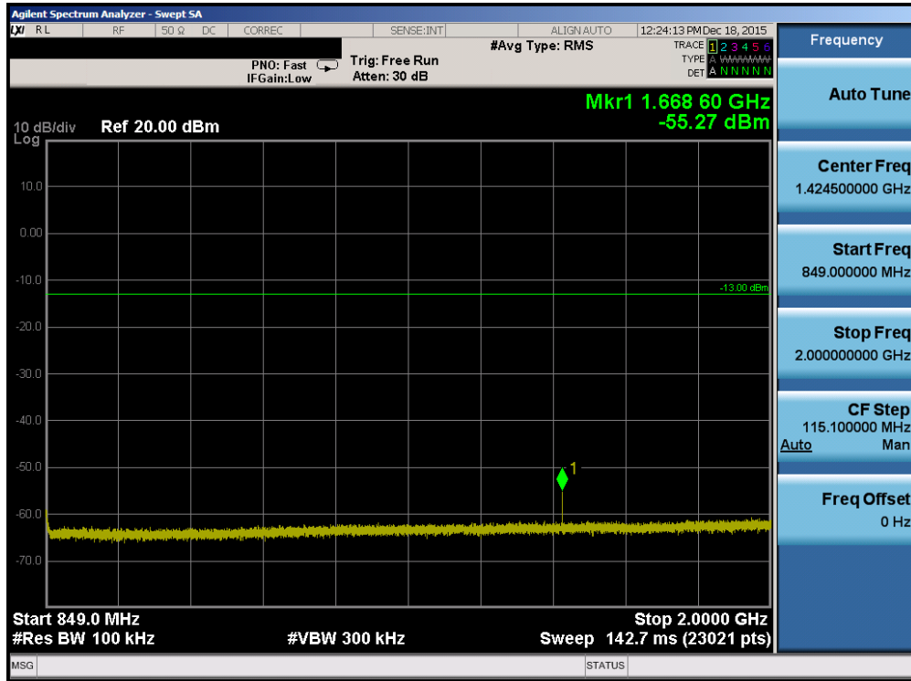
Plot 7-75. Conducted Spurious Plot (Band 5/26 – 5.0MHz QPSK – RB Size 1, RB Offset 0 – Mid Channel)
