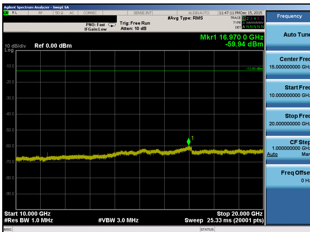
Plot 7-94. Conducted Spurious Plot (Band 2/25 – 5.0MHz QPSK – RB Size 1, RB Offset 0 – Mid Channel)
