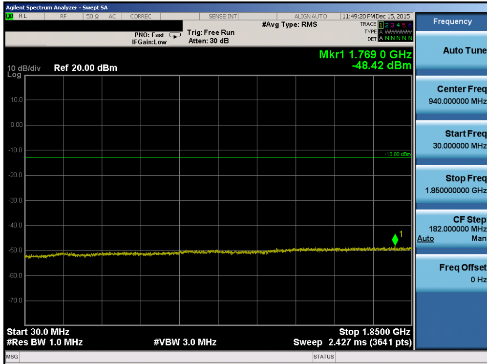
Plot 7-95. Conducted Spurious Plot (Band 2/25 – 5.0MHz QPSK – RB Size 1, RB Offset 0 – High Channel)
