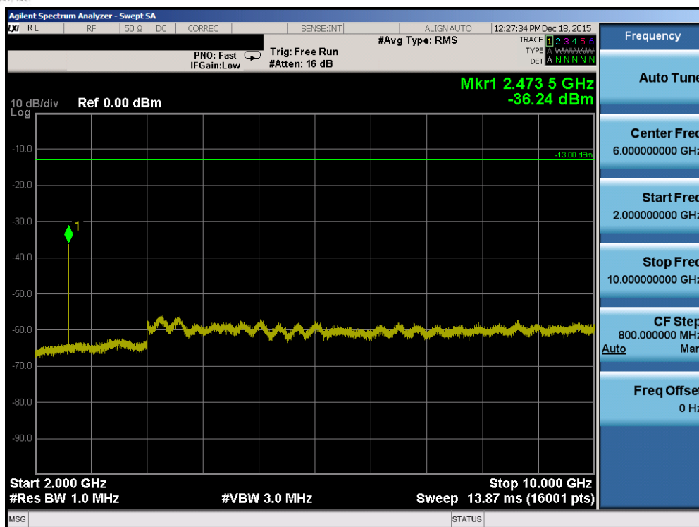
Plot 7-73. Conducted Spurious Plot (Band 5/26 – 5.0MHz QPSK – RB Size 1, RB Offset 0 – Low Channel)
