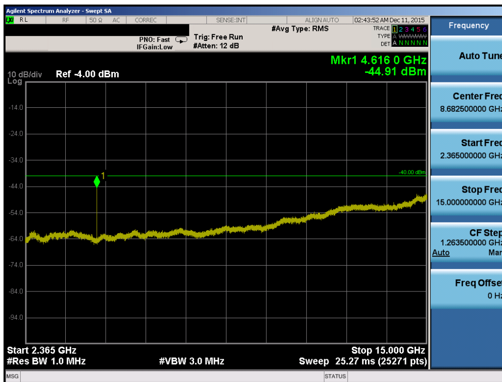
Plot 7-102. Conducted Spurious Plot (Band 30 – 5.0MHz QPSK – RB Size 1, RB Offset 0 – Mid Channel)
