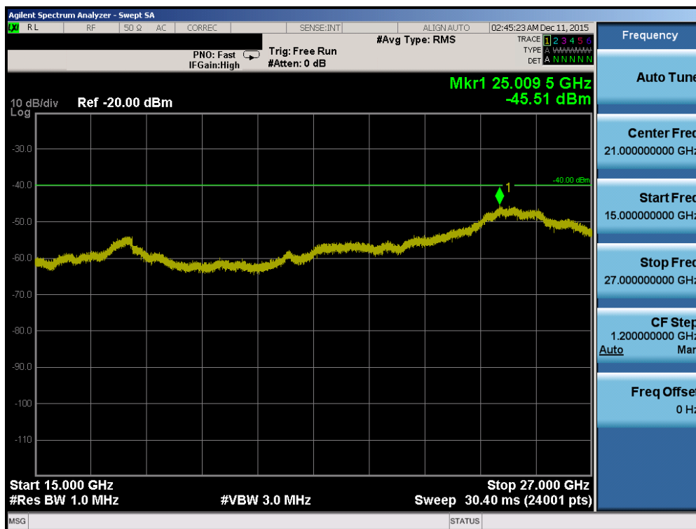
Plot 7-100. Conducted Spurious Plot (Band 30 – 5.0MHz QPSK – RB Size 1, RB Offset 0 – Low Channel)
