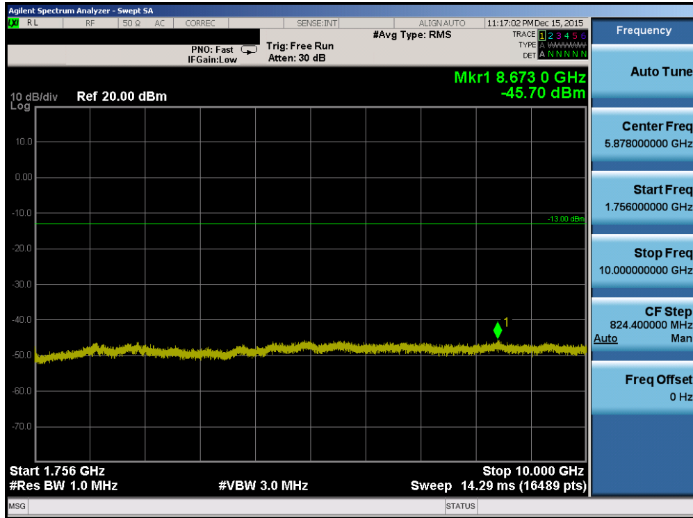
Plot 7-87. Conducted Spurious Plot (Band 4 – 15.0MHz QPSK – RB Size 1, RB Offset 0 – High Channel)
