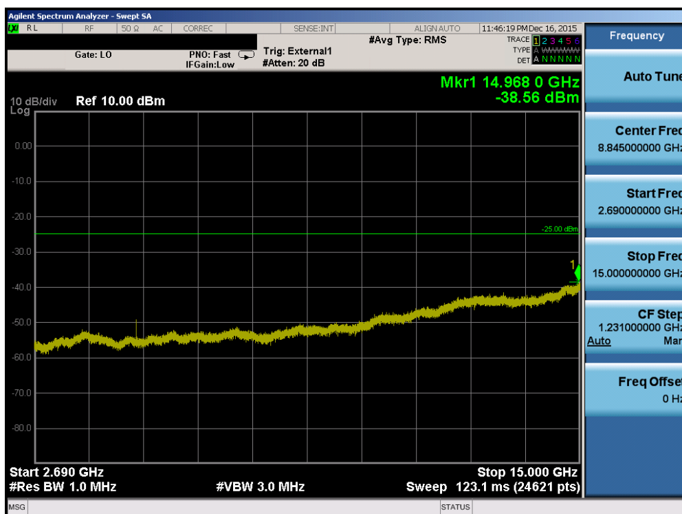
Plot 7-108. Conducted Spurious Plot (Band 41 – 5.0MHz QPSK – RB Size 1, RB Offset 0 – Low Channel)
