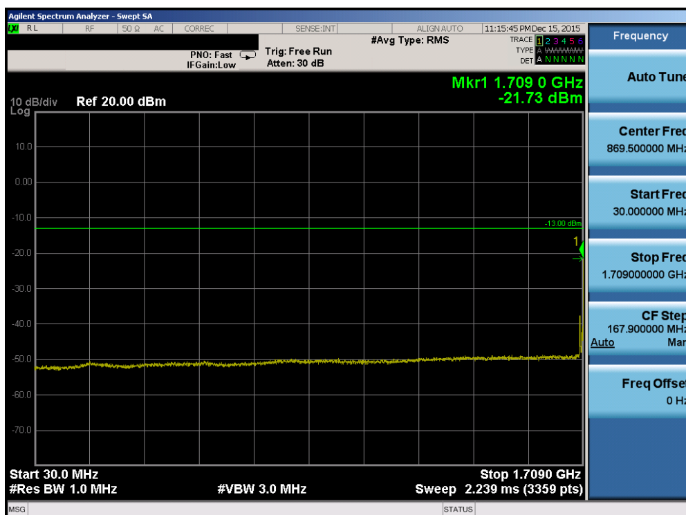
Plot 7-80. Conducted Spurious Plot (Band 4 – 15.0MHz QPSK – RB Size 1, RB Offset 0 – Low Channel)
