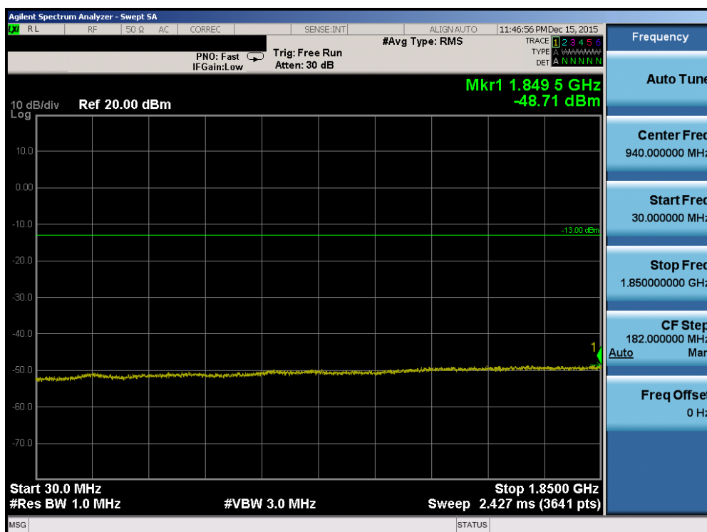
Plot 7-92. Conducted Spurious Plot (Band 2/25 – 5.0MHz QPSK – RB Size 1, RB Offset 0 – Mid Channel)
