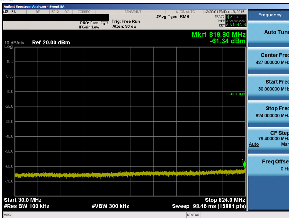
Plot 7-77. Conducted Spurious Plot (Band 5/26 – 5.0MHz QPSK – RB Size 1, RB Offset 0 – High Channel)
