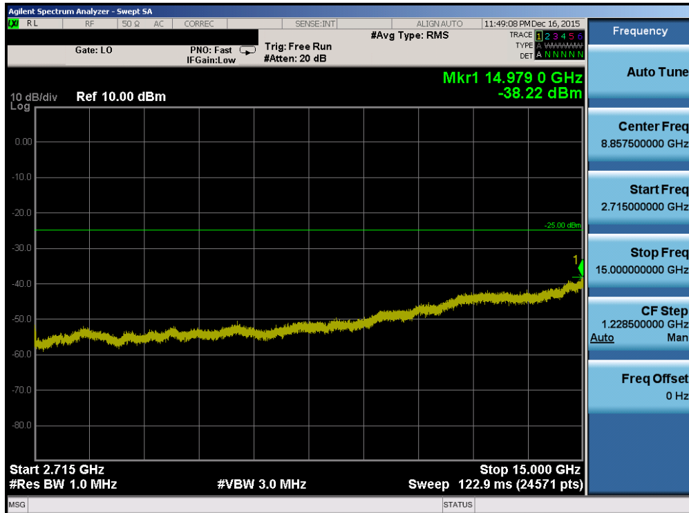
Plot 7-114. Conducted Spurious Plot (Band 41 – 5.0MHz QPSK – RB Size 1, RB Offset 0 – High Channel)
