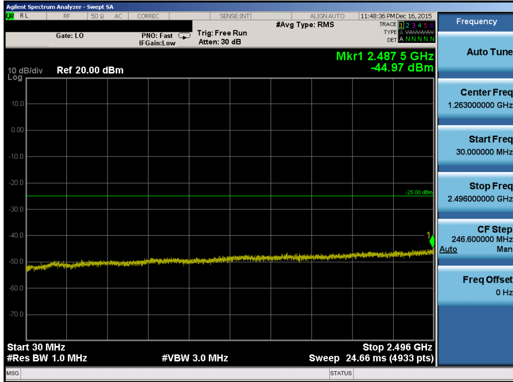
Plot 7-113. Conducted Spurious Plot (Band 41 – 5.0MHz QPSK – RB Size 1, RB Offset 0 – High Channel)
