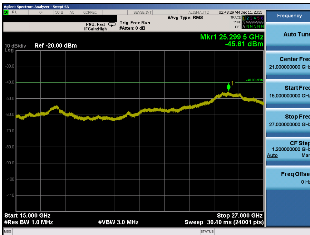
Plot 7-106. Conducted Spurious Plot (Band 30 – 5.0MHz QPSK – RB Size 1, RB Offset 0 – High Channel)
