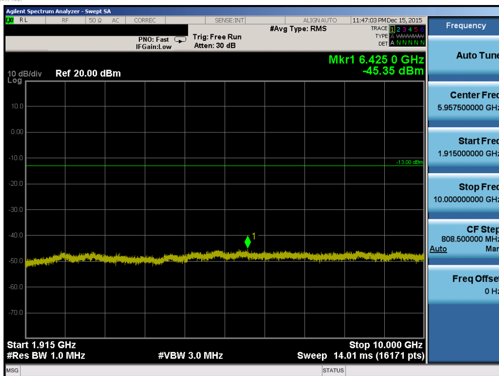
Plot 7-93. Conducted Spurious Plot (Band 2/25 – 5.0MHz QPSK – RB Size 1, RB Offset 0 – Mid Channel)
