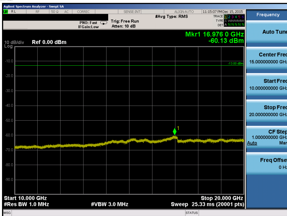
Plot 7-85. Conducted Spurious Plot (Band 4 – 15.0MHz QPSK – RB Size 1, RB Offset 0 – Mid Channel)
