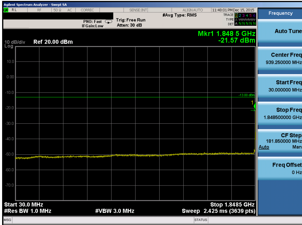
Plot 7-89. Conducted Spurious Plot (Band 2/25 – 5.0MHz QPSK – RB Size 1, RB Offset 0 – Low Channel)
