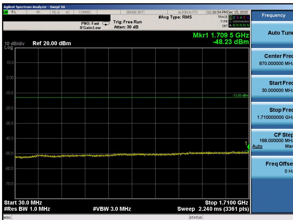
Plot 7-86. Conducted Spurious Plot (Band 4 – 15.0MHz QPSK – RB Size 1, RB Offset 0 – High Channel)
