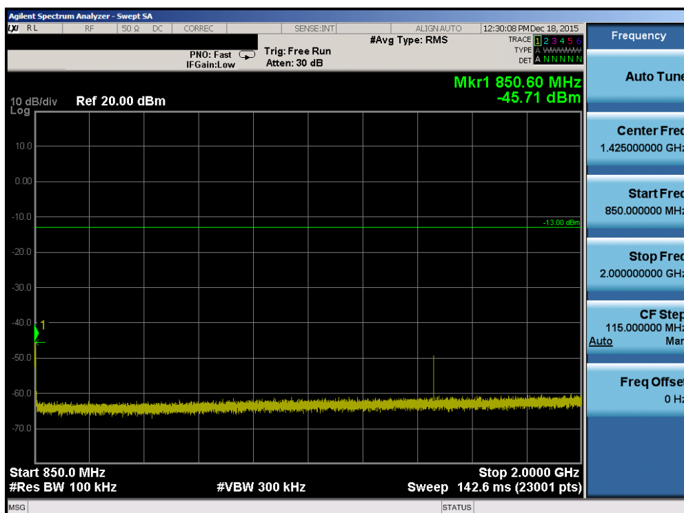
Plot 7-78. Conducted Spurious Plot (Band 5/26 – 5.0MHz QPSK – RB Size 1, RB Offset 0 – High Channel)
