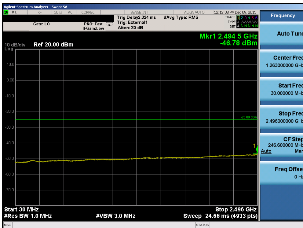
Plot 7-110. Conducted Spurious Plot (Band 41 – 5.0MHz QPSK – RB Size 1, RB Offset 0 – Mid Channel)
