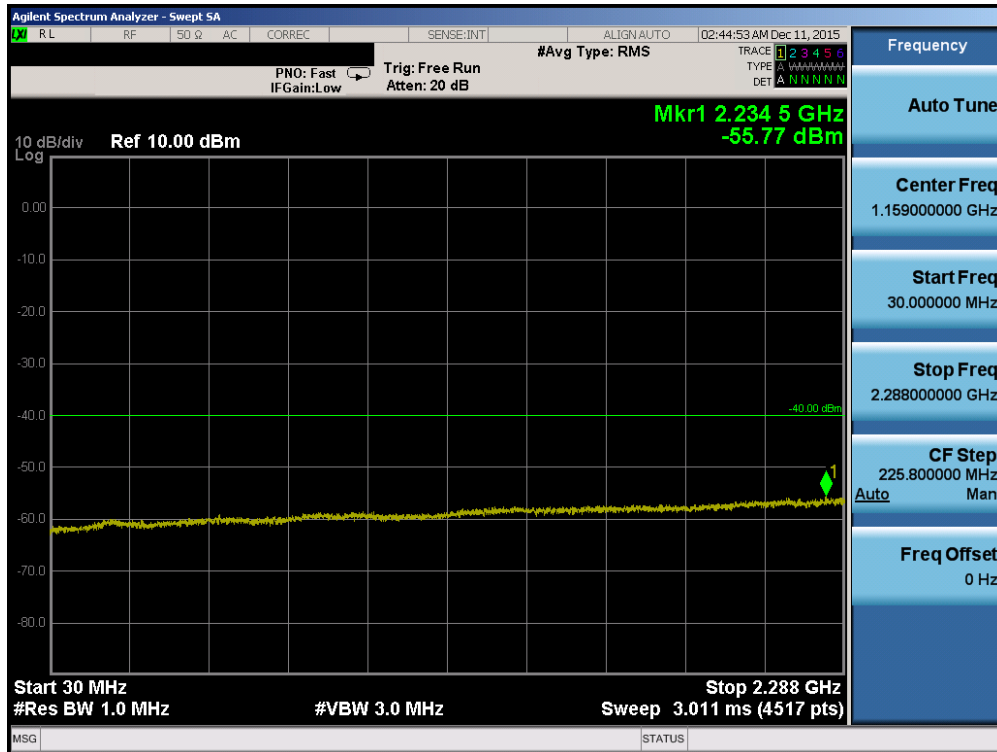
Plot 7-98. Conducted Spurious Plot (Band 30 – 5.0MHz QPSK – RB Size 1, RB Offset 0 – Low Channel)
