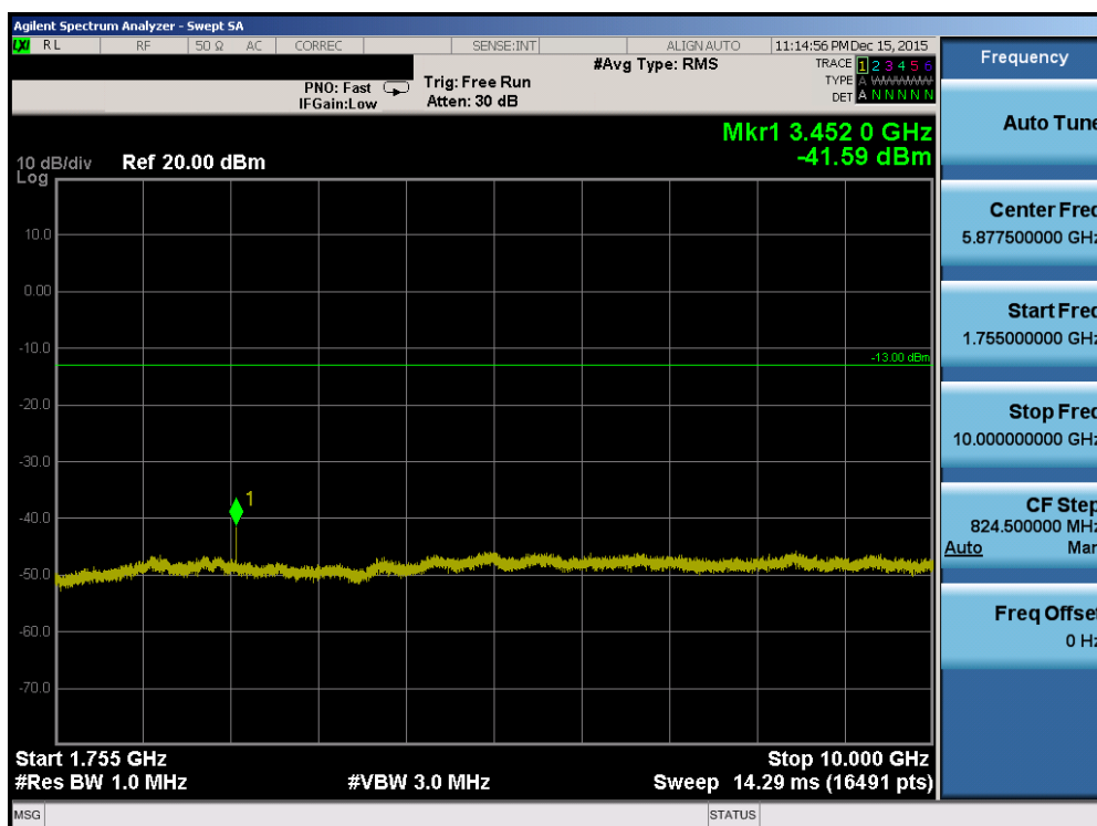
Plot 7-84. Conducted Spurious Plot (Band 4 – 15.0MHz QPSK – RB Size 1, RB Offset 0 – Mid Channel)
