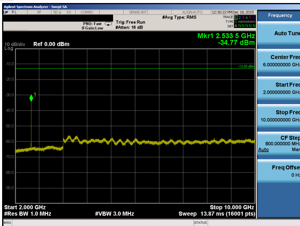
Plot 7-79. Conducted Spurious Plot (Band 5/26 – 5.0MHz QPSK – RB Size 1, RB Offset 0 – High Channel)
