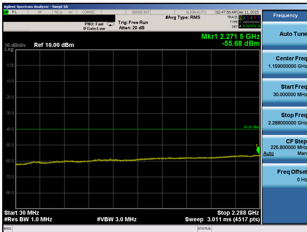
Plot 7-104. Conducted Spurious Plot (Band 30 – 5.0MHz QPSK – RB Size 1, RB Offset 0 – High Channel)
