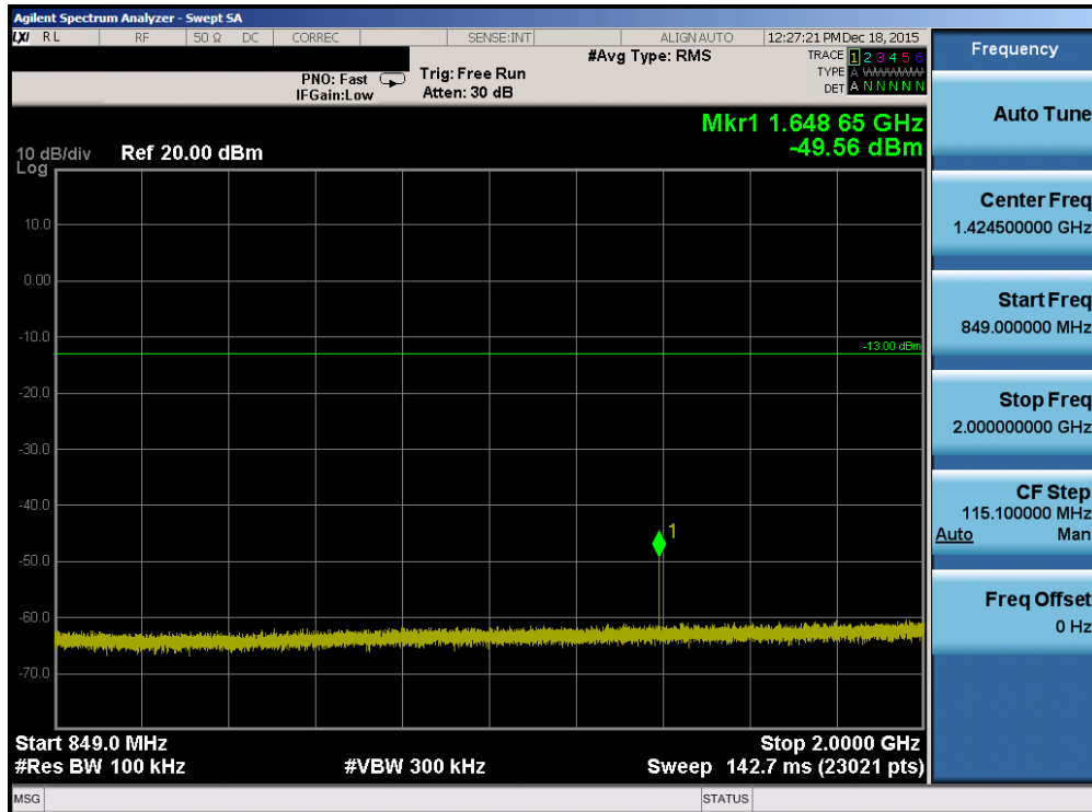
Plot 7-72. Conducted Spurious Plot (Band 5/26 – 5.0MHz QPSK – RB Size 1, RB Offset 0 – Low Channel)
