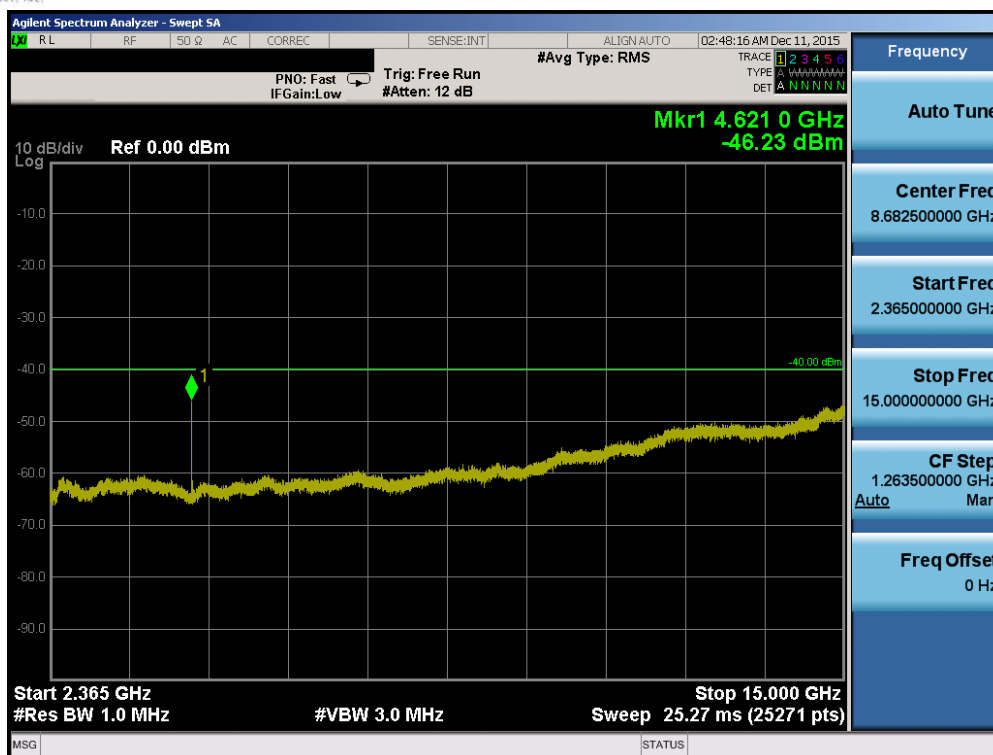
Plot 7-105. Conducted Spurious Plot (Band 30 – 5.0MHz QPSK – RB Size 1, RB Offset 0 – High Channel)
