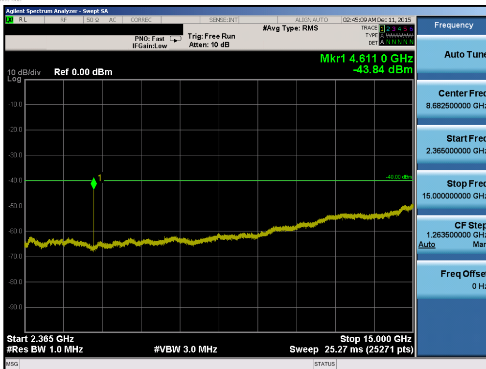
Plot 7-99. Conducted Spurious Plot (Band 30 – 5.0MHz QPSK – RB Size 1, RB Offset 0 – Low Channel)
