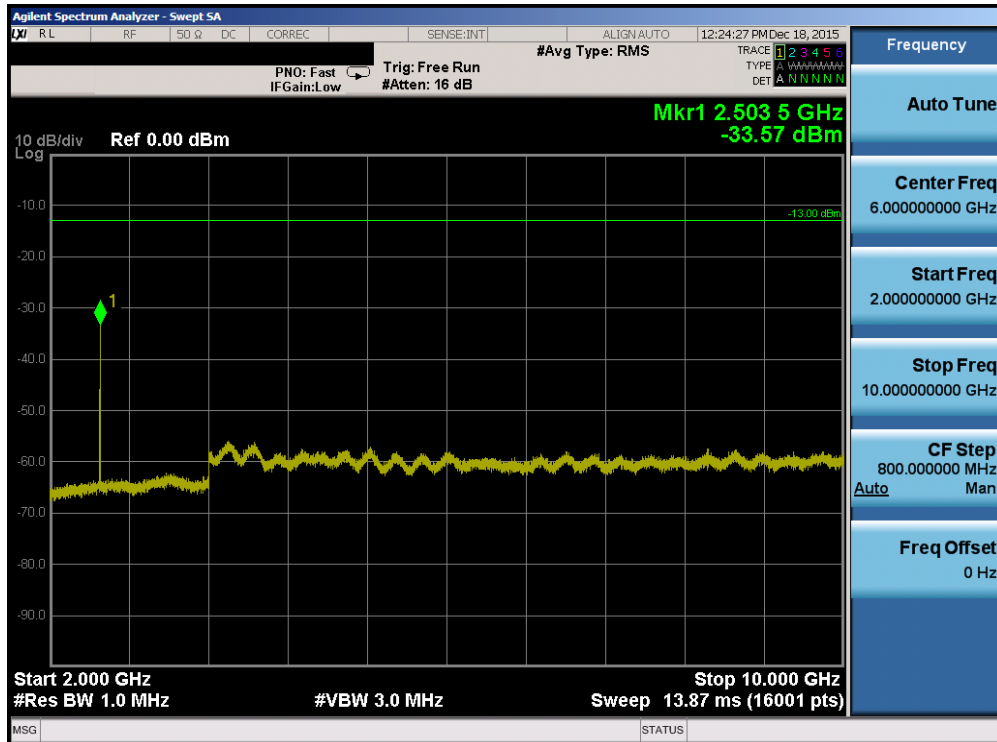
Plot 7-76. Conducted Spurious Plot (Band 5/26 – 5.0MHz QPSK – RB Size 1, RB Offset 0 – Mid Channel)
