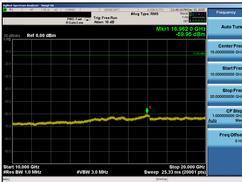
Plot 7-91. Conducted Spurious Plot (Band 2/25 – 5.0MHz QPSK – RB Size 1, RB Offset 0 – Low Channel)
