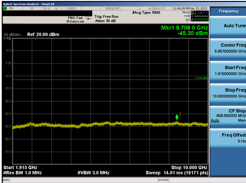
Plot 7-90. Conducted Spurious Plot (Band 2/25 – 5.0MHz QPSK – RB Size 1, RB Offset 0 – Low Channel)
