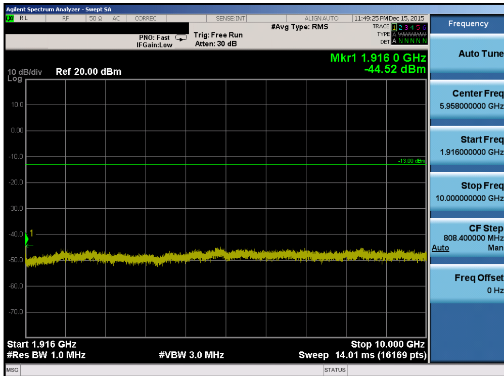
Plot 7-96. Conducted Spurious Plot (Band 2/25 – 5.0MHz QPSK – RB Size 1, RB Offset 0 – High Channel)
