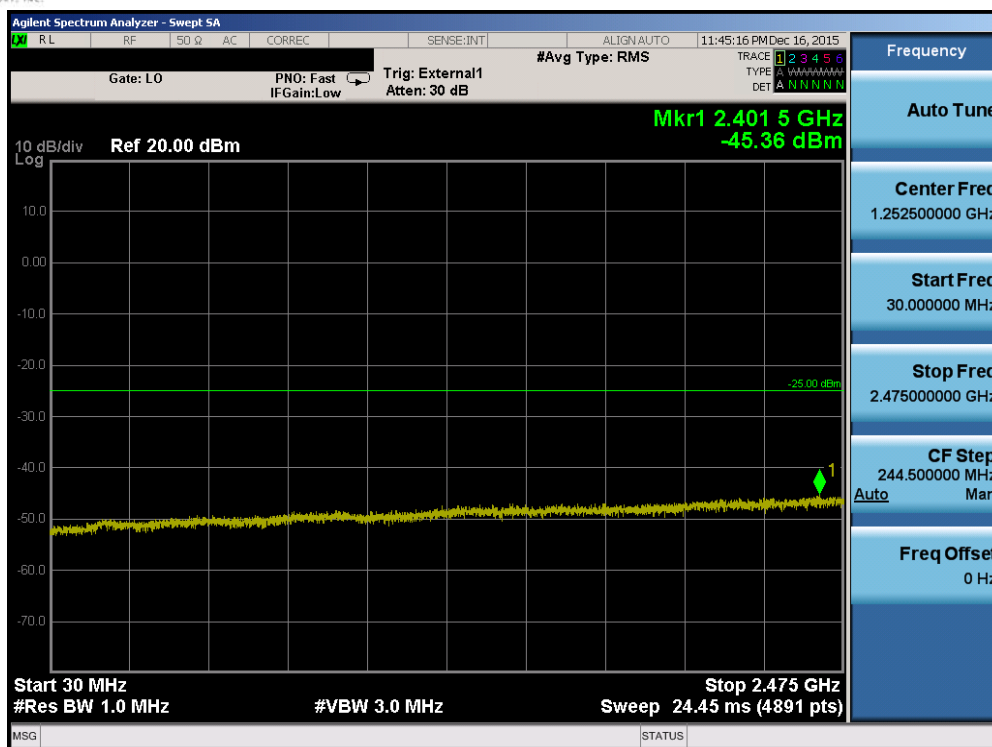
Plot 7-107. Conducted Spurious Plot (Band 41 – 5.0MHz QPSK – RB Size 1, RB Offset 0 – Low Channel)
