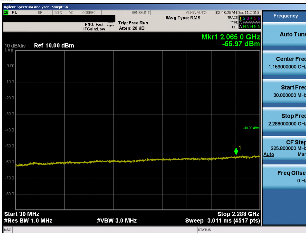
Plot 7-101. Conducted Spurious Plot (Band 30 – 5.0MHz QPSK – RB Size 1, RB Offset 0 – Mid Channel)
