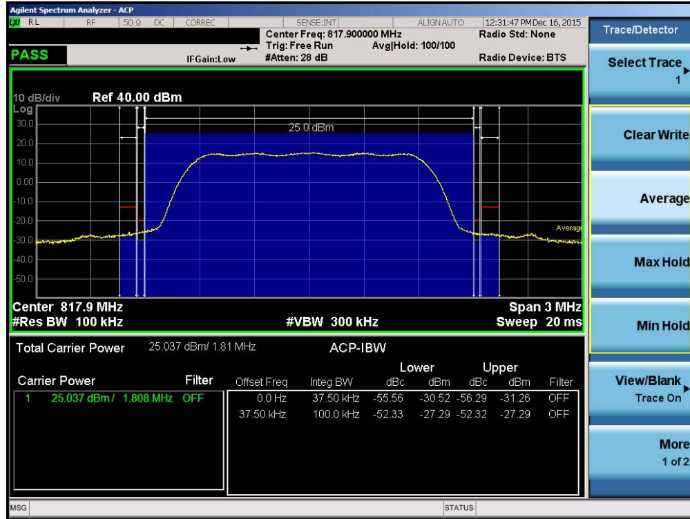
Plot 7-19. Channel Edge Plot (Ch. 476)
