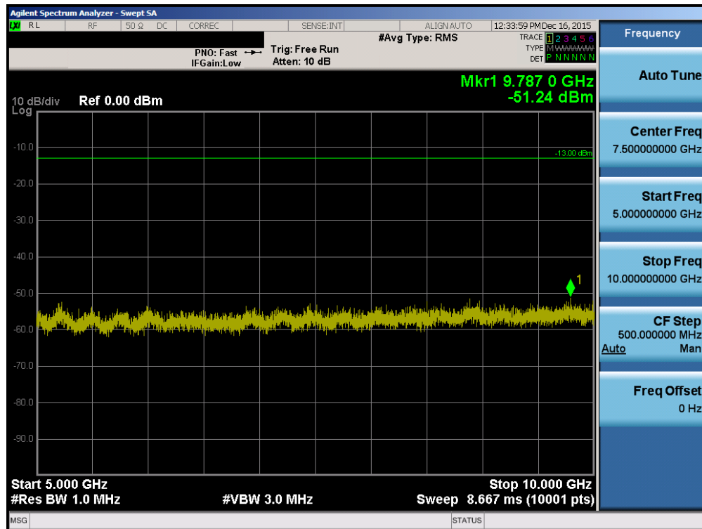
Plot 7-14. Conducted Spurious Plot (Ch. 684)
