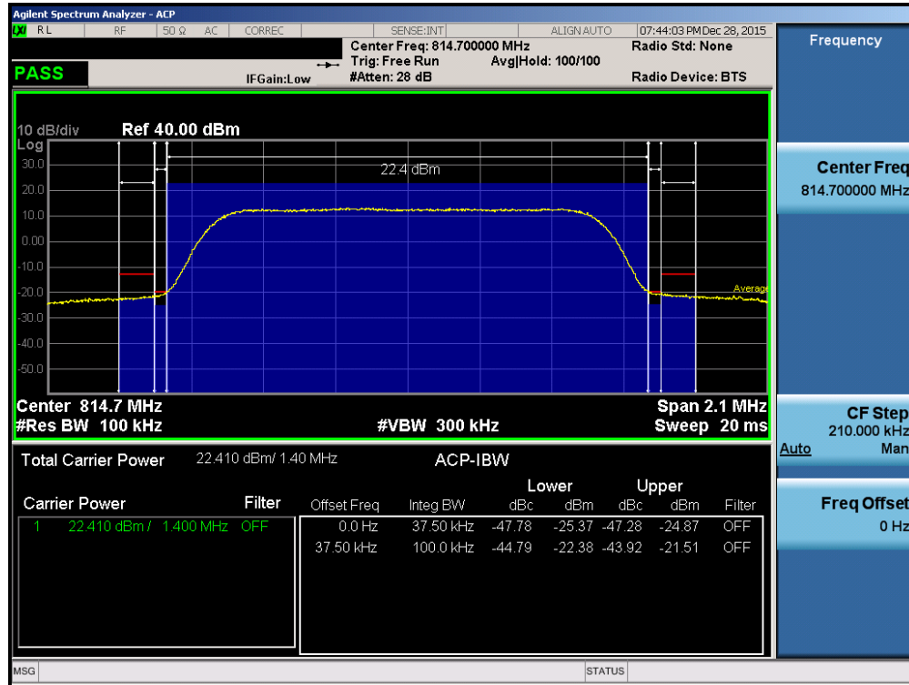
Plot 7-21. Channel Edge Plot (1.4MHz QPSK – RB Size 6– Low Channel)
