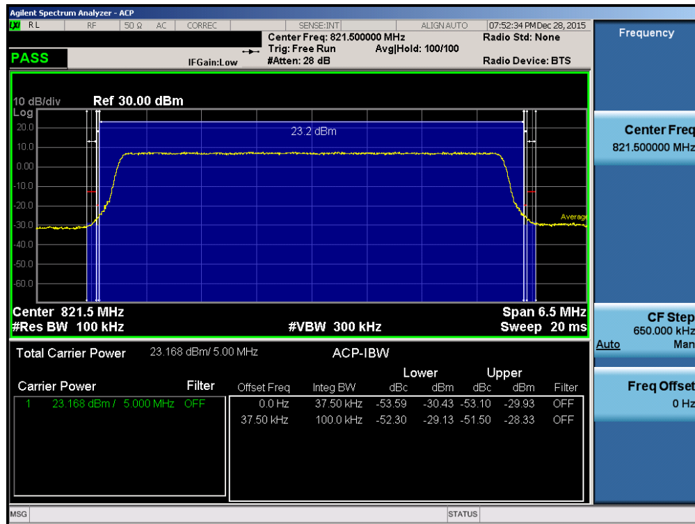
Plot 7-26. Channel Edge Plot (5MHz QPSK – RB Size 25 – High Channel)
