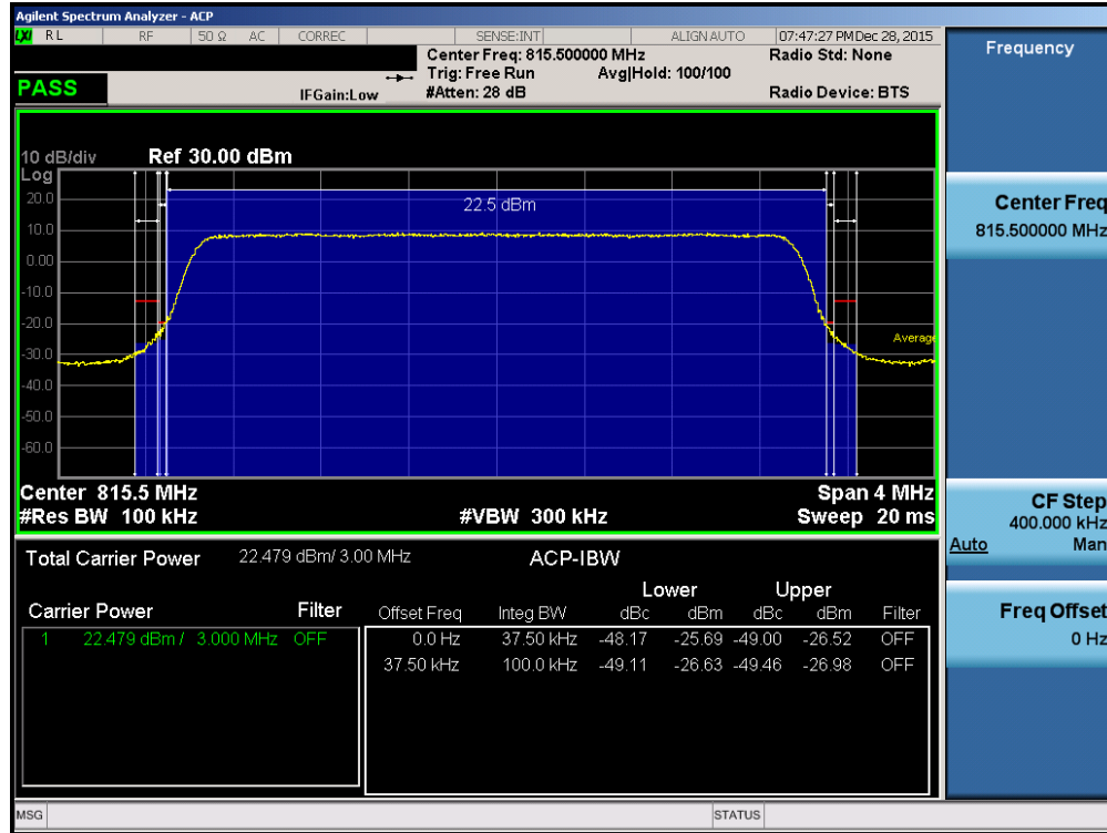
Plot 7-23. Channel Edge Plot (3MHz QPSK – RB Size 15– Low Channel)
