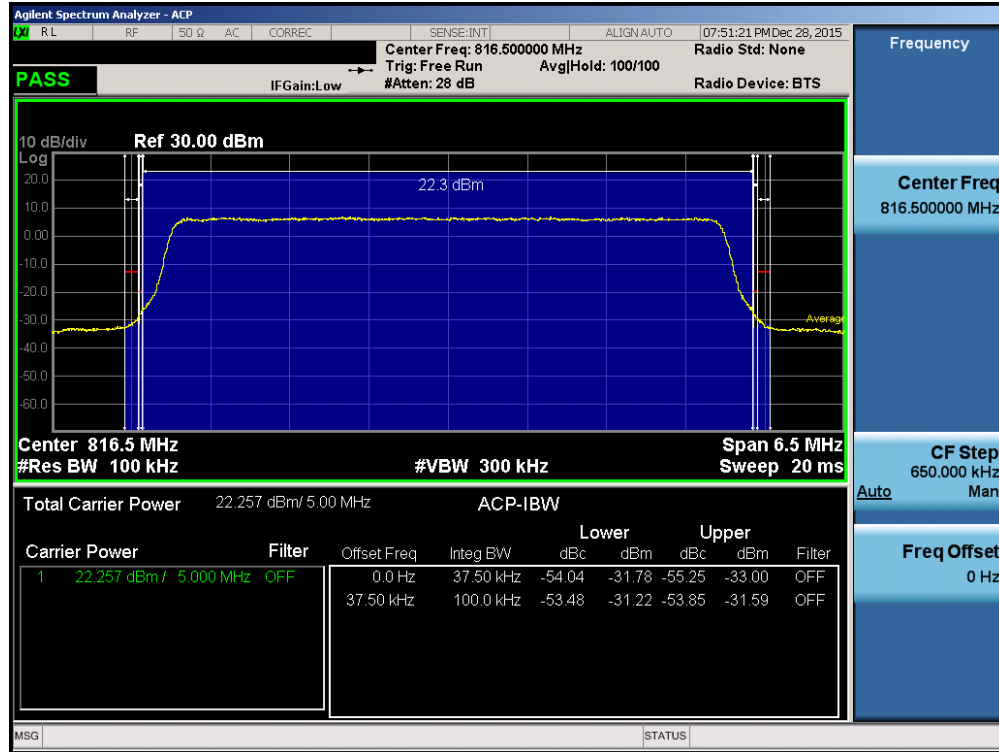
Plot 7-25. Channel Edge Plot (5MHz QPSK – RB Size 25– Low Channel)
