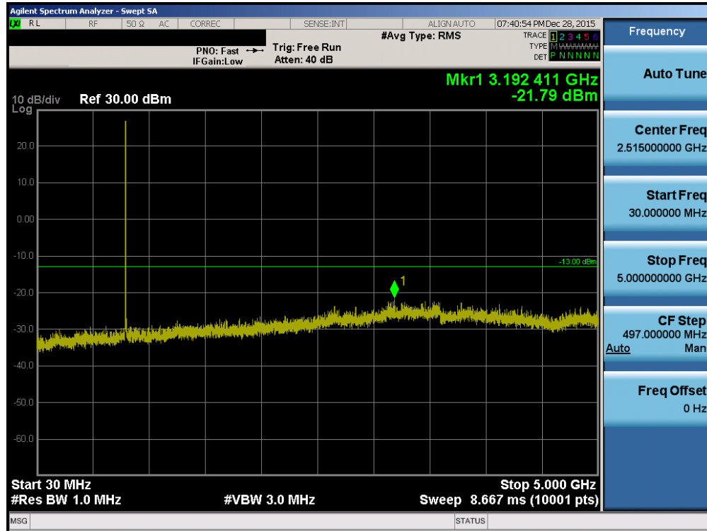
Plot 7-15. Conducted Spurious Plot (3MHz QPSK – RB Size 1, RB Offset 0 – Low Channel)
