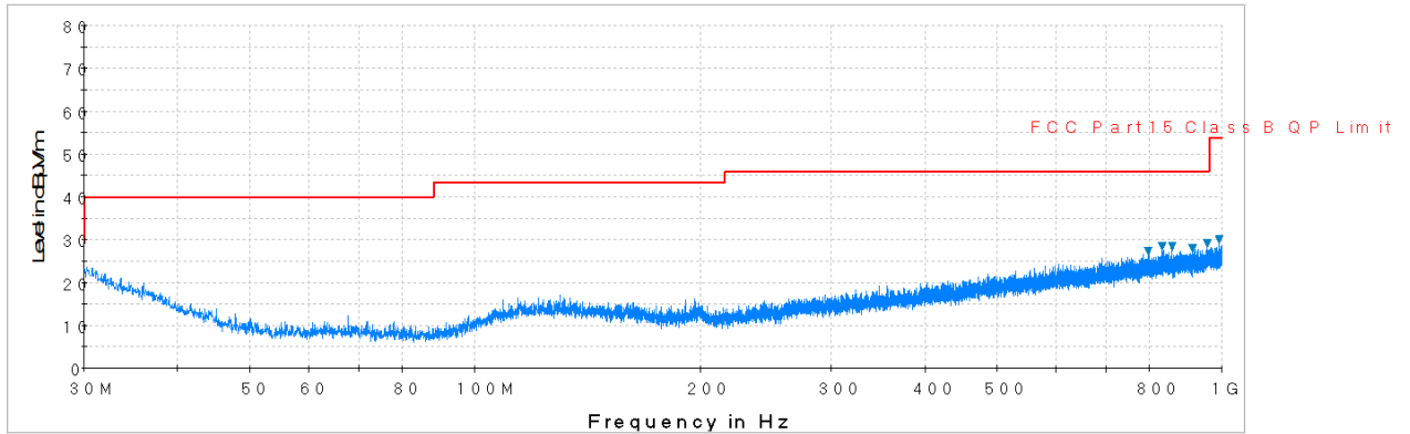
Plot 7-54. Radiated Spurious Plot below 1GHz (Pol. H)
