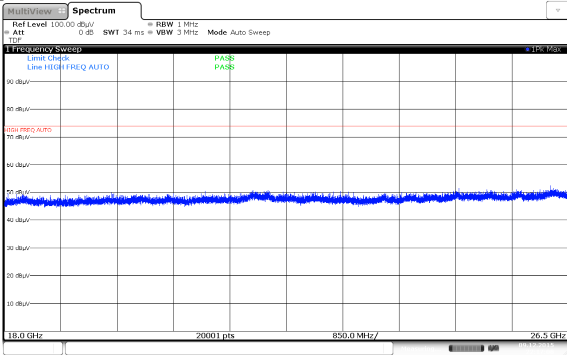
Plot 7-177. Radiated Spurious Plot 18GHz – 26.5GHz (802.11a – Ant. Pol. H)
