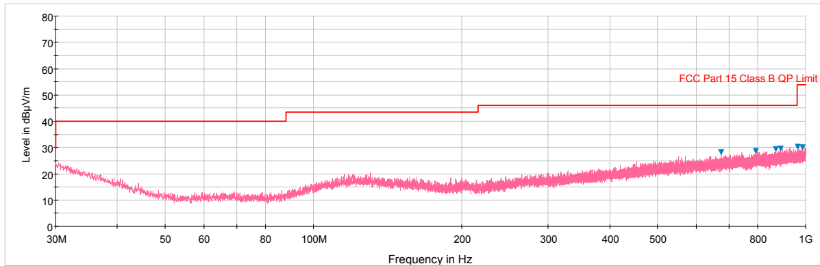
Plot 7-279. Radiated Spurious Plot below 1GHz (Simultaneous Transmission Config-1, Ant. Pol. V)
