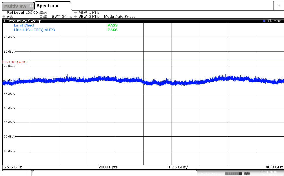
Plot 7-186. Radiated Spurious Plot above 26.5GHz (Simultaneous Transmission Config-1 Ant. Pol. H)
