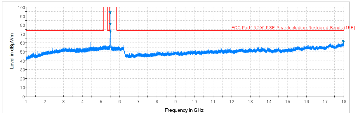
Plot 7-173. Radiated Spurious Plot above 1GHz (802.11a – U2C Ch. 116, Ant. Pol. H)
