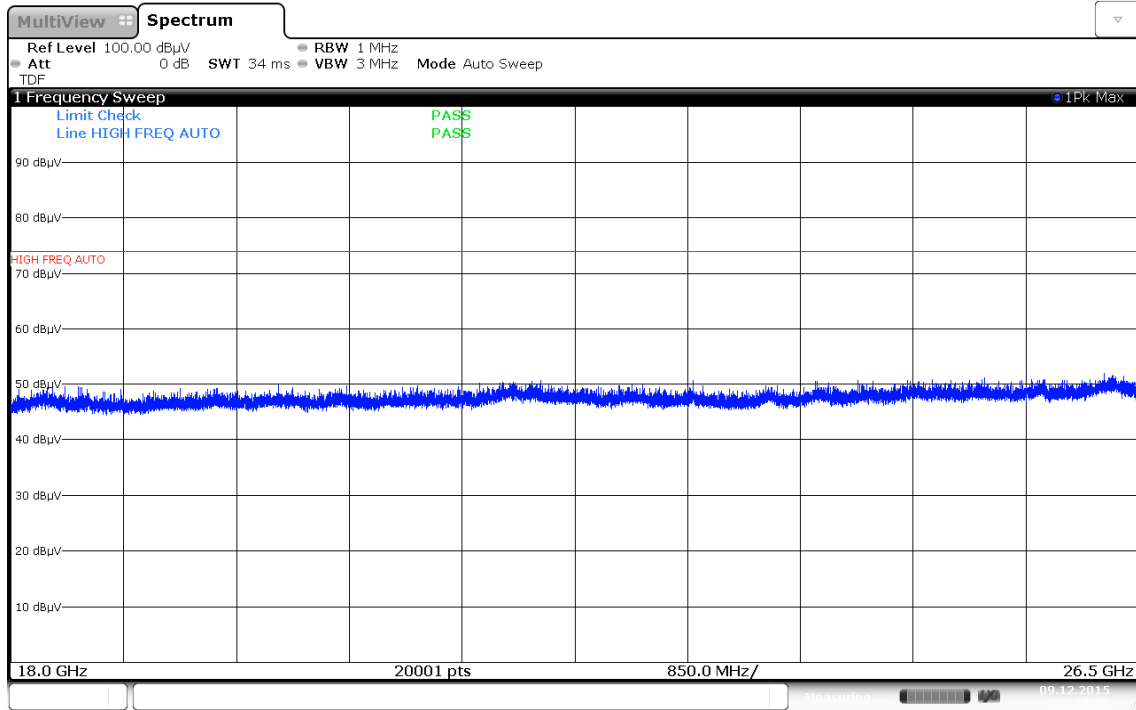
Plot 7-179. Radiated Spurious Plot 18GHz – 26.5GHz (802.11a – Ant. Pol. V)
