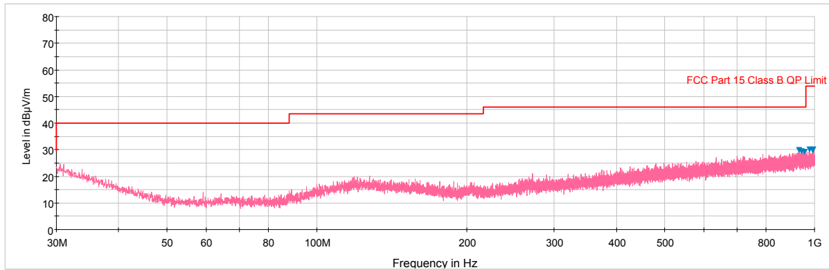
Plot 7-278. Radiated Spurious Plot below 1GHz (Simultaneous Transmission Config-1, Ant. Pol. H)
