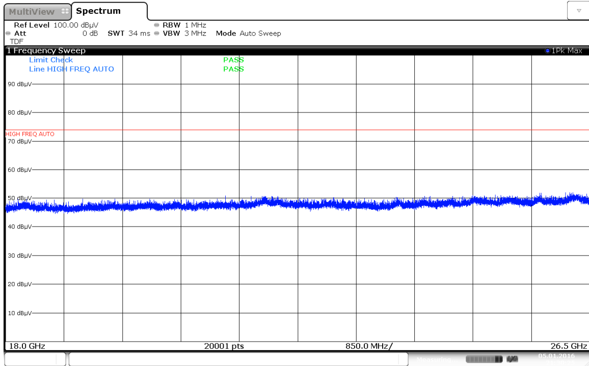
Plot 7-189. Radiated Spurious Plot 18GHz – 26.5GHz (Simultaneous Transmission Config-2 Ant. Pol. H)
