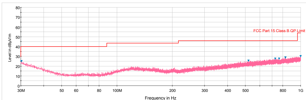
Plot 7-280. Radiated Spurious Plot below 1GHz (Simultaneous Transmission Config-2, Ant. Pol. H)
