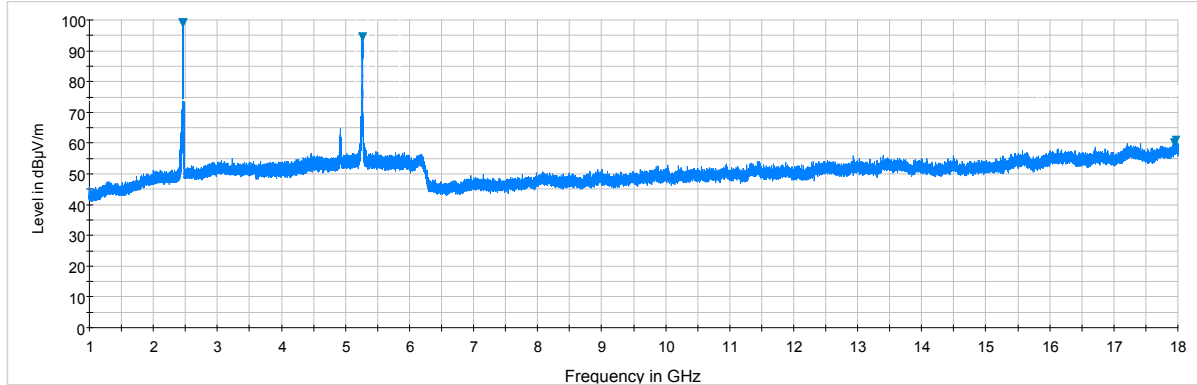
Plot 7-187. Radiated Spurious Plot above 1GHz (Simultaneous Transmission Config-2, Ant. Pol. H)
