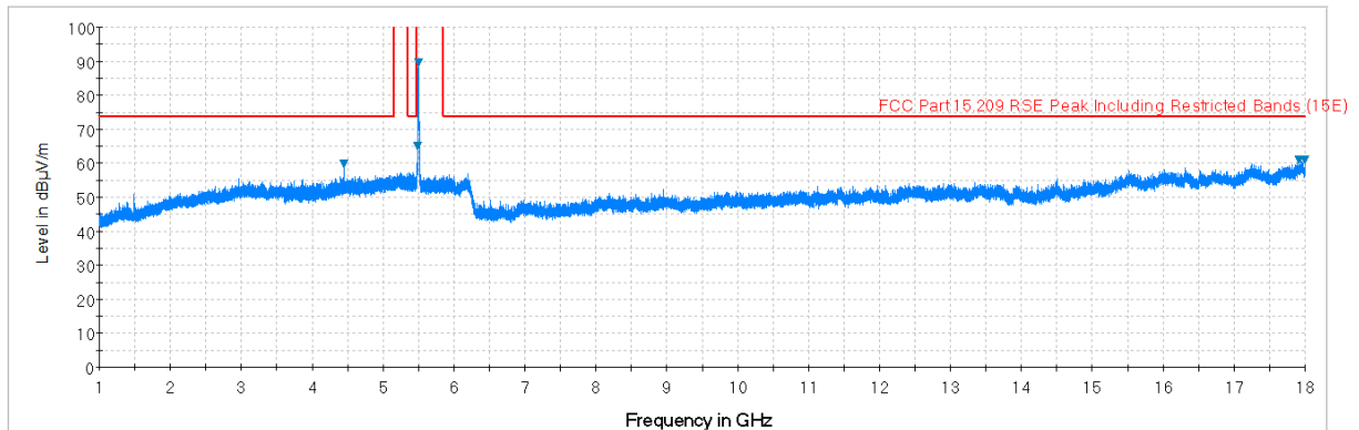
Plot 7-174. Radiated Spurious Plot above 1GHz (802.11a – U2C Ch. 116, Ant. Pol. V)
