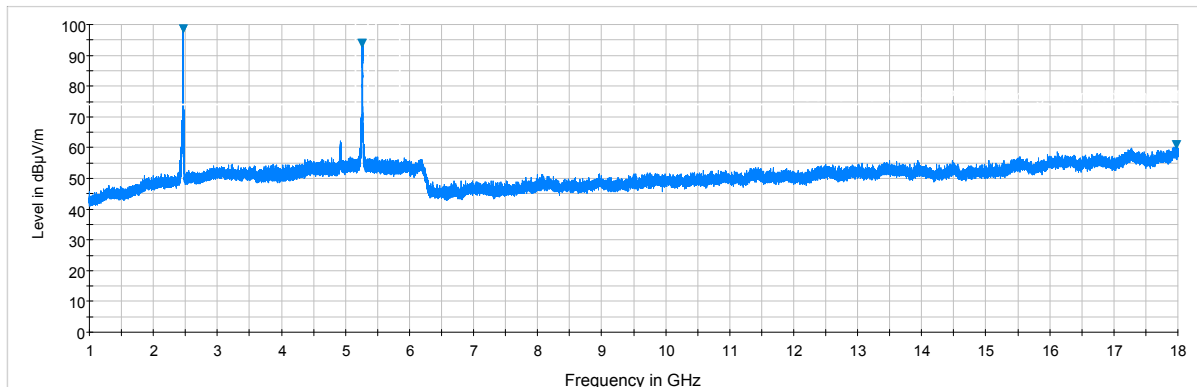
Plot 7-188. Radiated Spurious Plot above 1GHz (Simultaneous Transmission Config-2, Ant. Pol. V)
