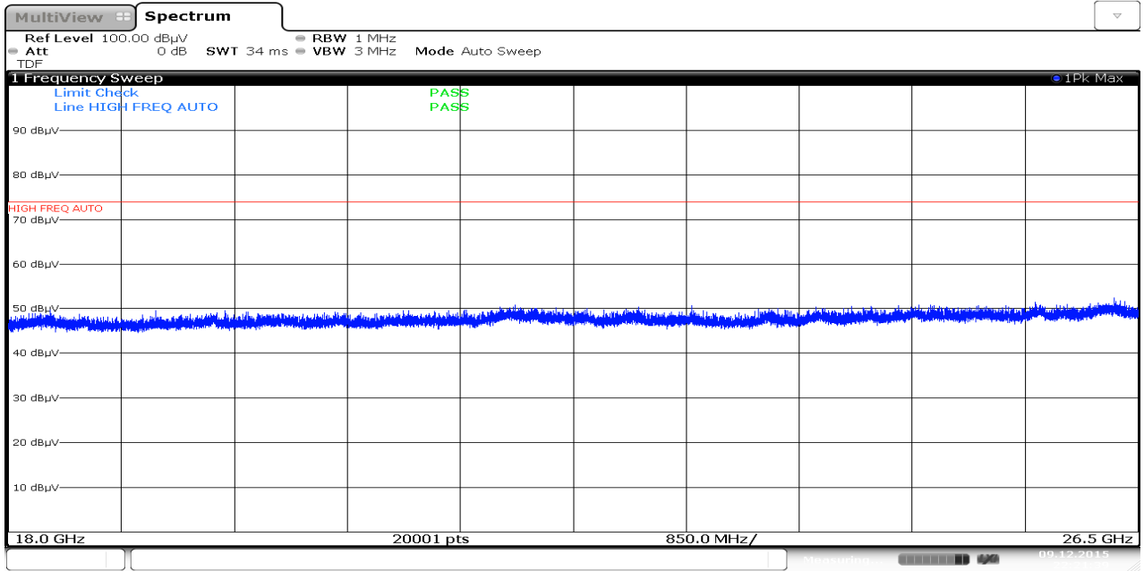
Plot 7-167. Radiated Spurious Plot 18GHz – 26.5GHz (802.11a – Ant. Pol. V)
