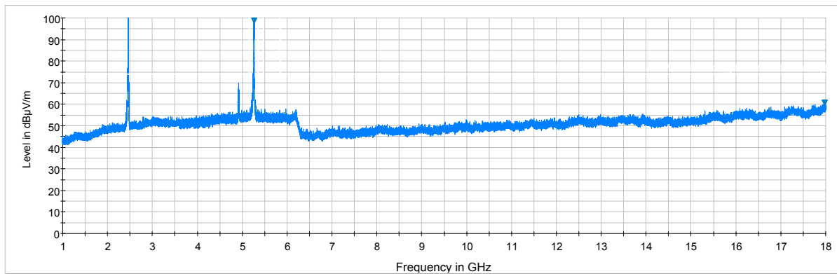
Plot 7-181. Radiated Spurious Plot above 1GHz (Simultaneous Transmission Config-1, Ant. Pol. H)
