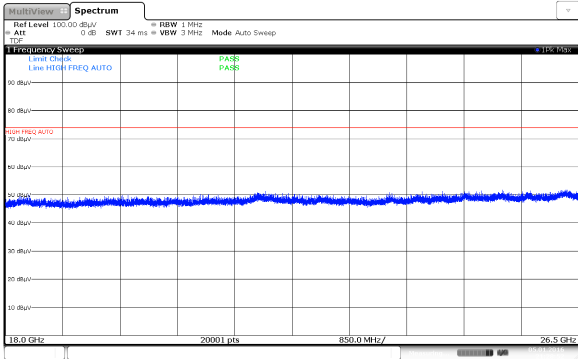
Plot 7-185. Radiated Spurious Plot 18GHz – 26.5GHz (Simultaneous Transmission Config-1 Ant. Pol. V)
