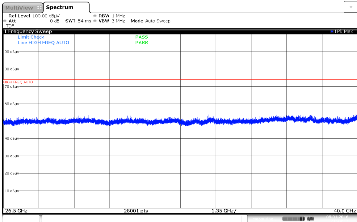
Plot 7-192. Radiated Spurious Plot above 26.5GHz (Simultaneous Transmission Config-2 Ant. Pol. H)
