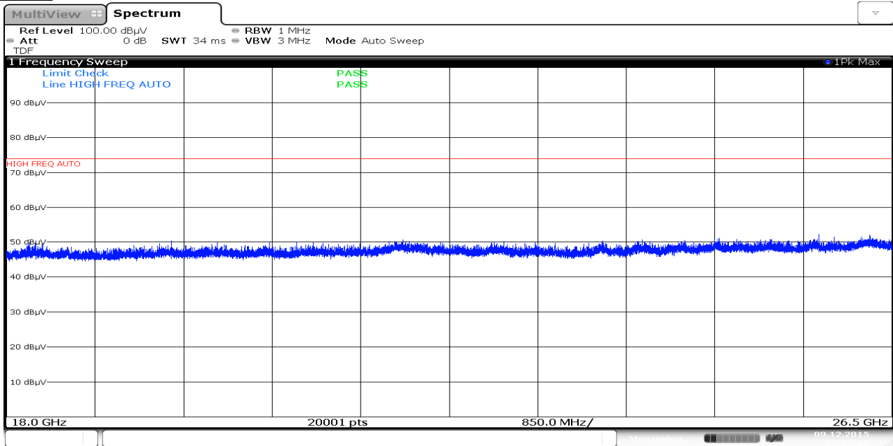
Plot 7-165. Radiated Spurious Plot 18GHz – 26.5GHz (802.11a – Ant. Pol. H)
