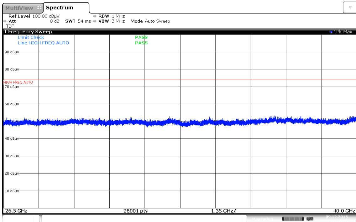
Plot 7-180. Radiated Spurious Plot above 26.5GHz (802.11a – Ant. Pol. H)
