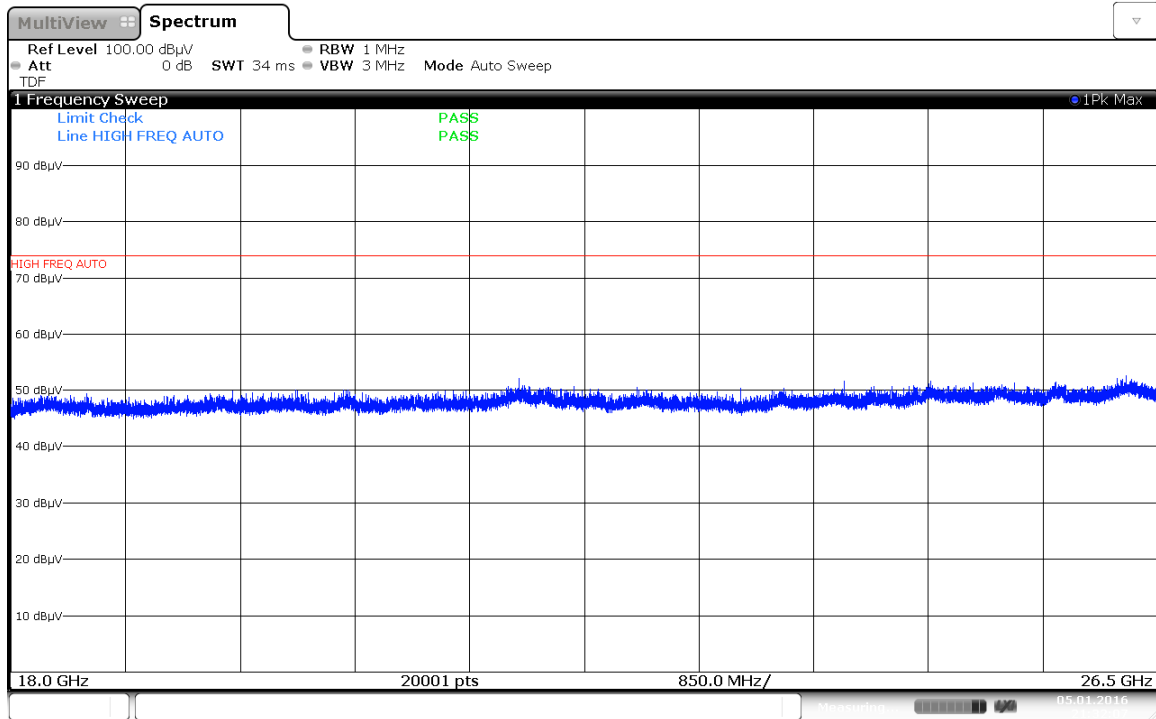
Plot 7-191. Radiated Spurious Plot 18GHz – 26.5GHz (Simultaneous Transmission Config-2 Ant. Pol. V)
