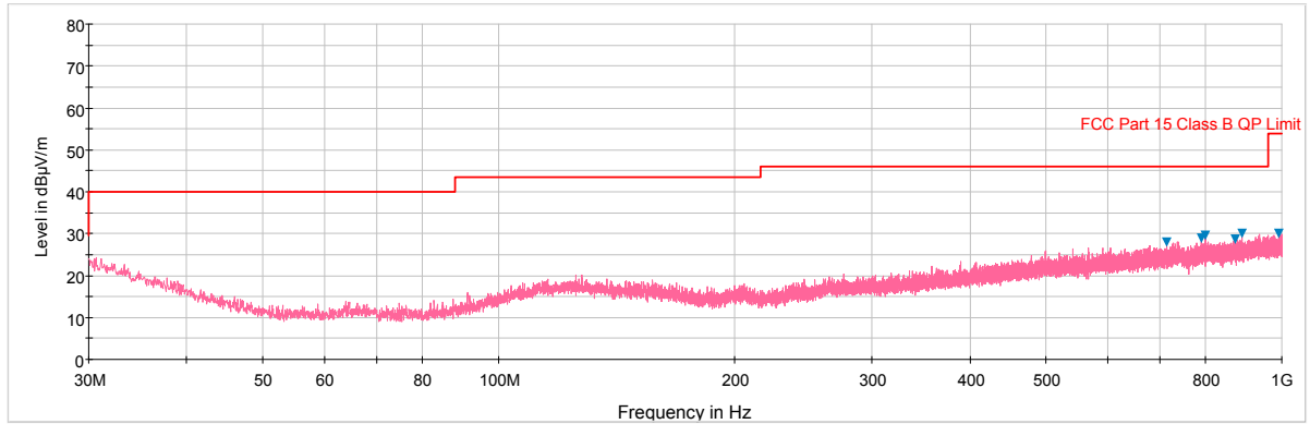
Plot 7-281. Radiated Spurious Plot below 1GHz (Simultaneous Transmission Config-2, Ant. Pol. V)
