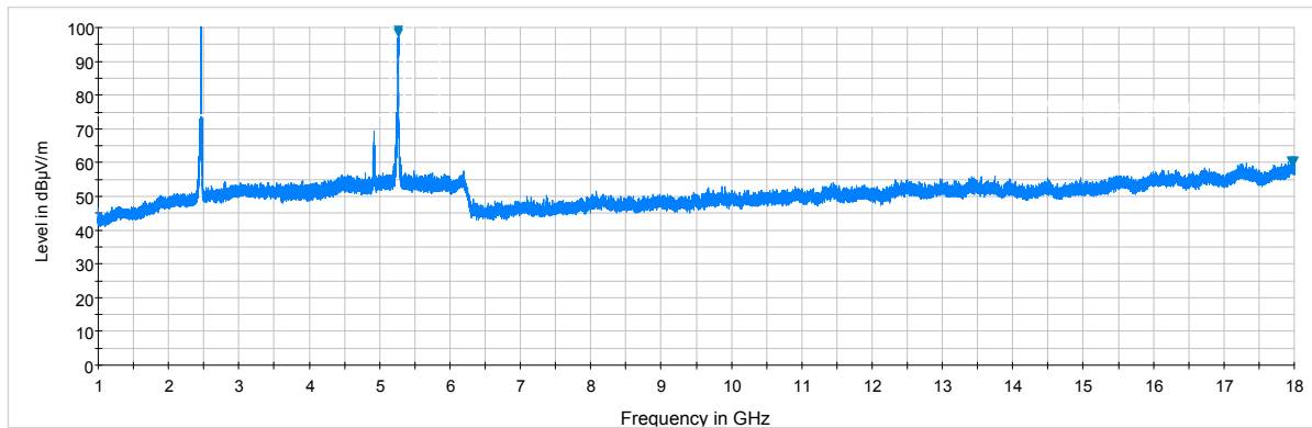
Plot 7-182. Radiated Spurious Plot above 1GHz (Simultaneous Transmission Config-1, Ant. Pol. V)
