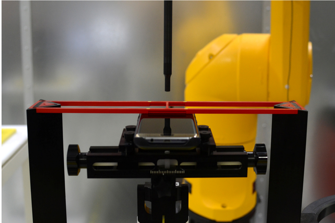
Figure 15-1 Ear Reference Point HAC Phantom Alignment
