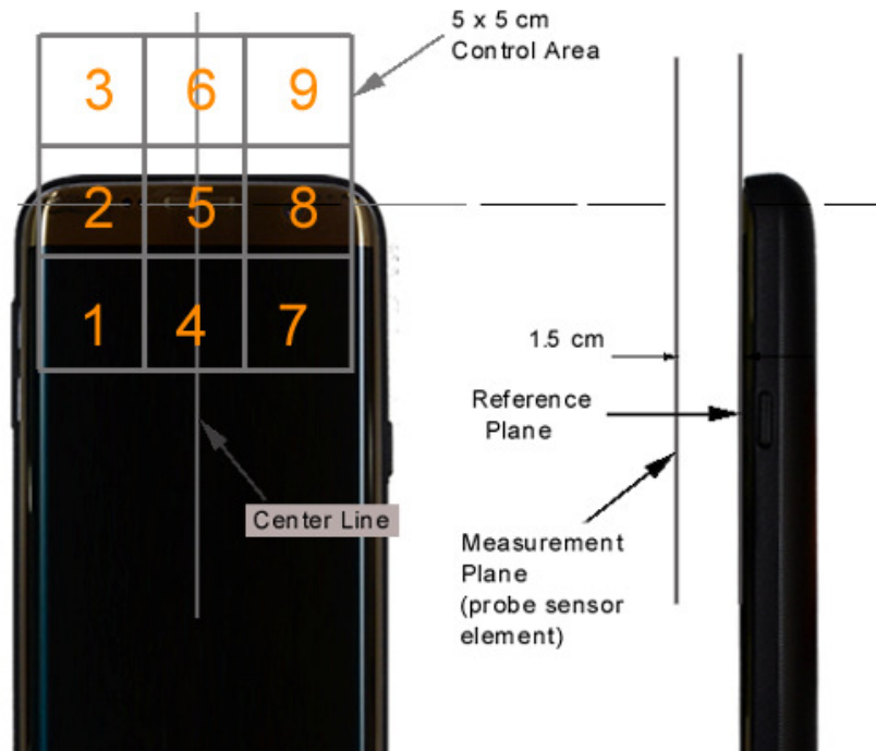
Figure 15-3 5x5 Scan grid above WD
