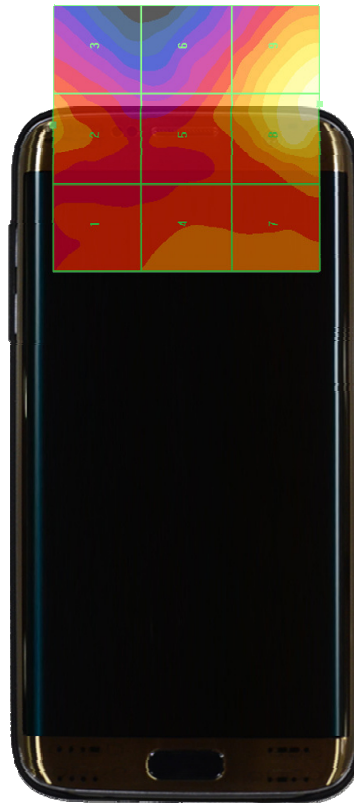
Figure 15-4 E-Field WD Scan overlay
