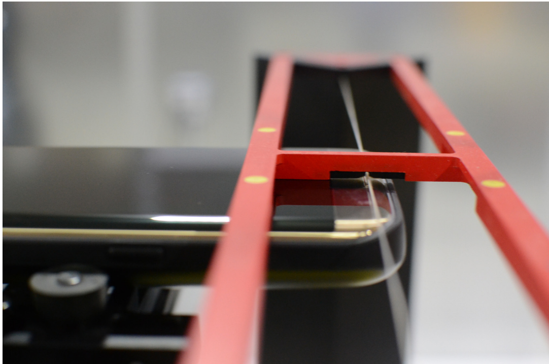
Figure 15-2 HAC Phantom Plane Alignment
