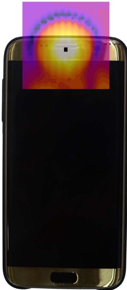
Figure 13-3 Axial T-Coil Scan Overlay Magnetic Field Distributions
