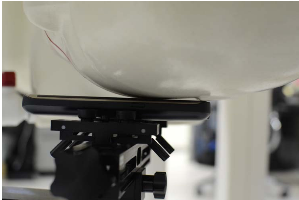
SAR Test Setup Photo 5: Left Cheek Wireless Charging Battery Cover
