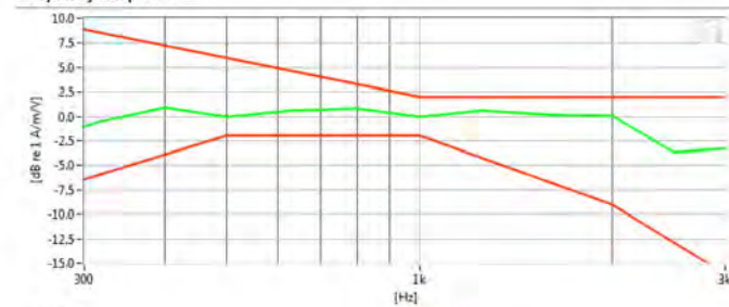
Frequency Response
