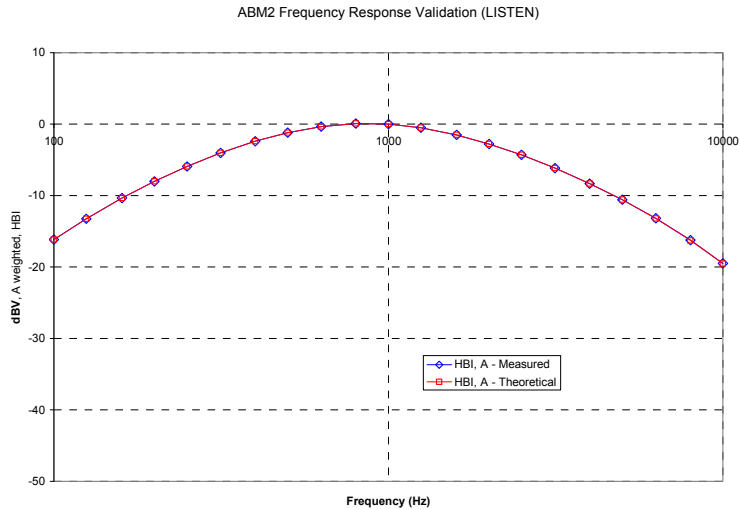
Figure 5-7 ABM2 Frequency Response Validation
