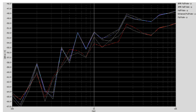
Figure 5-11 Vocoder Analysis for ABM Noise for GSM
