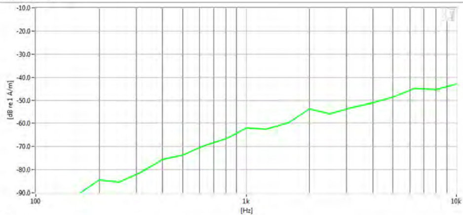
Noise Spectrum
