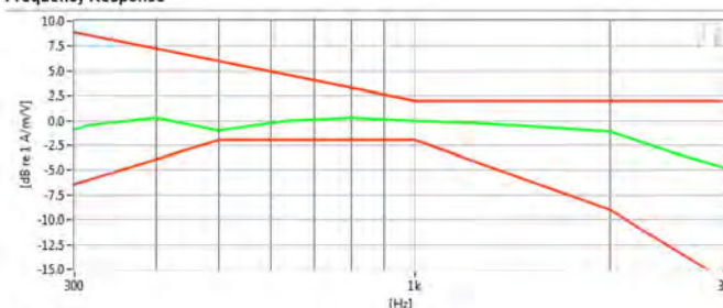
Frequency Response
