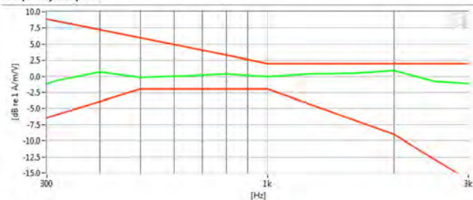
Frequency Response
