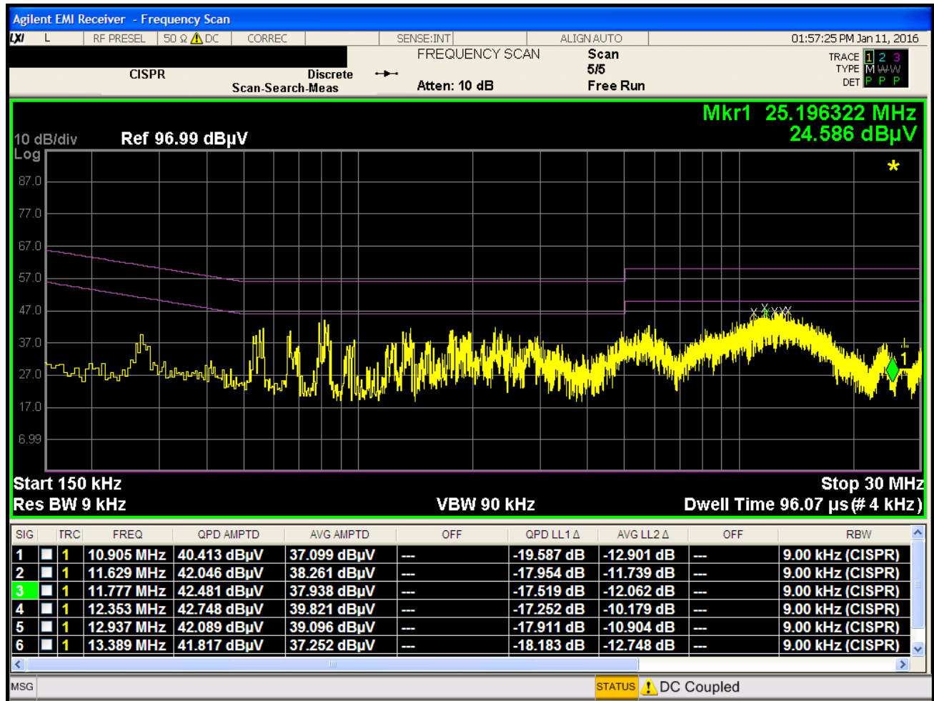
Plot 8-3. Line-Conducted Test Plot (L1) – Terminated in 50 Ohms
