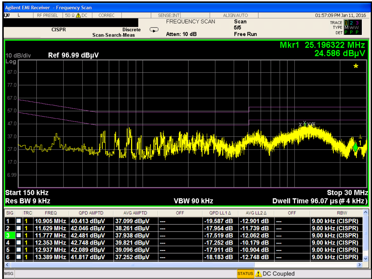
Plot 8-4. Line-Conducted Test Plot (N) – Terminated in 50 Ohms
