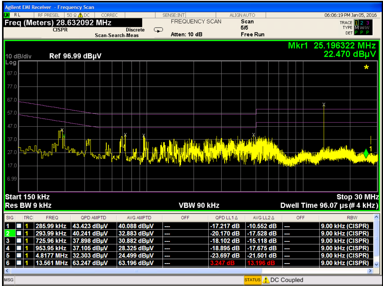
Plot 8-2. Line-Conducted Test Plot (N) with RFID Antenna Attached
