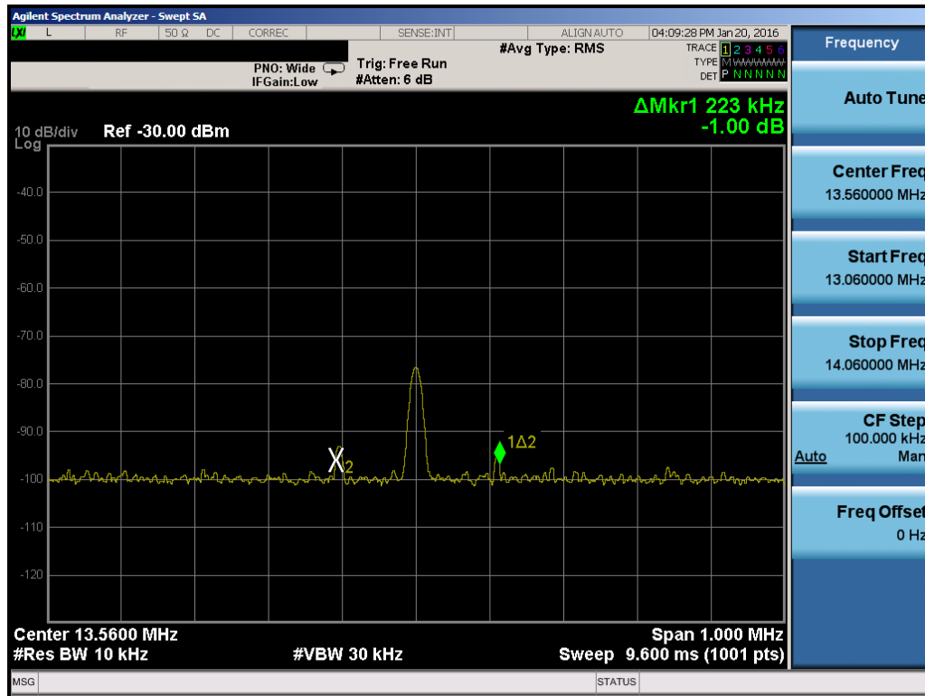
Figure 8-3. 20dB Bandwidth Plot with WCP
