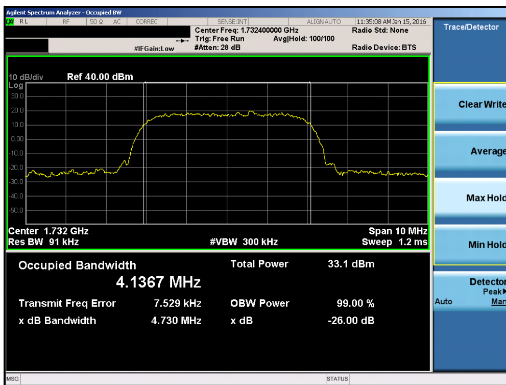
Plot 7-6. Occupied Bandwidth Plot (AWS WCDMA Mode – Ch. 1412)
