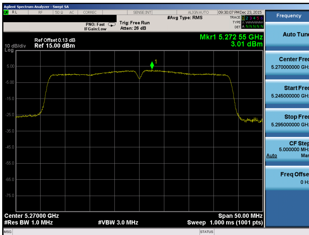
Plot 7-94. Power Spectral Density Plot (40MHz BW 802.11n (UNII Band 2A) – Ch. 54)
