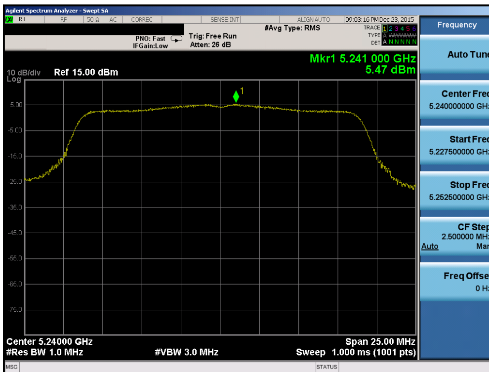
Plot 7-84. Power Spectral Density Plot (20MHz BW 802.11n (UNII Band 1) – Ch. 48)
