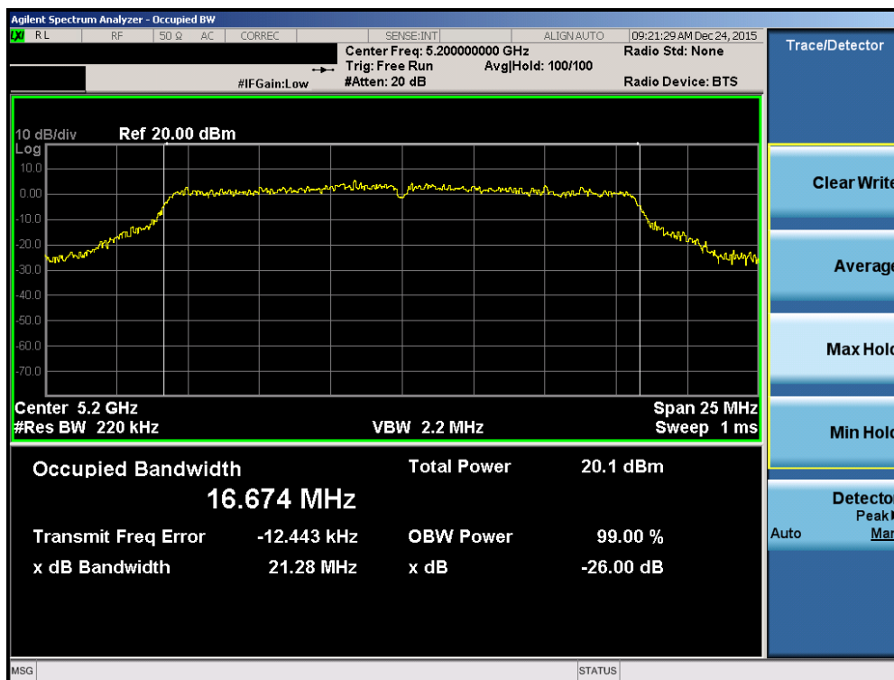
Plot 7-32. 26dB Bandwidth Plot (802.11a (UNII Band 1) – Ch. 40)
