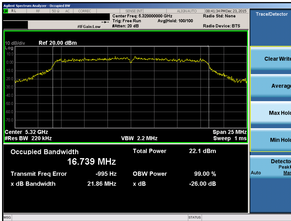
Plot 7-12. 26dB Bandwidth Plot (802.11a (UNII Band 2A) – Ch. 64)
