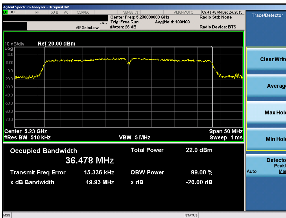
Plot 7-38. 26dB Bandwidth Plot (40MHz BW 802.11n (UNII Band 1) – Ch. 46)
