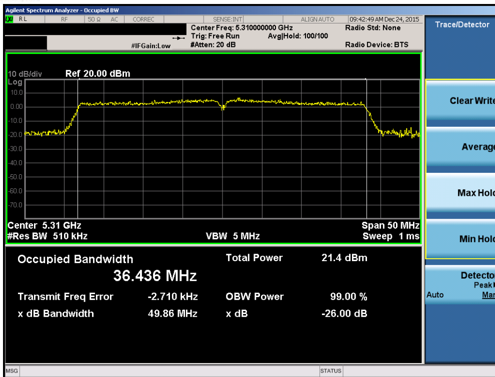
Plot 7-47. 26dB Bandwidth Plot (40MHz BW 802.11n (UNII Band 2A) – Ch. 62)
