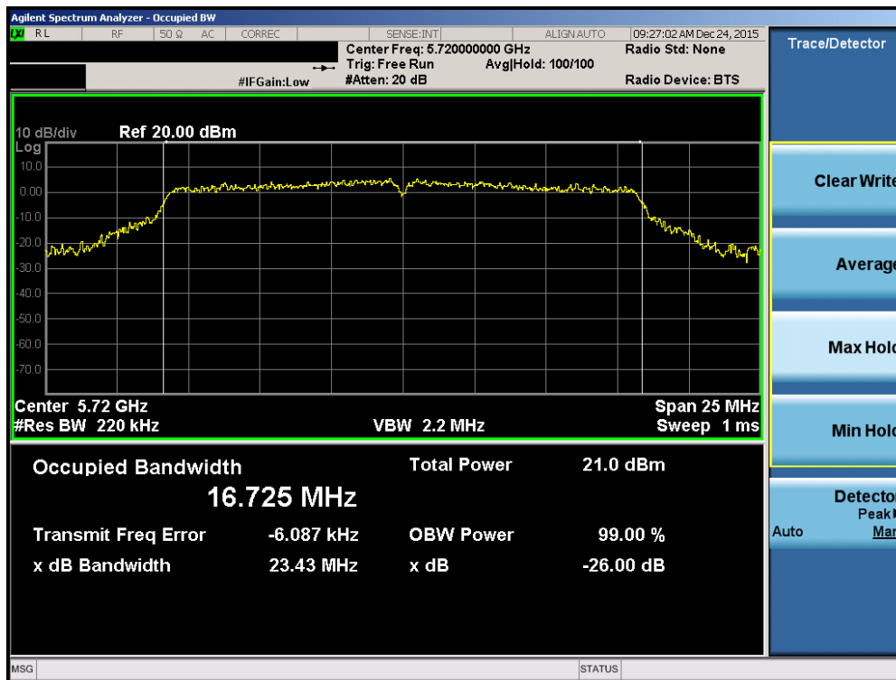
Plot 7-51. 26dB Bandwidth Plot (802.11a (UNII Band 2C) – Ch. 144)
