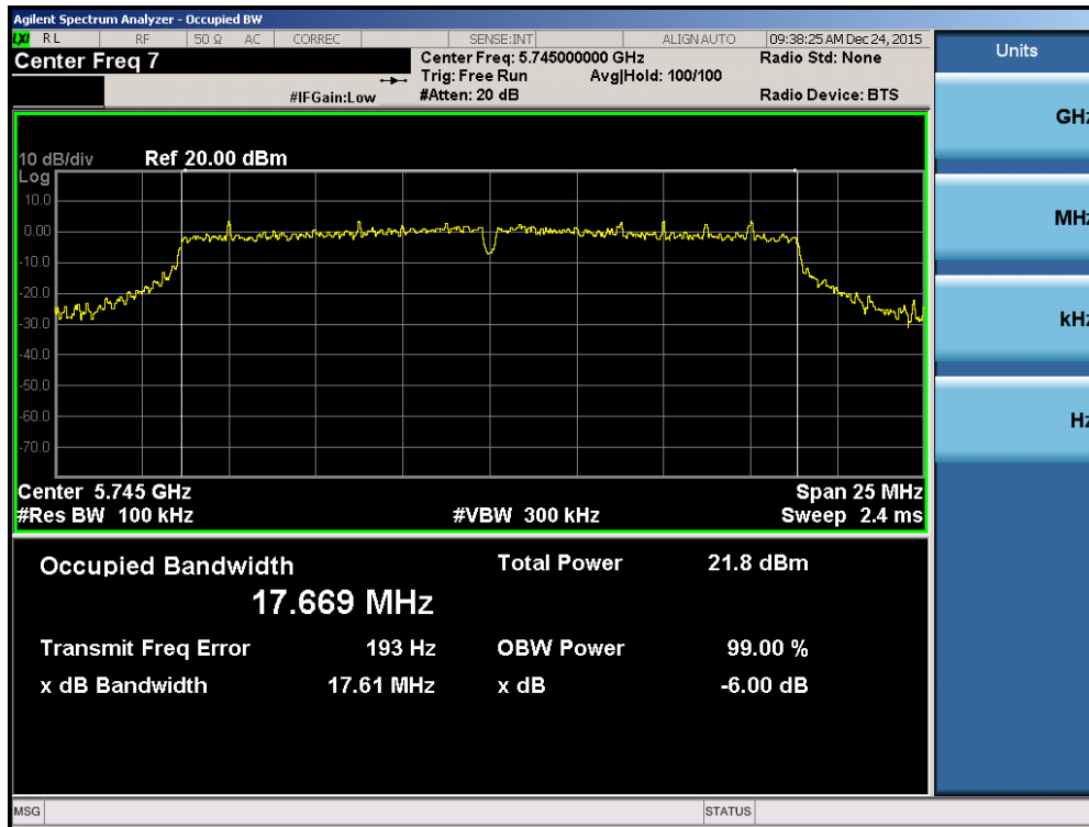
Plot 7-73. 6dB Bandwidth Plot (20MHz BW 802.11n (UNII Band 3) – Ch. 149)
