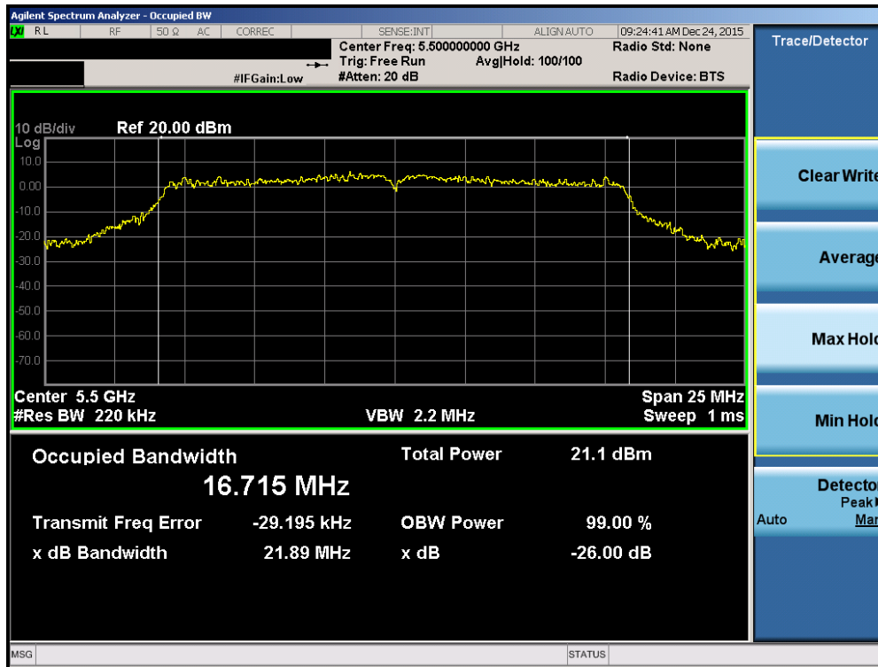
Plot 7-49. 26dB Bandwidth Plot (802.11a (UNII Band 2C) – Ch. 100)
