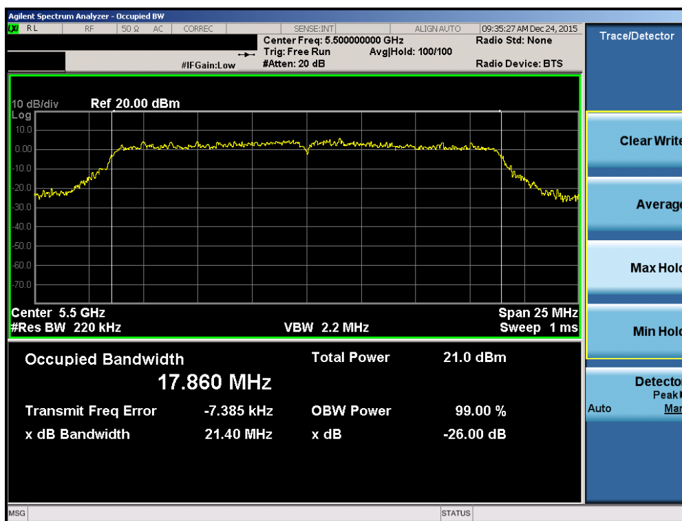
Plot 7-52. 26dB Bandwidth Plot (20MHz BW 802.11n (UNII Band 2C) – Ch. 100)
