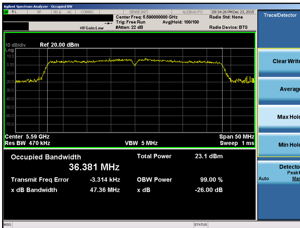
Plot 7-26. 26dB Bandwidth Plot (40MHz BW 802.11n (UNII Band 2C) – Ch. 118)
