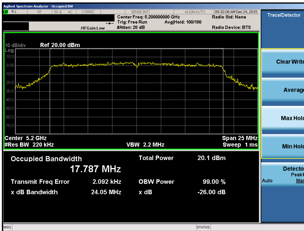
Plot 7-35. 26dB Bandwidth Plot (20MHz BW 802.11n (UNII Band 1) – Ch. 40)
