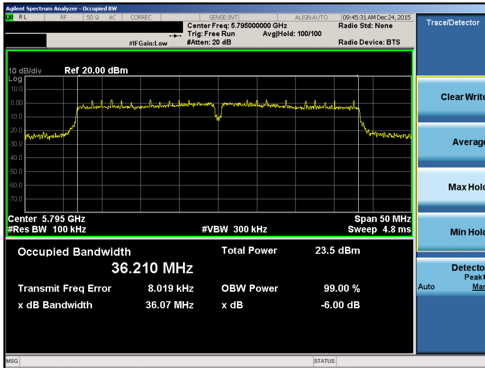
Plot 7-77. 6dB Bandwidth Plot (40MHz BW 802.11n (UNII Band 3) – Ch. 159)
