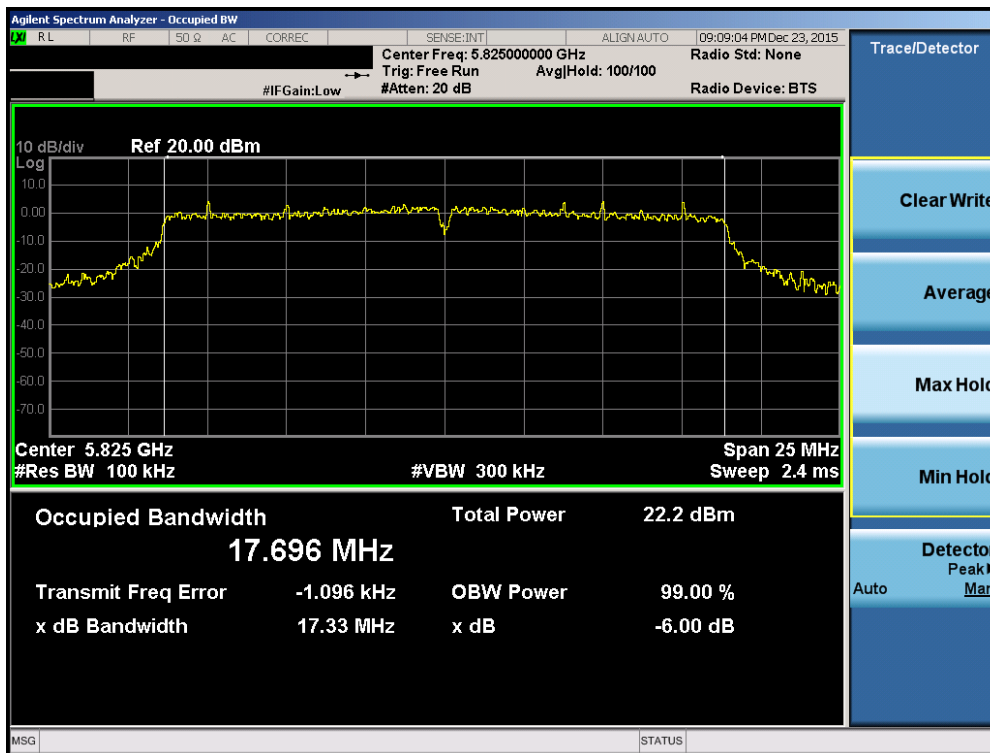
Plot 7-66. 6dB Bandwidth Plot (20MHz BW 802.11n (UNII Band 3) – Ch. 165)
