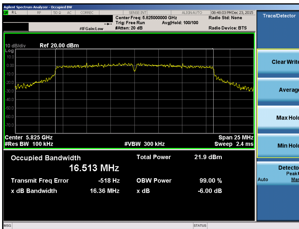
Plot 7-63. 6dB Bandwidth Plot (802.11a (UNII Band 3) – Ch. 165)
