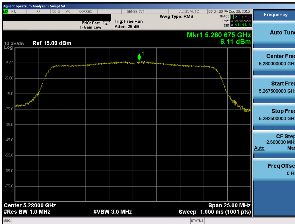
Plot 7-92. Power Spectral Density Plot (20MHz BW 802.11n (UNII Band 2A) – Ch. 56)
