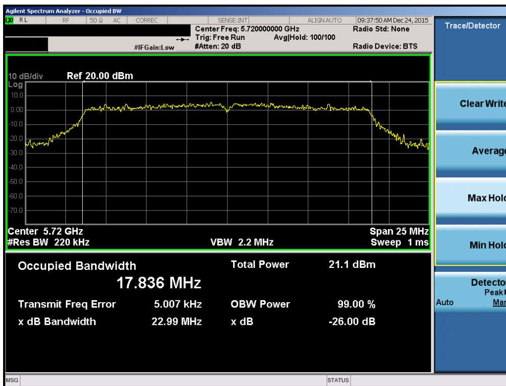
Plot 7-54. 26dB Bandwidth Plot (20MHz BW 802.11n (UNII Band 2C) – Ch. 144)
