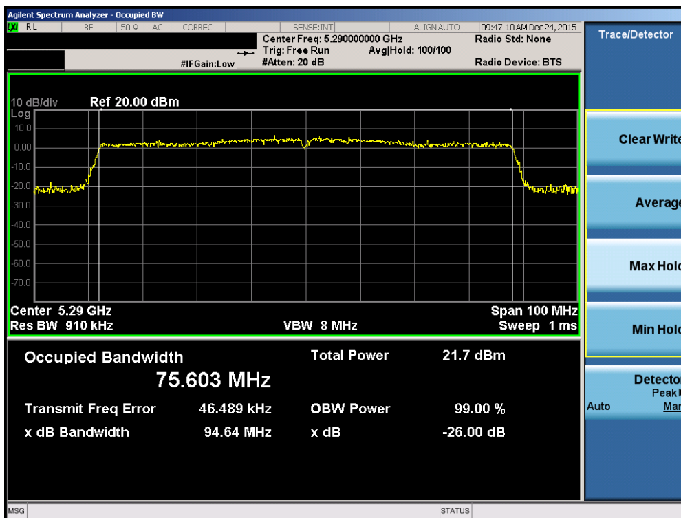
Plot 7-48. 26dB Bandwidth Plot (80MHz BW 802.11ac (UNII Band 2A) – Ch. 58)
