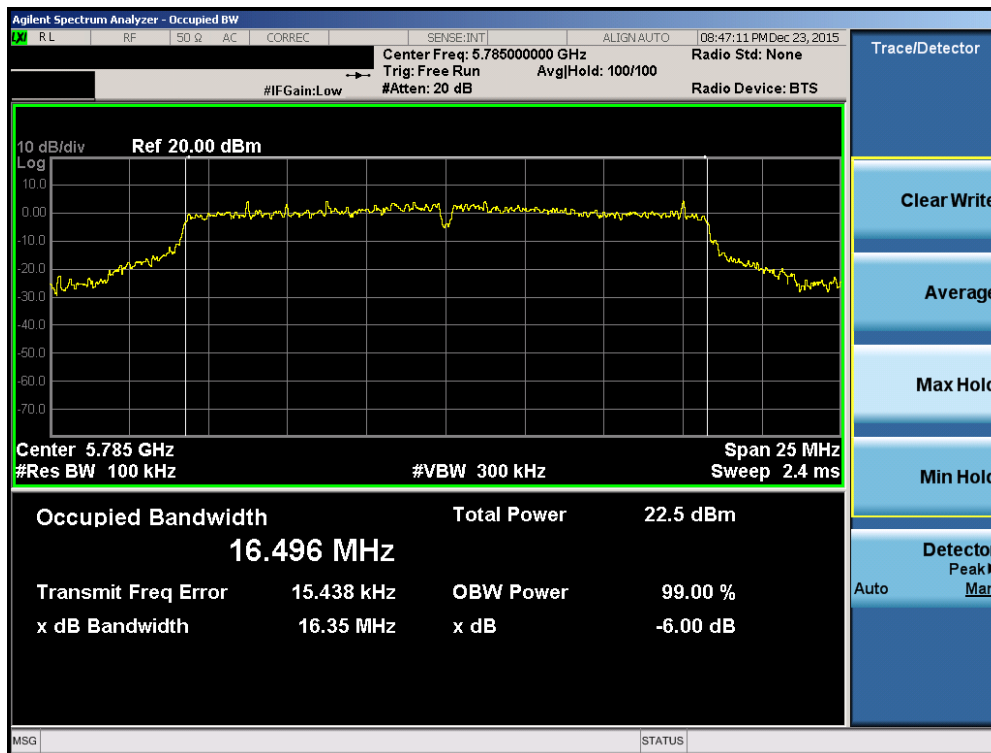
Plot 7-62. 6dB Bandwidth Plot (802.11a (UNII Band 3) – Ch. 157)
