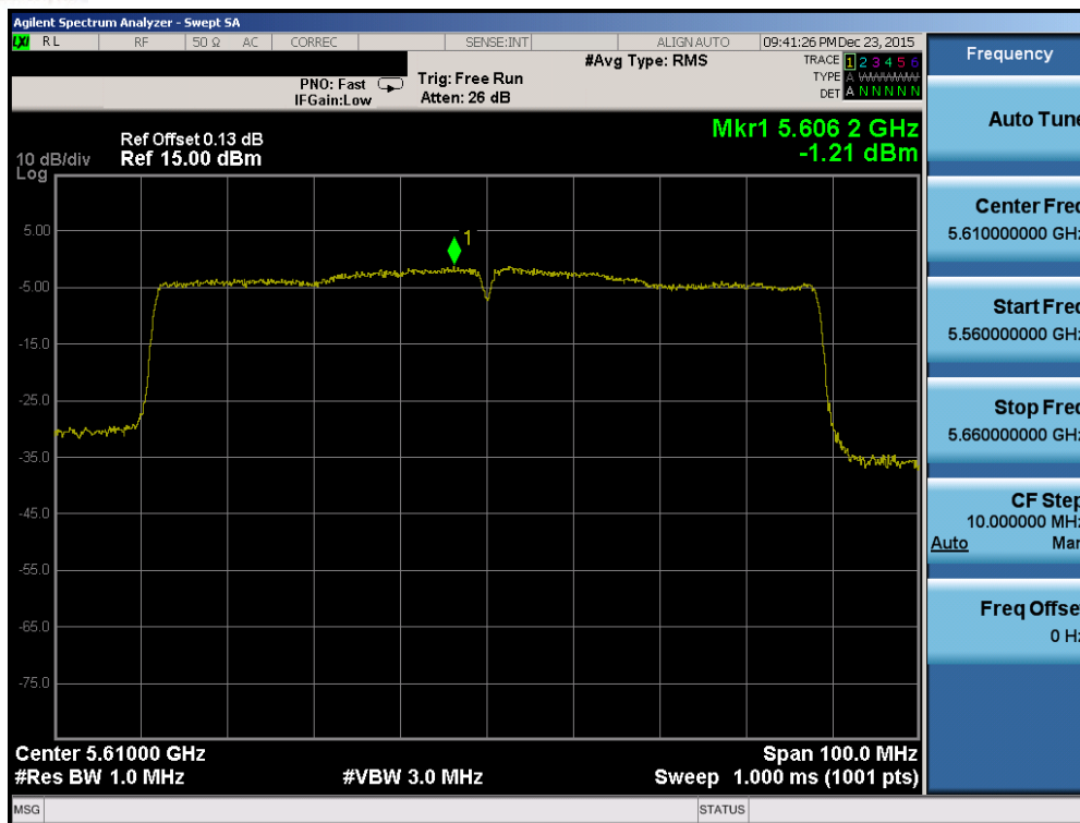
Plot 7-107. Power Spectral Density Plot (80MHz BW 802.11ac (UNII Band 2C) – Ch. 122)
