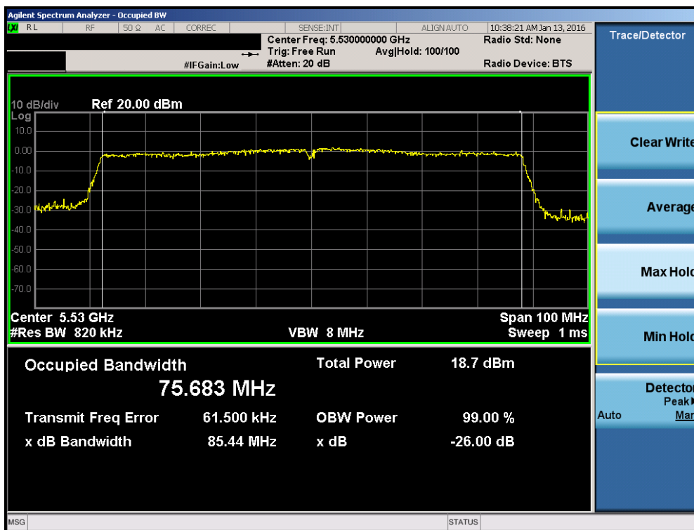
Plot 7-58. 26dB Bandwidth Plot (80MHz BW 802.11ac (UNII Band 2C) – Ch. 106)
