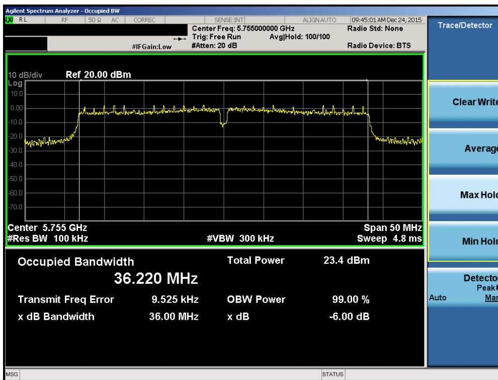
Plot 7-76. 6dB Bandwidth Plot (40MHz BW 802.11n (UNII Band 3) – Ch. 151)
