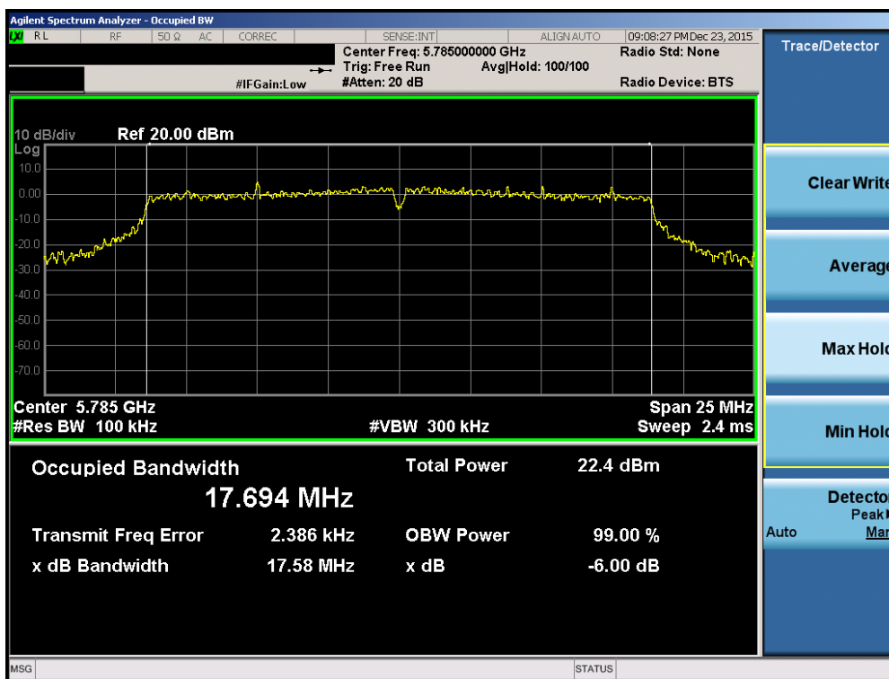
Plot 7-65. 6dB Bandwidth Plot (20MHz BW 802.11n (UNII Band 3) – Ch. 157)
