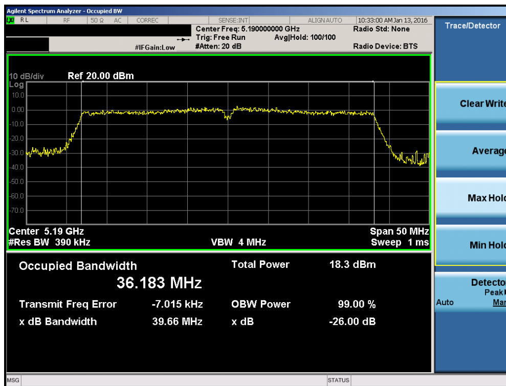
Plot 7-37. 26dB Bandwidth Plot (40MHz BW 802.11n (UNII Band 1) – Ch. 38)
