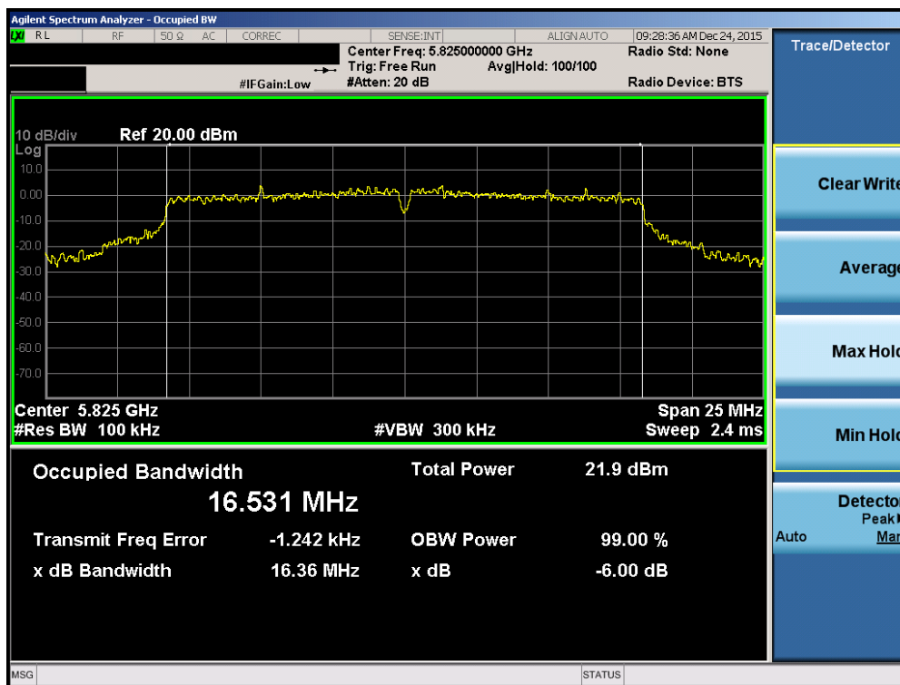
Plot 7-72. 6dB Bandwidth Plot (802.11a (UNII Band 3) – Ch. 165)
