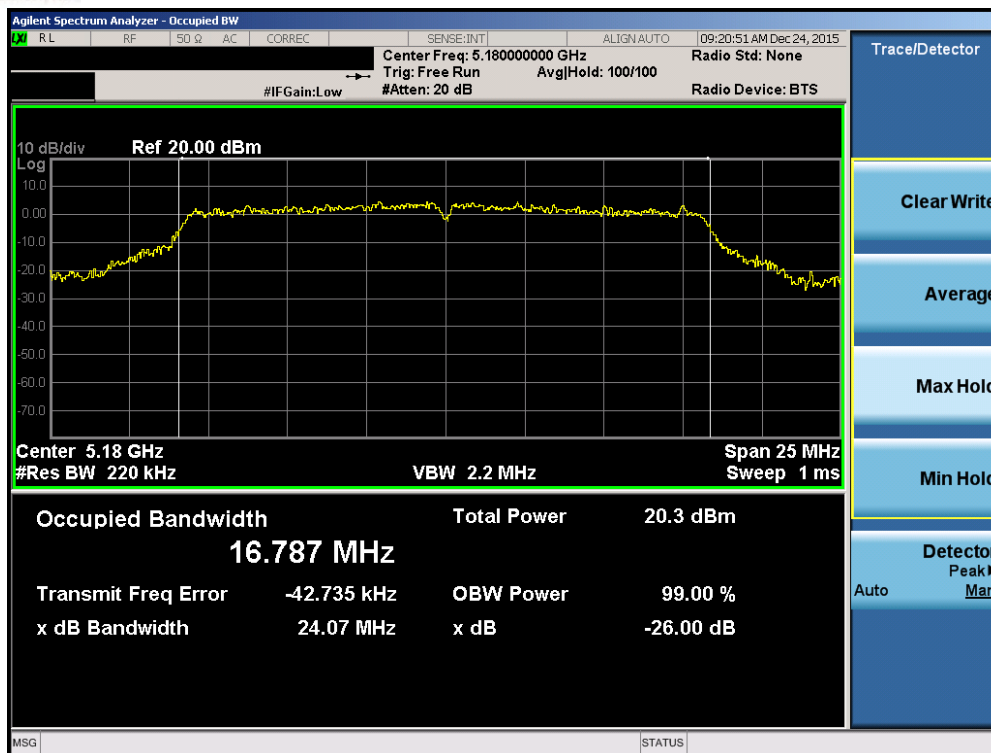
Plot 7-31. 26dB Bandwidth Plot (802.11a (UNII Band 1) – Ch. 36)
