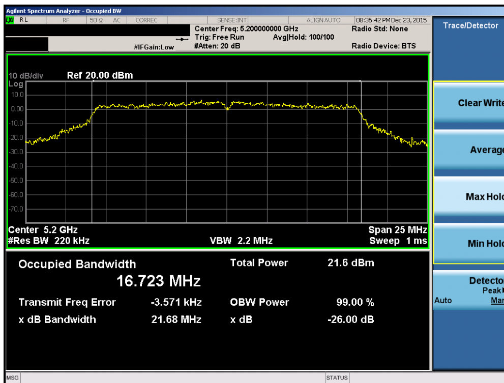
Plot 7-2. 26dB Bandwidth Plot (802.11a (UNII Band 1) – Ch. 40)
