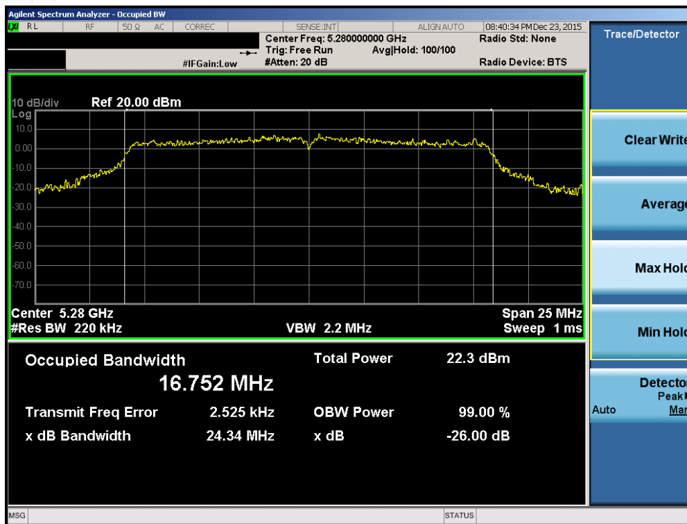
Plot 7-11. 26dB Bandwidth Plot (802.11a (UNII Band 2A) – Ch. 56)
