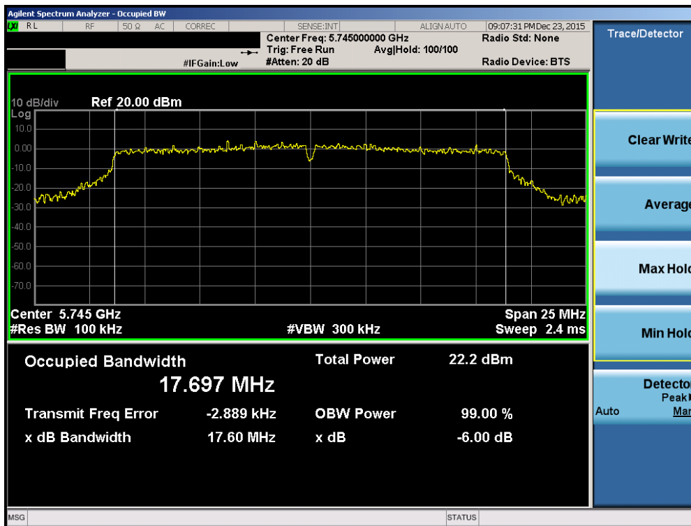
Plot 7-64. 6dB Bandwidth Plot (20MHz BW 802.11n (UNII Band 3) – Ch. 149)
