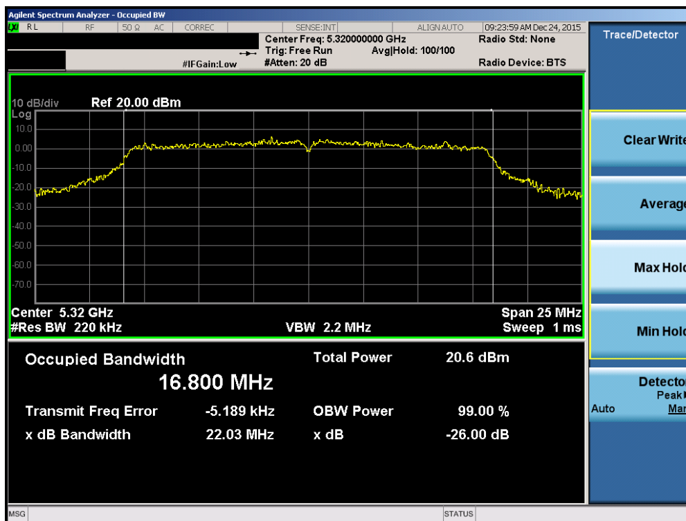
Plot 7-42. 26dB Bandwidth Plot (802.11a (UNII Band 2A) – Ch. 64)
