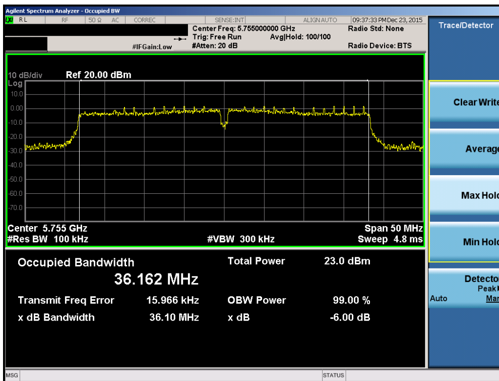
Plot 7-67. 6dB Bandwidth Plot (40MHz BW 802.11n (UNII Band 3) – Ch. 151)
