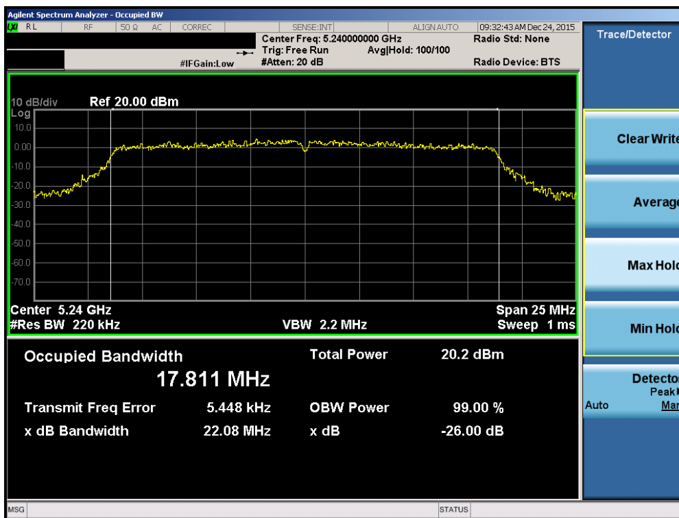
Plot 7-36. 26dB Bandwidth Plot (20MHz BW 802.11n (UNII Band 1) – Ch. 48)
