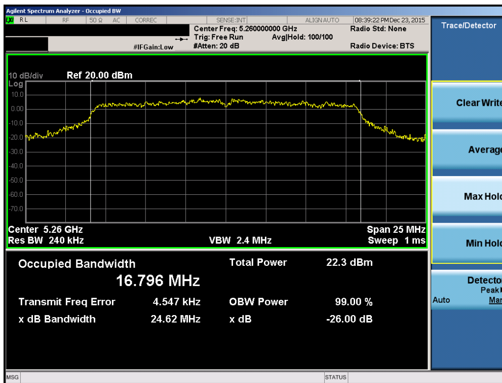
Plot 7-10. 26dB Bandwidth Plot (802.11a (UNII Band 2A) – Ch. 52)
