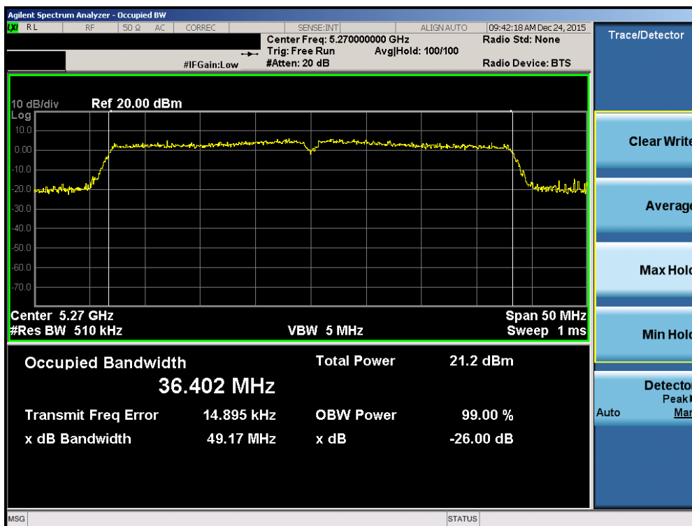
Plot 7-46. 26dB Bandwidth Plot (40MHz BW 802.11n (UNII Band 2A) – Ch. 54)
