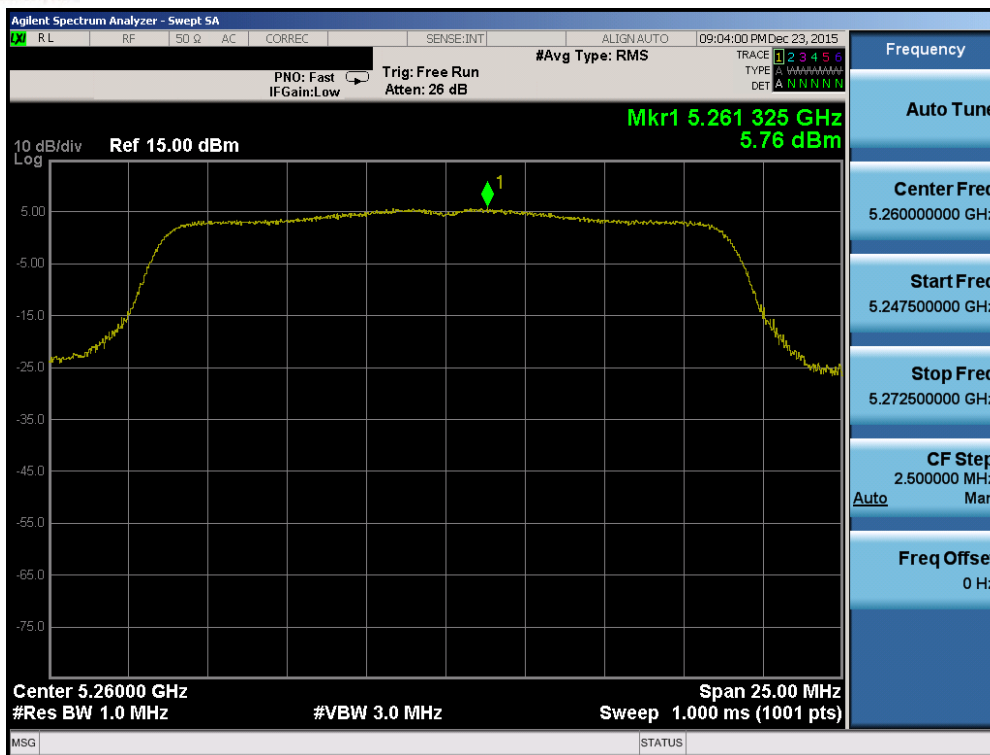
Plot 7-91. Power Spectral Density Plot (20MHz BW 802.11n (UNII Band 2A) – Ch. 52)
