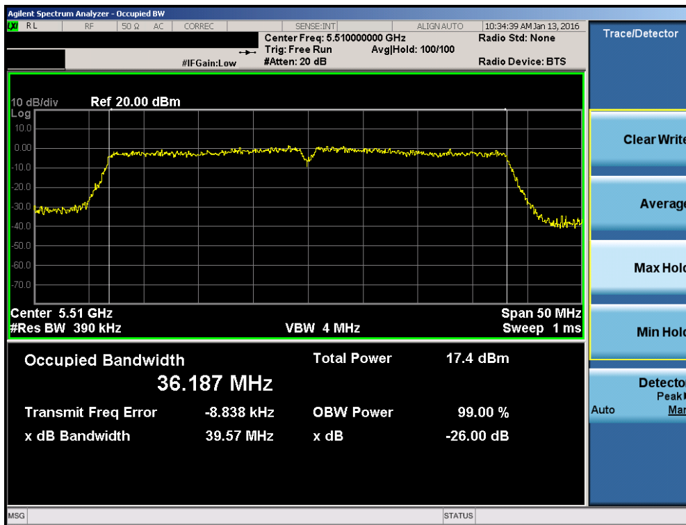
Plot 7-55. 26dB Bandwidth Plot (40MHz BW 802.11n (UNII Band 2C) – Ch. 102)
