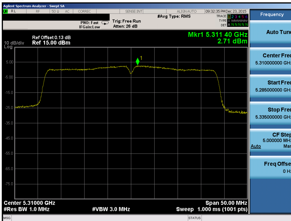
Plot 7-95. Power Spectral Density Plot (40MHz BW 802.11n (UNII Band 2A) – Ch. 62)
