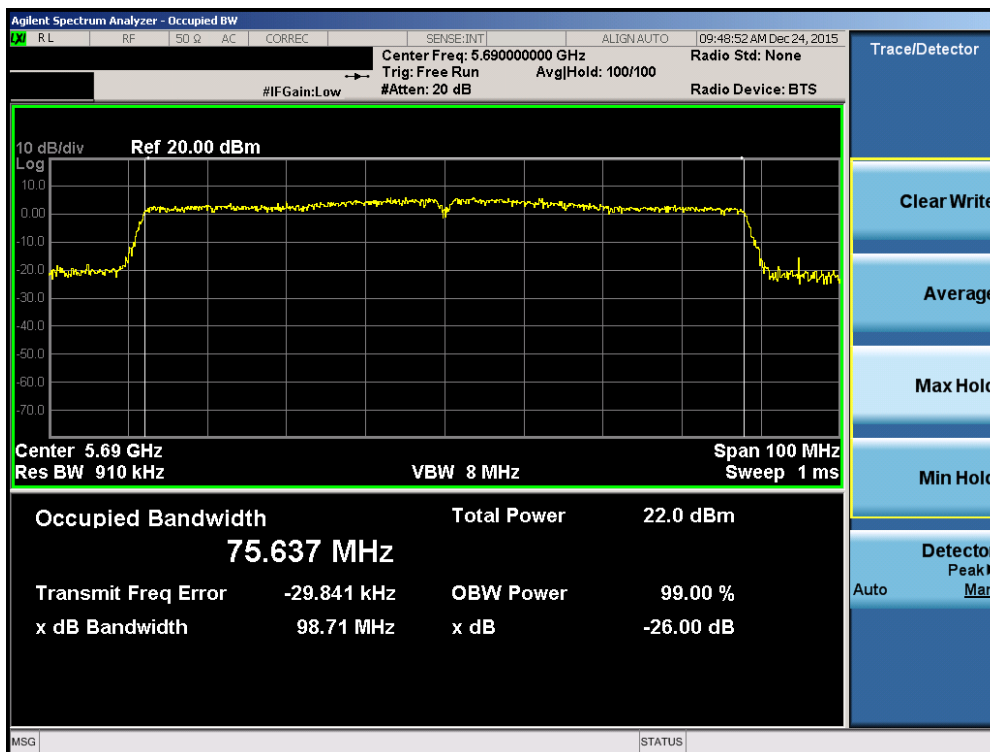
Plot 7-60. 26dB Bandwidth Plot (80MHz BW 802.11ac (UNII Band 2C) – Ch. 138)
