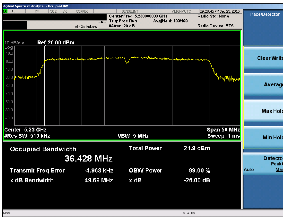
Plot 7-8. 26dB Bandwidth Plot (40MHz BW 802.11n (UNII Band 1) – Ch. 46)
