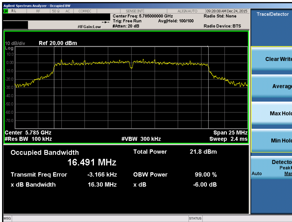
Plot 7-71. 6dB Bandwidth Plot (802.11a (UNII Band 3) – Ch. 157)
