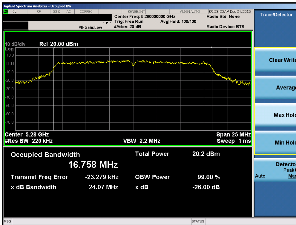
Plot 7-41. 26dB Bandwidth Plot (802.11a (UNII Band 2A) – Ch. 56)
