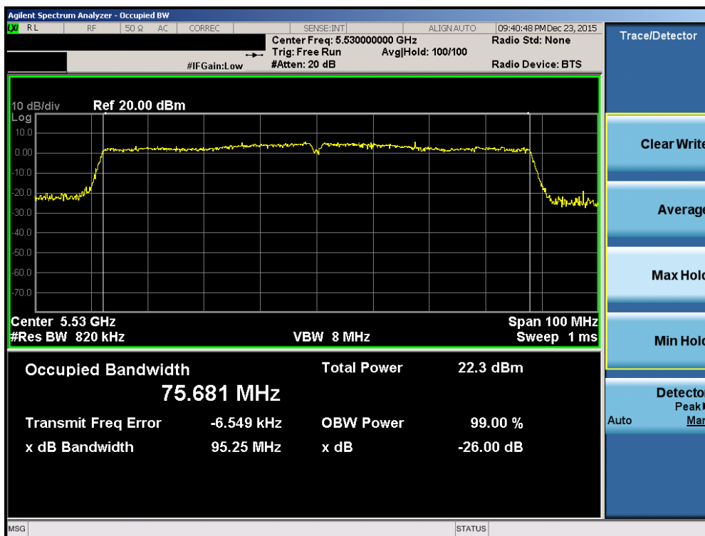
Plot 7-28. 26dB Bandwidth Plot (80MHz BW 802.11ac (UNII Band 2C) – Ch. 106)
