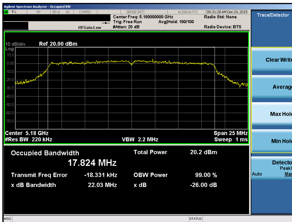
Plot 7-34. 26dB Bandwidth Plot (20MHz BW 802.11n (UNII Band 1) – Ch. 36)
