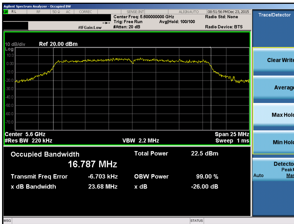
Plot 7-20. 26dB Bandwidth Plot (802.11a (UNII Band 2C) – Ch. 120)
