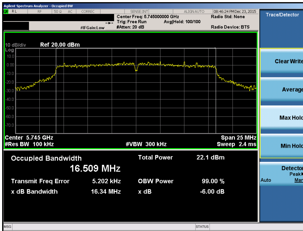
Plot 7-61. 6dB Bandwidth Plot (802.11a (UNII Band 3) – Ch. 149)
