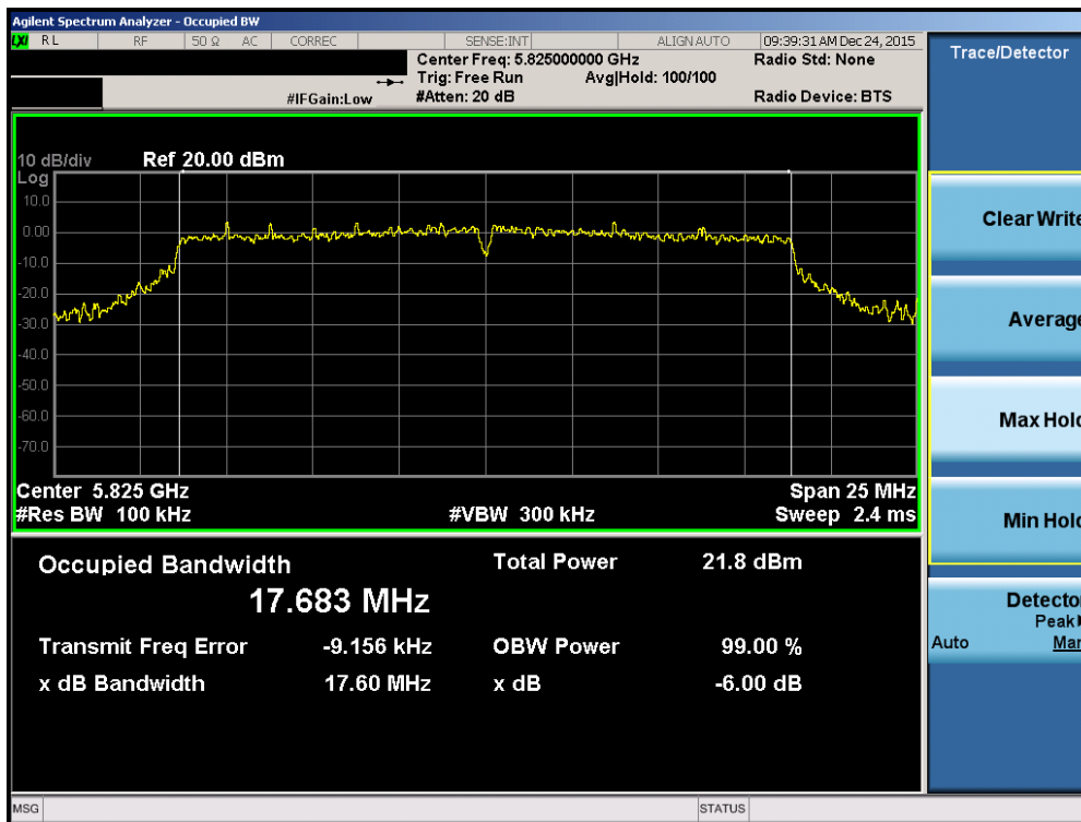
Plot 7-75. 6dB Bandwidth Plot (20MHz BW 802.11n (UNII Band 3) – Ch. 165)
