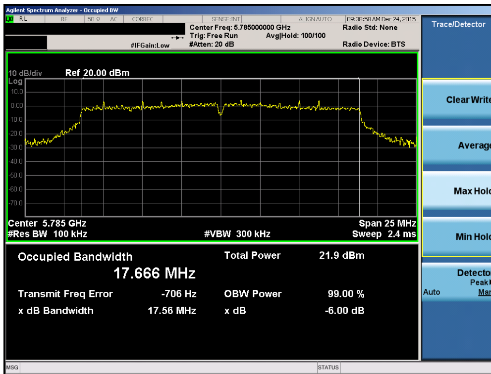
Plot 7-74. 6dB Bandwidth Plot (20MHz BW 802.11n (UNII Band 3) – Ch. 157)
