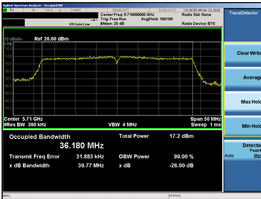
Plot 7-57. 26dB Bandwidth Plot (40MHz BW 802.11n (UNII Band 2C) – Ch. 142)
