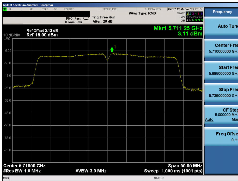
Plot 7-105. Power Spectral Density Plot (40MHz BW 802.11n (UNII Band 2C) – Ch. 142)
