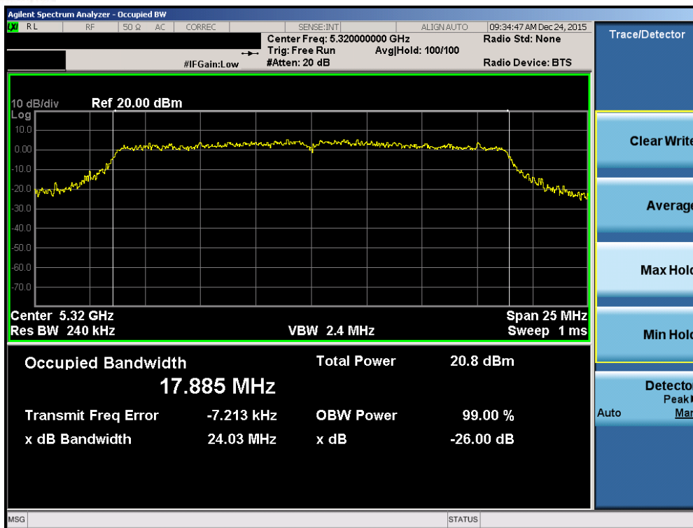
Plot 7-45. 26dB Bandwidth Plot (20MHz BW 802.11n (UNII Band 2A) – Ch. 64)
