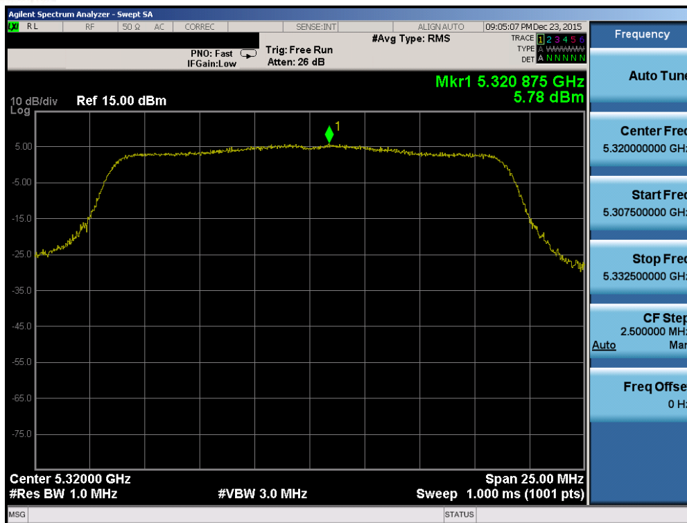
Plot 7-93. Power Spectral Density Plot (20MHz BW 802.11n (UNII Band 2A) – Ch. 64)
