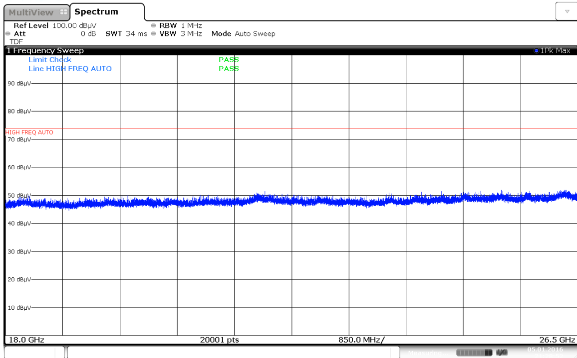
Plot 7-181. Radiated Spurious Plot 18GHz – 26.5GHz (Simultaneous Transmission Config-1 Ant. Pol. V)
