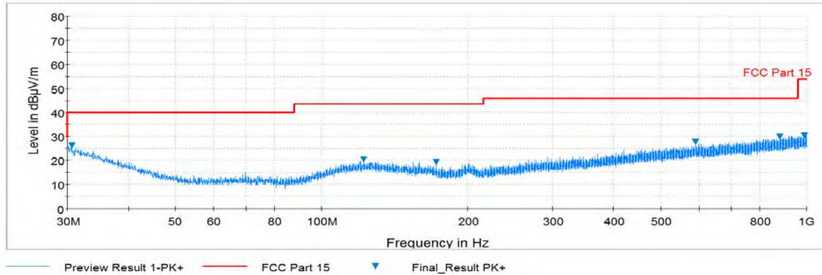
Plot 7-269. Radiated Spurious Plot below 1GHz (802.11a – U3 Ch. 157, Ant. Pol. H)
