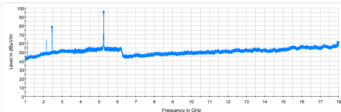
Plot 7-183. Radiated Spurious Plot above 1GHz (Simultaneous Transmission Config-2, Ant. Pol. H)
