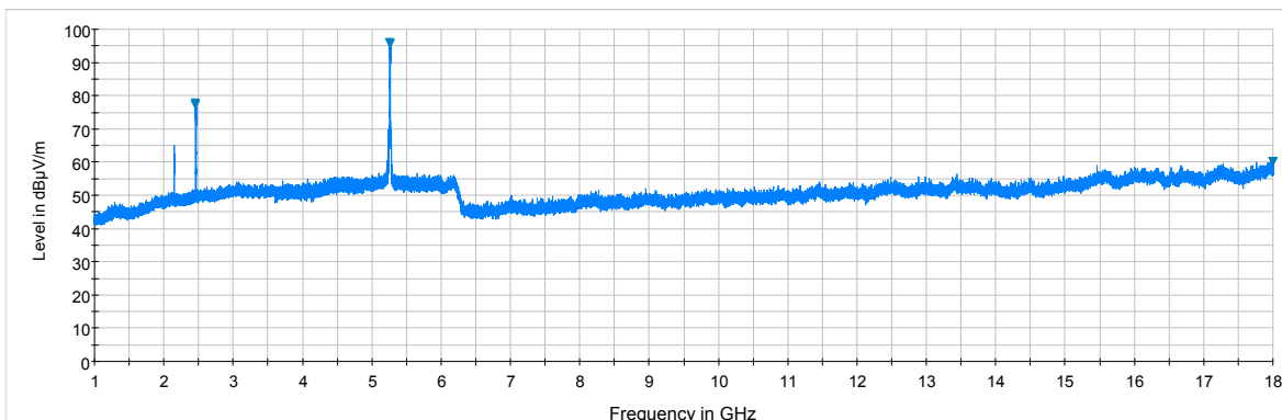
Plot 7-184. Radiated Spurious Plot above 1GHz (Simultaneous Transmission Config-2, Ant. Pol. V)
