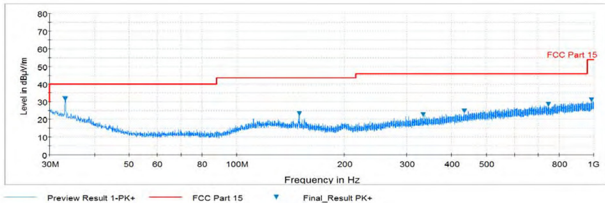
Plot 7-270. Radiated Spurious Plot below 1GHz (802.11a – U3 Ch. 157, Ant. Pol. V)
