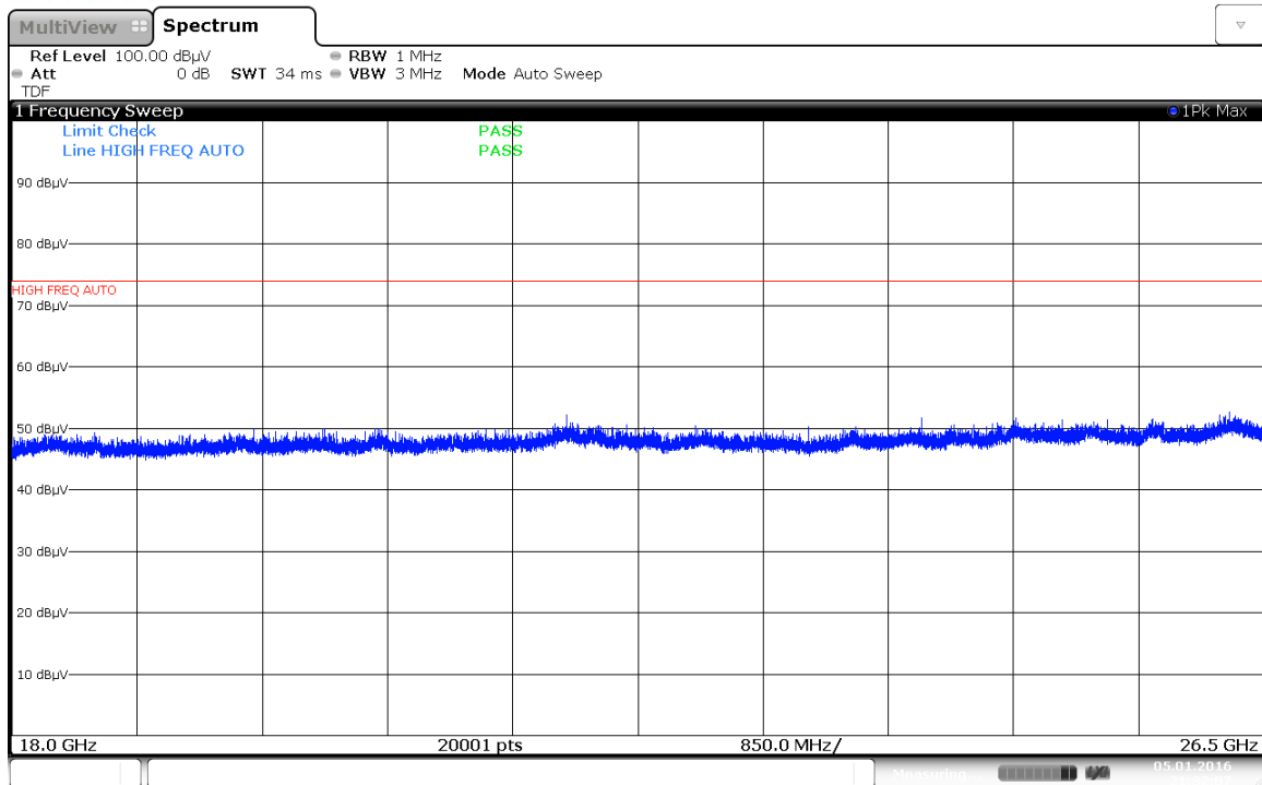
Plot 7-187. Radiated Spurious Plot 18GHz – 26.5GHz (Simultaneous Transmission Config-2 Ant. Pol. V)
