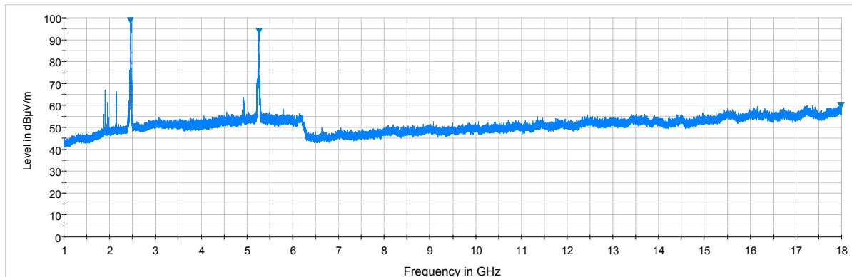
Plot 7-178. Radiated Spurious Plot above 1GHz (Simultaneous Transmission Config-1, Ant. Pol. V)
