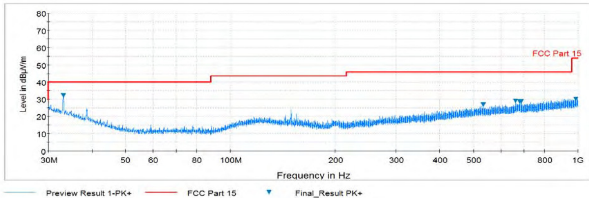
Plot 7-272. Radiated Spurious Plot below 1GHz (802.11a – U3 Ch. 157, Ant. Pol. V)
