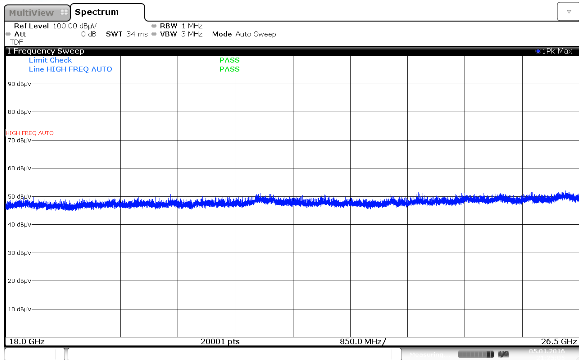
Plot 7-179. Radiated Spurious Plot 18GHz – 26.5GHz (Simultaneous Transmission Config-1 Ant. Pol. H)
