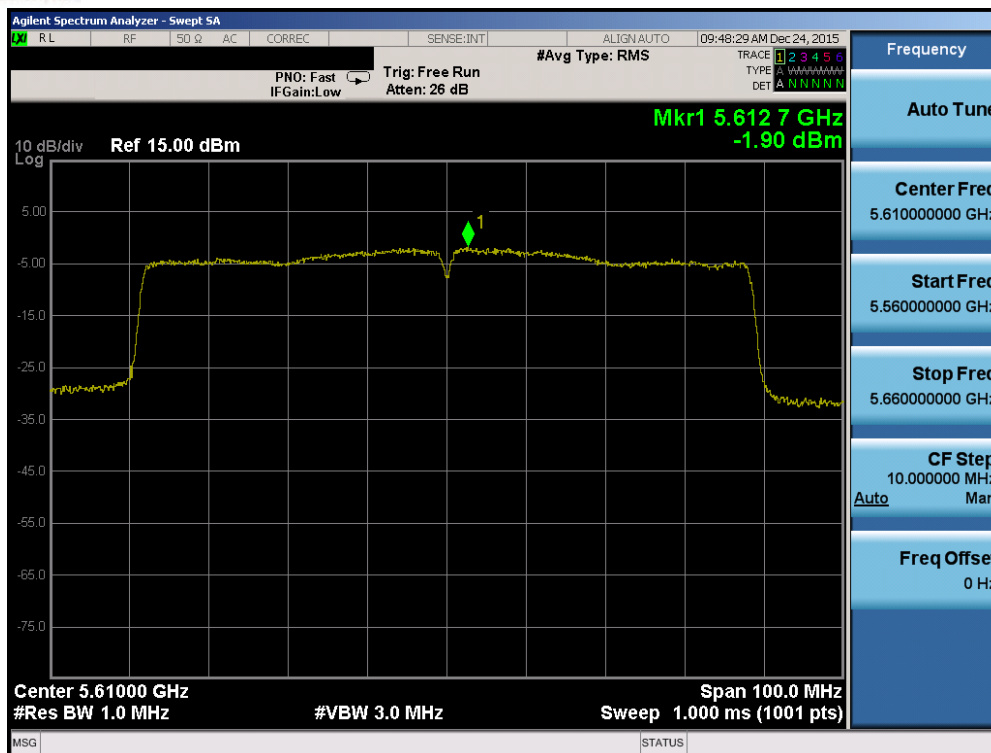
Plot 7-146. Power Spectral Density Plot (80MHz BW 802.11ac (UNII Band 2C) – Ch. 122)
