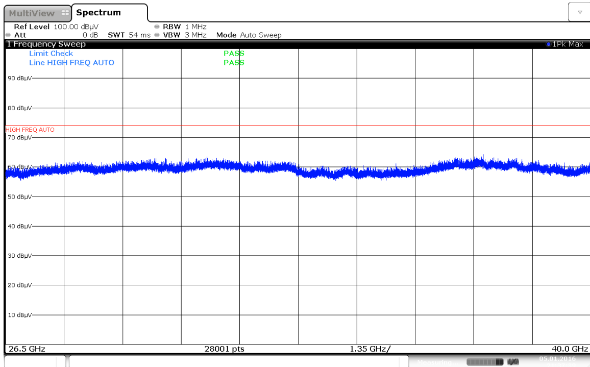
Plot 7-180. Radiated Spurious Plot above 26.5GHz (Simultaneous Transmission Config-1 Ant. Pol. H)
