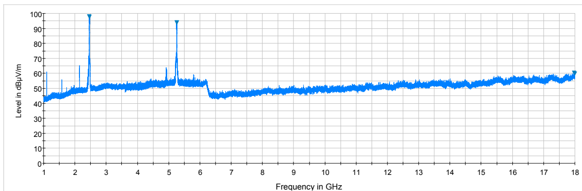
Plot 7-177. Radiated Spurious Plot above 1GHz (Simultaneous Transmission Config-1, Ant. Pol. H)
