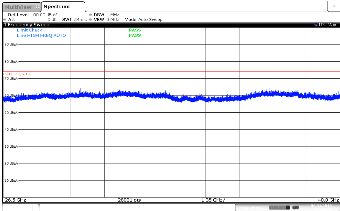
Plot 7-182. Radiated Spurious Plot above 26.5GHz (Simultaneous Transmission Config-1 Ant. Pol. H)
