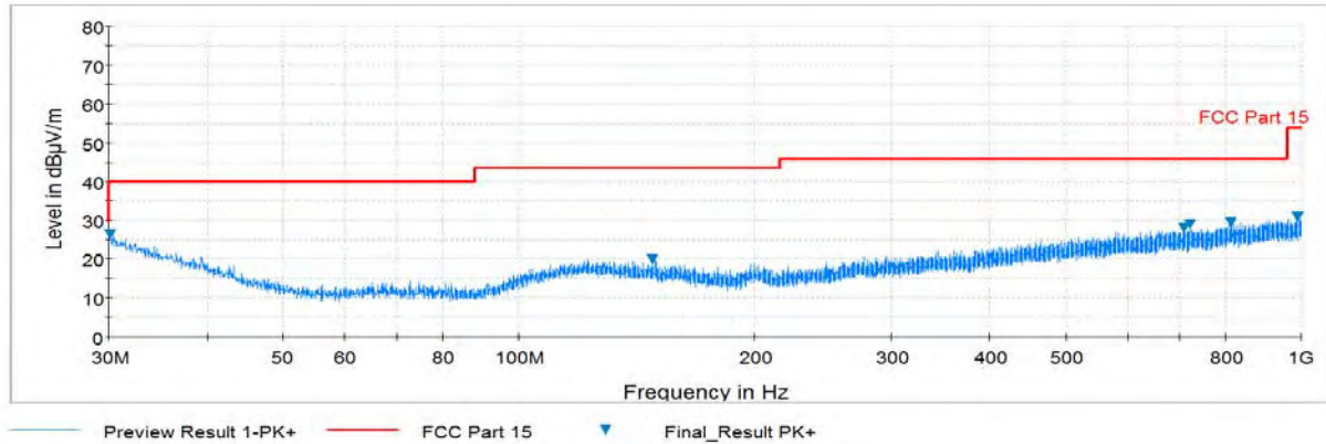
Plot 7-271. Radiated Spurious Plot below 1GHz (802.11a – U3 Ch. 157, Ant. Pol. H)
