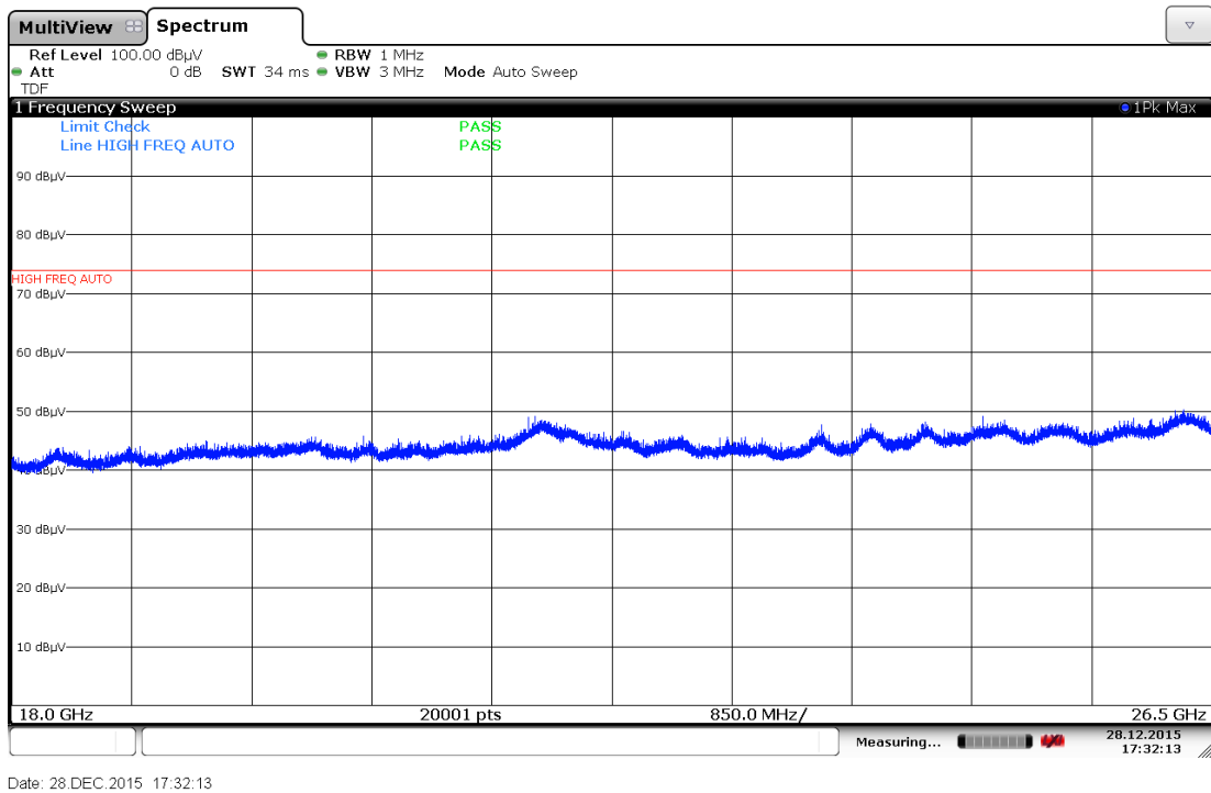
Plot 7-76. Radiated Spurious Plot above 18GHz (Pol. V)
