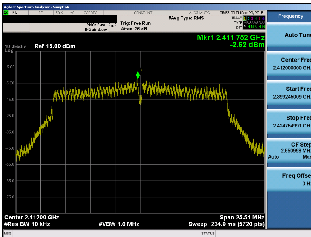
Plot 7-34. Power Spectral Density Plot (802.11n (2.4GHz) – Ch. 1)
