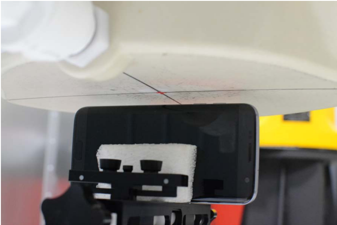
SAR Test Setup Photo 11- Left Edge
