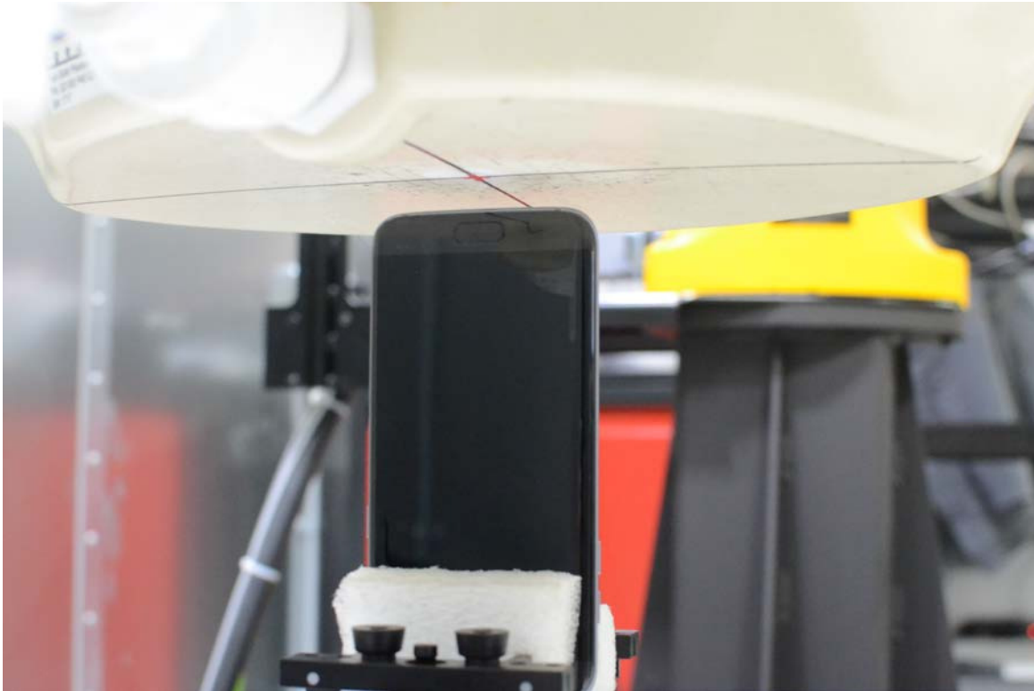
SAR Test Setup Photo 9 - Bottom Edge
