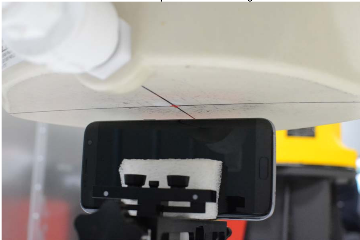
SAR Test Setup Photo 10 - Right Edge
