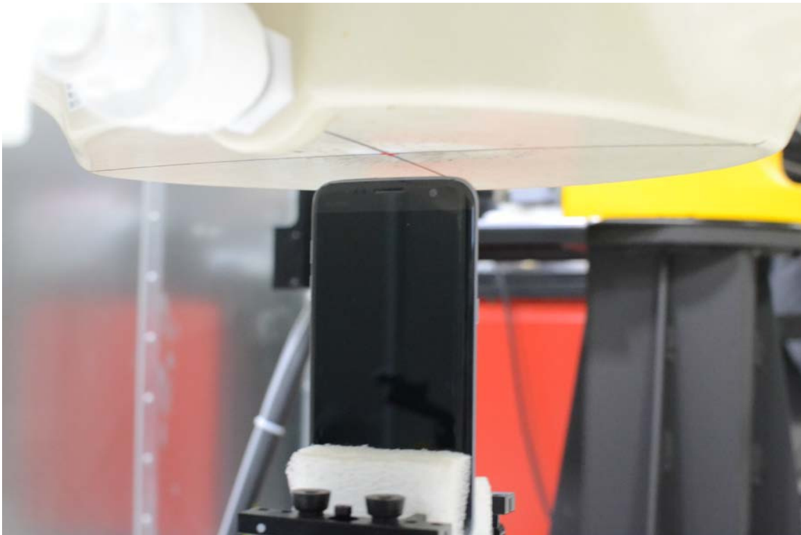
SAR Test Setup Photo 8 - Top Edge
