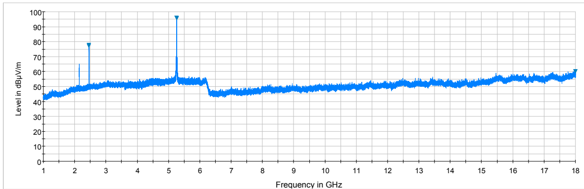
Plot 7-184. Radiated Spurious Plot above 1GHz (Simultaneous Transmission Config-2, Ant. Pol. V)
