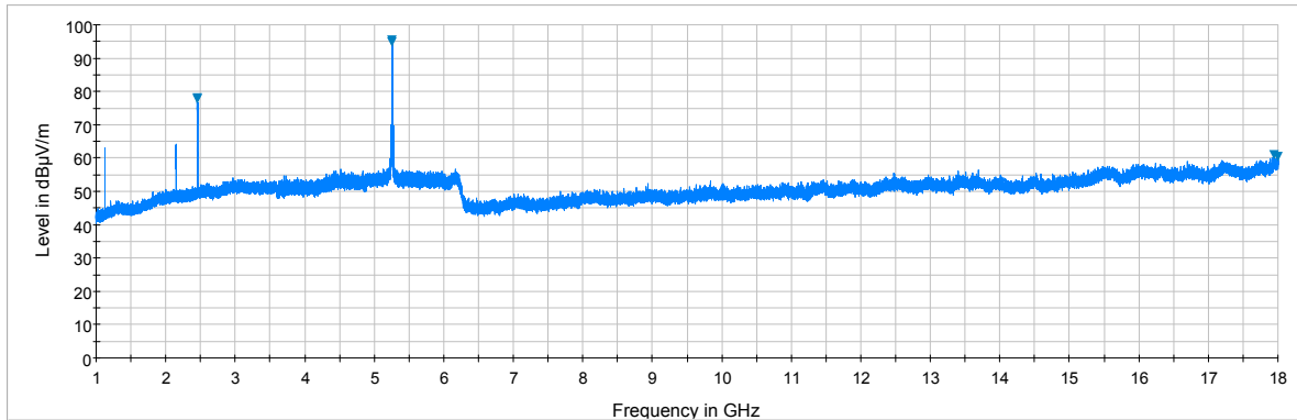
Plot 7-183. Radiated Spurious Plot above 1GHz (Simultaneous Transmission Config-2, Ant. Pol. H)
