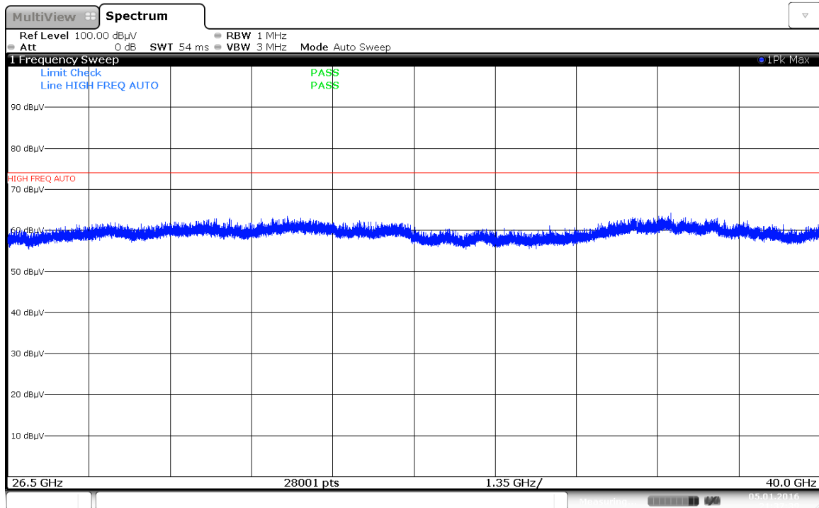
Plot 7-180. Radiated Spurious Plot above 26.5GHz (Simultaneous Transmission Config-1 Ant. Pol. H)
