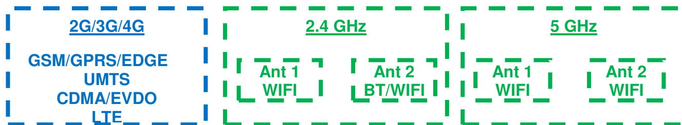
Figure 1-A Simultaneous Transmission Paths
