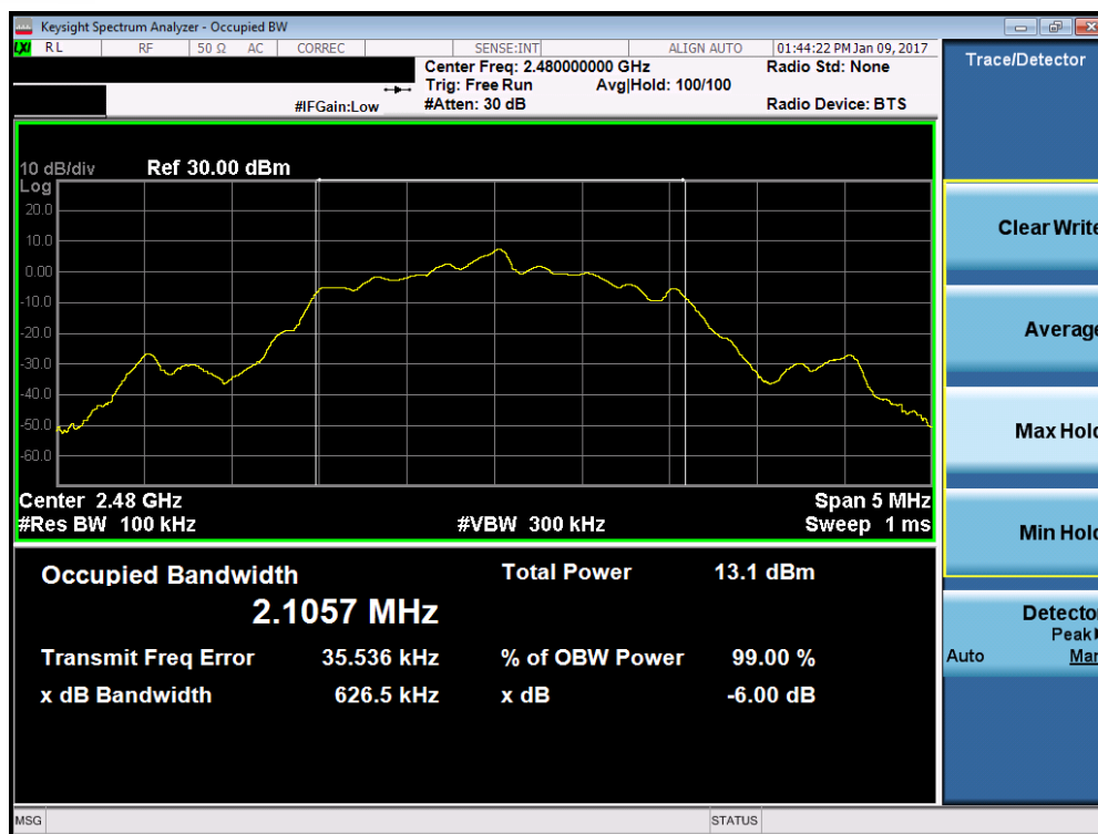
Plot 7-6. 6dB Bandwidth Plot (Bluetooth (LE), 2Mbps – Ch. 39)
