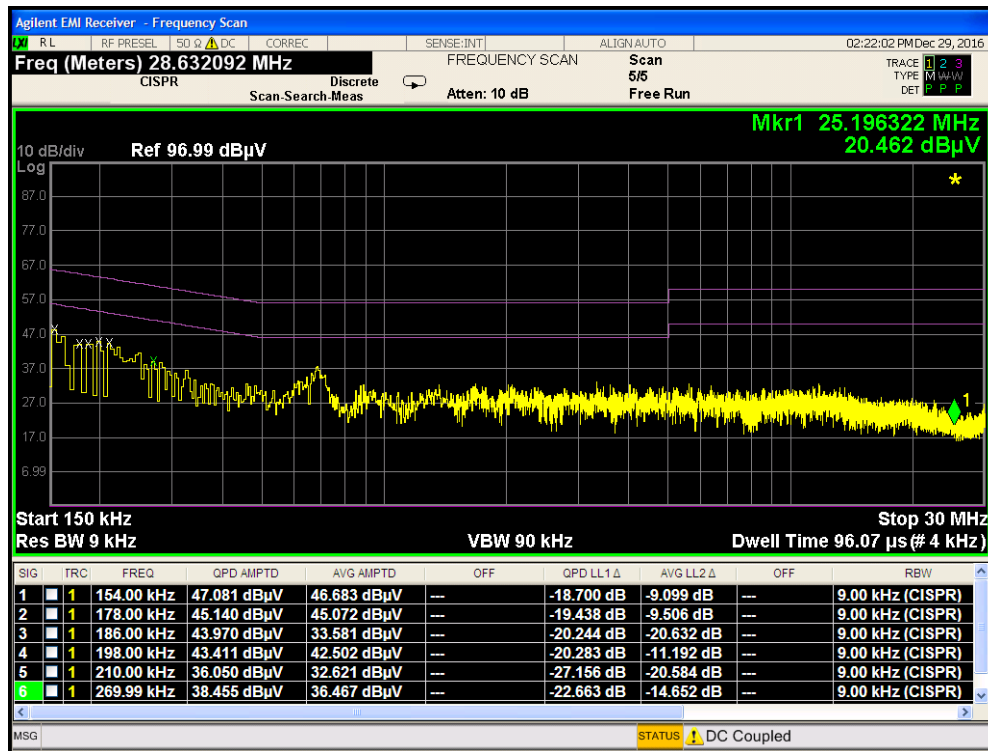
Plot 7-39. Line Conducted Plot with Bluetooth LE (L1)
