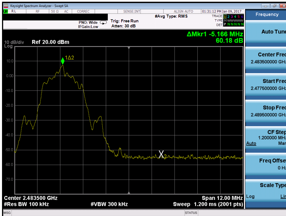
Plot 7-22. Band Edge Plot (Bluetooth (LE), 2Mbps – Ch. 39)
