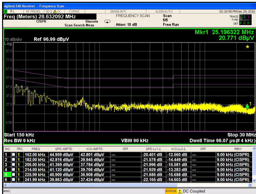
Plot 7-40. Line Conducted Plot with Bluetooth LE (N)
