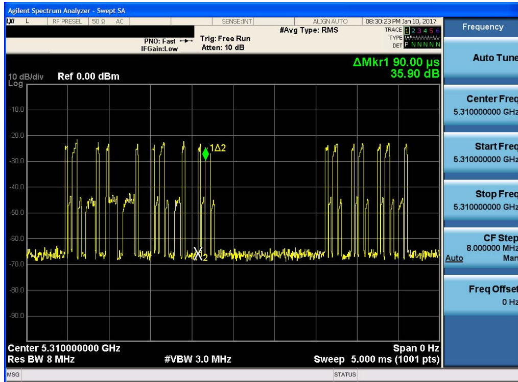
Figure 5-2. Band 2A Period
