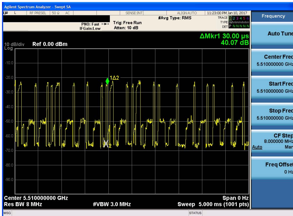
Figure 5-3. Band 2C Pulse Width
