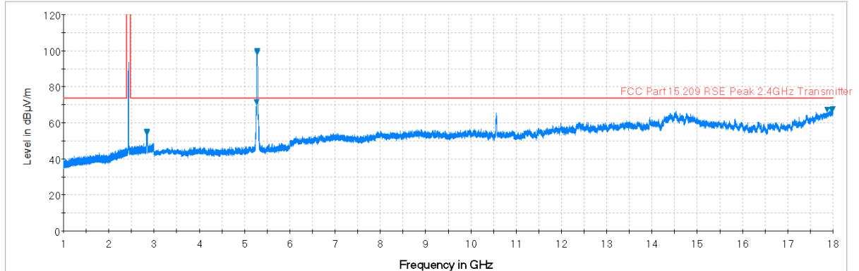
Plot 7-31. Radiated Spurious Plot above 1GHz (5GHz – 2.4 GHz, Ant. Pol. H)
