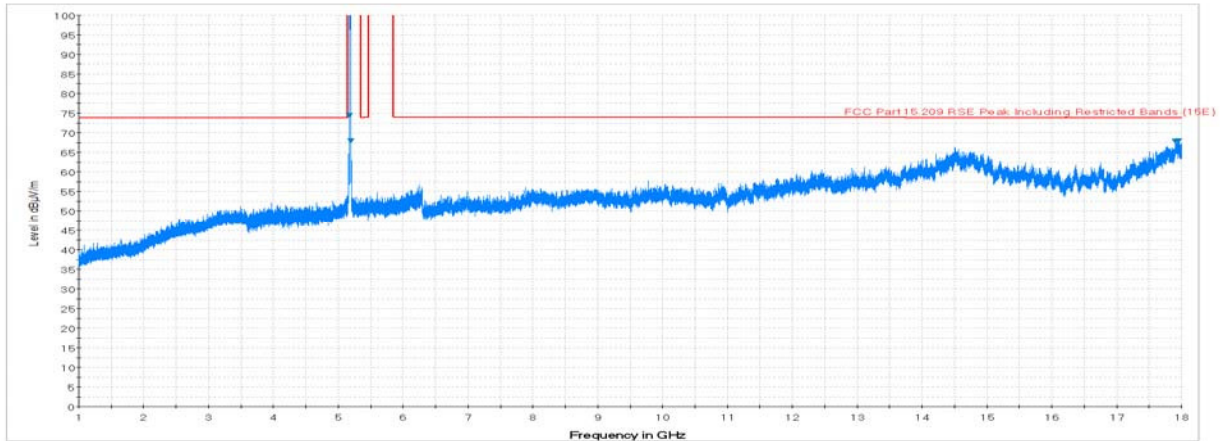
Plot 7-13. Radiated Spurious Plot above 1GHz (802.11a – U1 Ch. 40, Ant. Pol. H)
