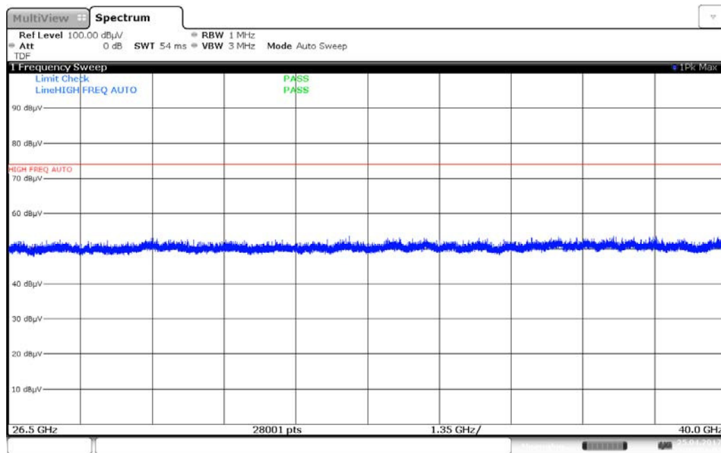
Plot 7-40. Radiated Spurious Plot, 26GHz – 40GHz (2.4GHz – 5GHz, Ant. Pol. H)
