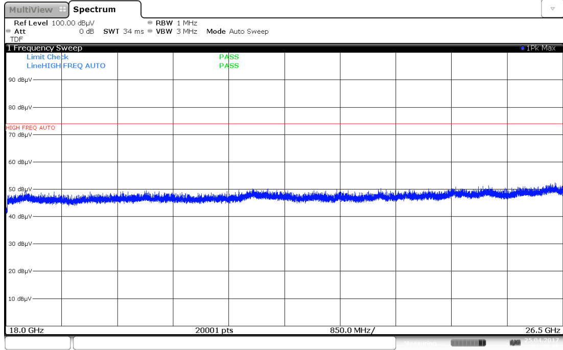
Plot 7-27. Radiated Spurious Plot, 18GHz – 26GHz (2.4GHz – 5GHz, Ant. Pol. H)
