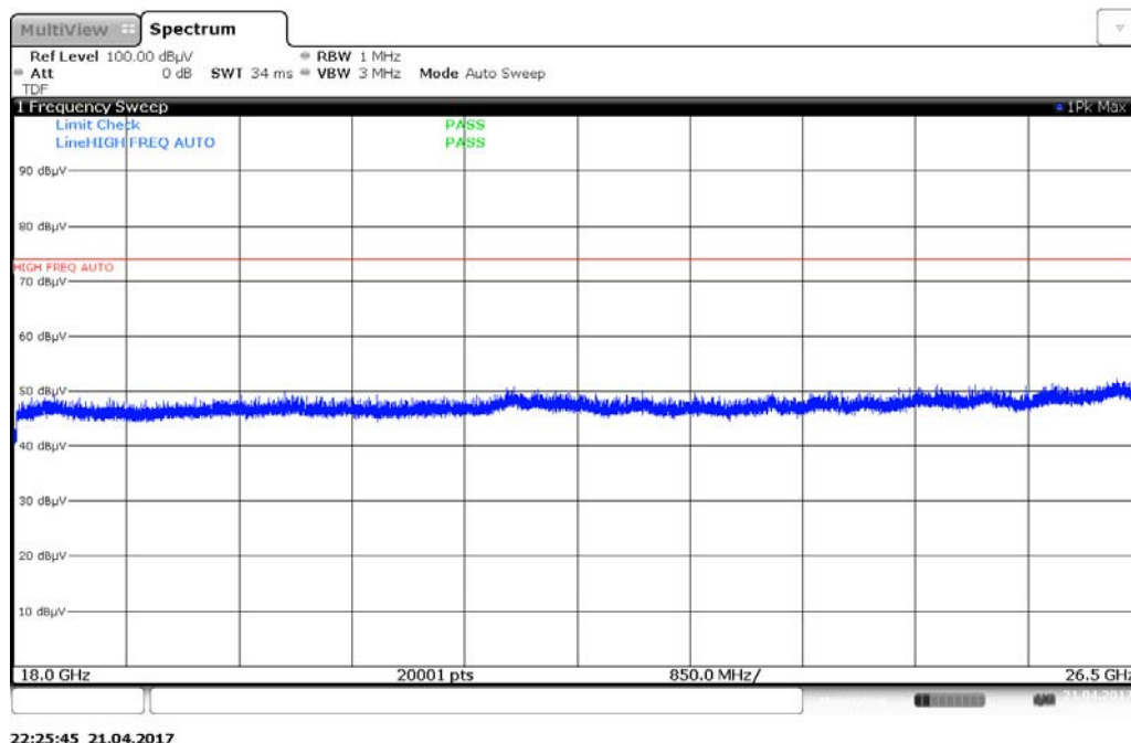
Plot 7-22. Radiated Spurious Plot above 18GHz - 26.5GHz (802.11a – Ant. Pol. V)
