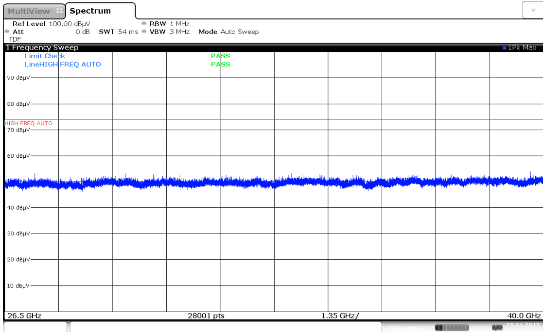
Plot 7-28. Radiated Spurious Plot, 26GHz – 40GHz (2.4GHz – 5GHz, Ant. Pol. H)
