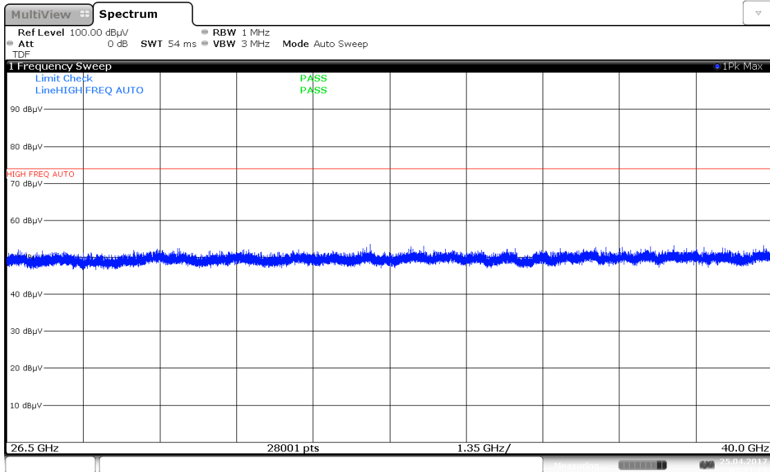
Plot 7-42. Radiated Spurious Plot, 26GHz – 40GHz (2.4GHz – 5GHz, Ant. Pol. V)
