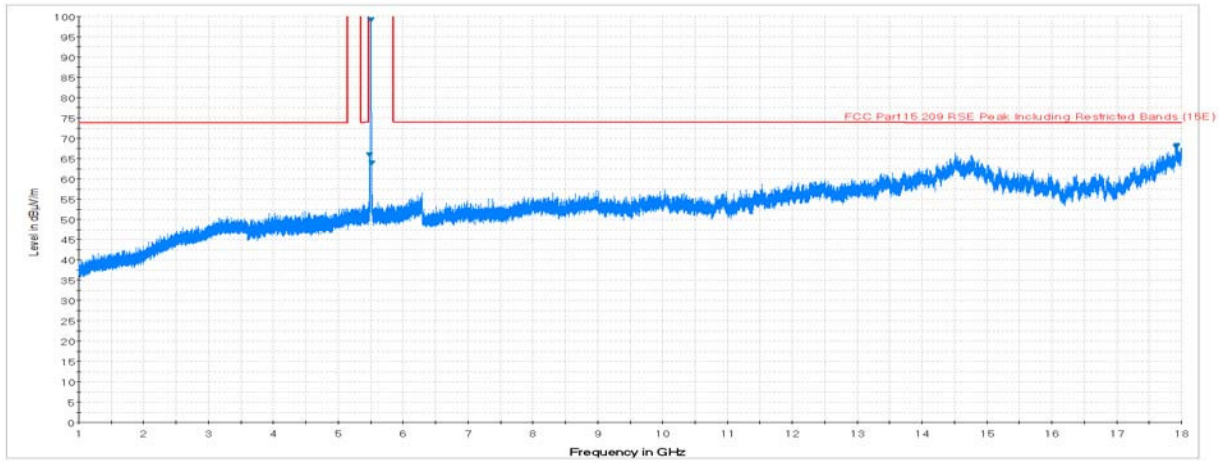
Plot 7-5. Radiated Spurious Plot above 1GHz (802.11a – U2C Ch. 120, Ant. Pol. H)
