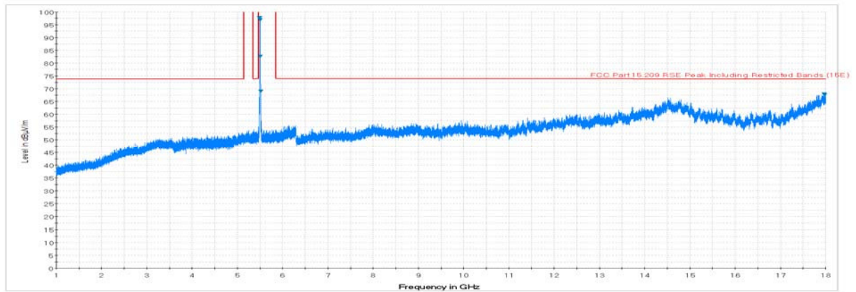
Plot 7-17. Radiated Spurious Plot above 1GHz (802.11a – U2C Ch. 120, Ant. Pol. H)
