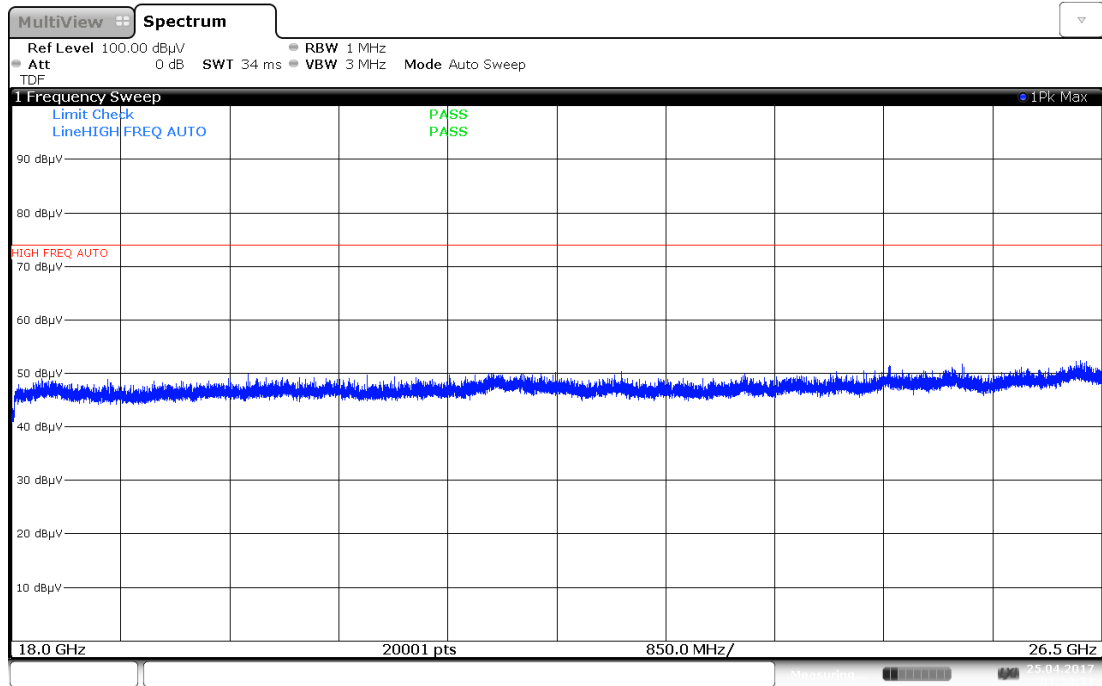
Plot 7-29. Radiated Spurious Plot, 18GHz – 26GHz (2.4GHz – 5GHz, Ant. Pol. V)
