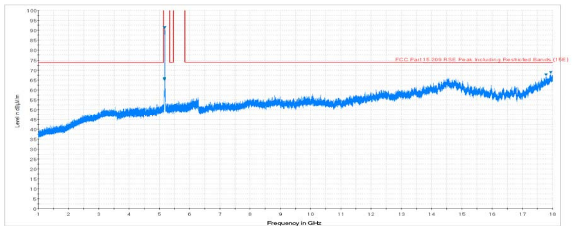
Plot 7-2. Radiated Spurious Plot above 1GHz (802.11a – U1 Ch. 40, Ant. Pol. V)
