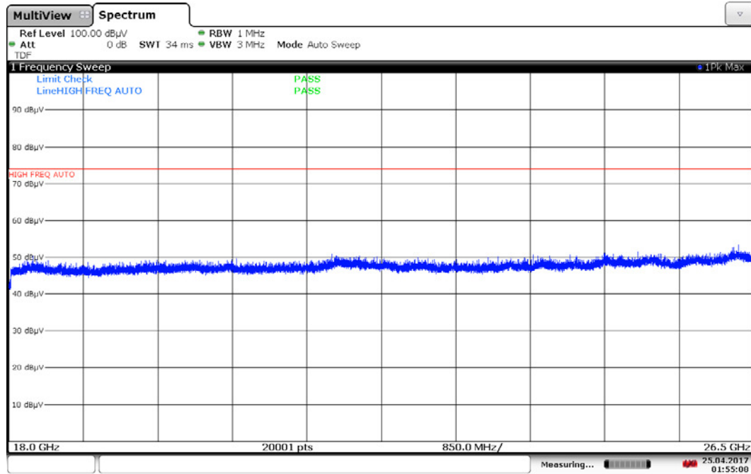
Plot 7-33. Radiated Spurious Plot, 18GHz – 26GHz (2.4GHz – 5GHz, Ant. Pol. H)
