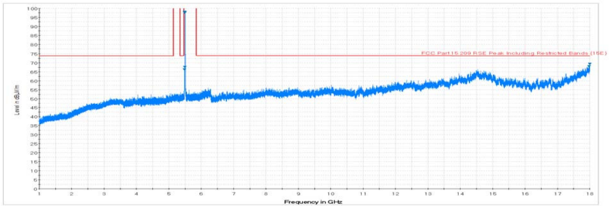
Plot 7-6. Radiated Spurious Plot above 1GHz (802.11a – U2C Ch. 120, Ant. Pol. V)
