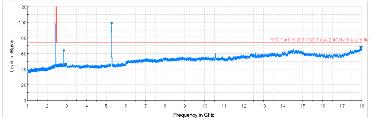
Plot 7-37. Radiated Spurious Plot above 1GHz (Ant1: 2.4 - 5GHz Ant2: 2.4 - 5GHz, Ant. Pol. H)
