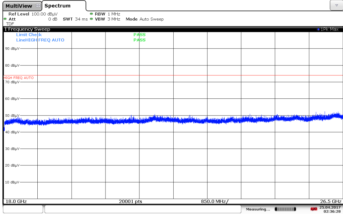
Plot 7-41. Radiated Spurious Plot, 18GHz – 26GHz (2.4GHz – 5GHz, Ant. Pol. V)
