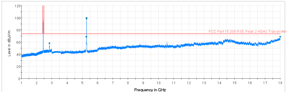
Plot 7-38. Radiated Spurious Plot above 1GHz (Ant1: 2.4 - 5GHz Ant2: 2.4 - 5GHz, Ant. Pol. V)
