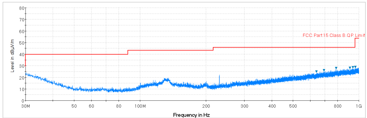
Plot 7-56. Radiated Spurious Plot below 1GHz (802.11a – U3 Ch. 157, Ant. Pol. H)
