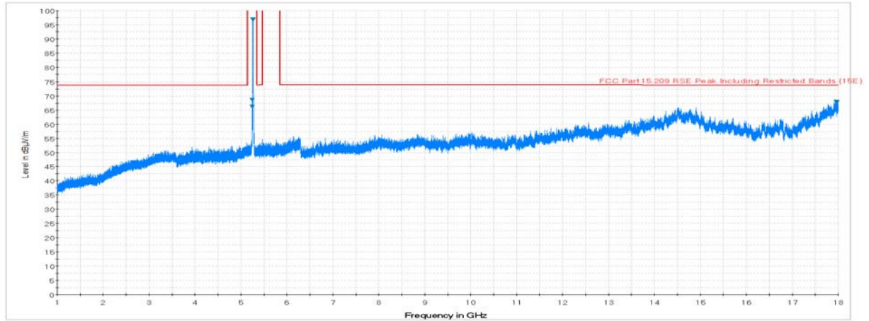
Plot 7-16. Radiated Spurious Plot above 1GHz (802.11a – U2A Ch. 56, Ant. Pol. V)
