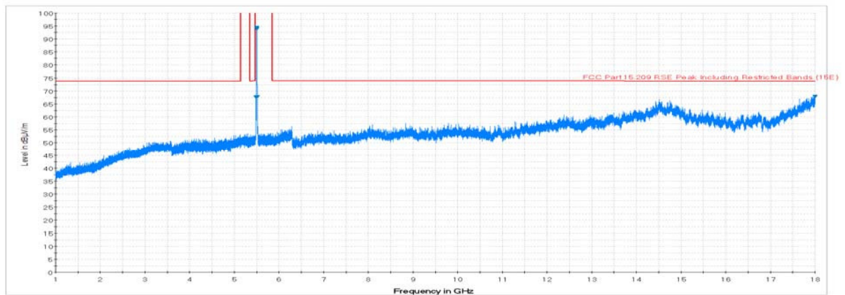
Plot 7-18. Radiated Spurious Plot above 1GHz (802.11a – U2C Ch. 120, Ant. Pol. V)
