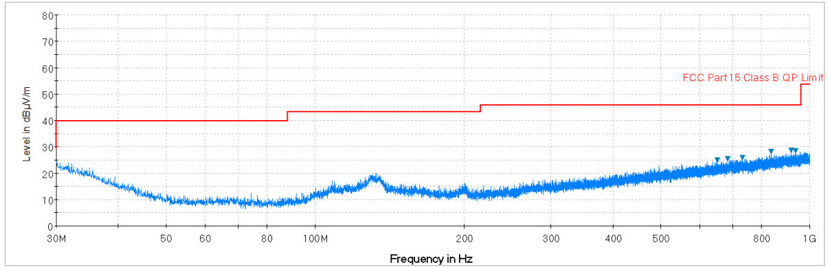
Plot 7-54. Radiated Spurious Plot below 1GHz (802.11a – U3 Ch. 157, Ant. Pol. H)
