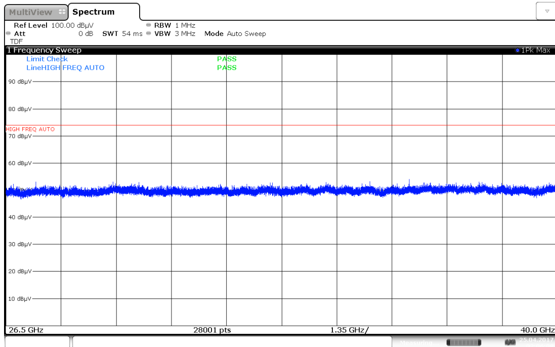
Plot 7-36. Radiated Spurious Plot, 26GHz – 40GHz (2.4GHz – 5GHz, Ant. Pol. V)
