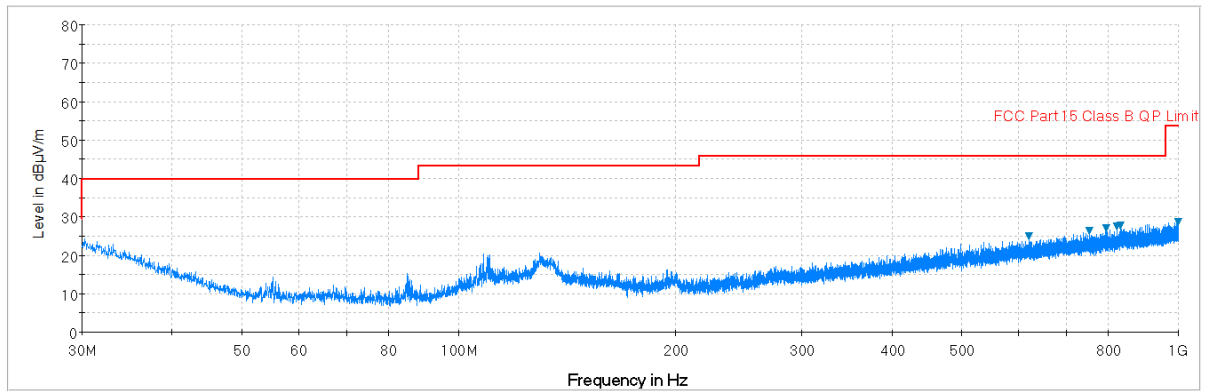
Plot 7-55. Radiated Spurious Plot below 1GHz (802.11a – U3 Ch. 157, Ant. Pol. V)
