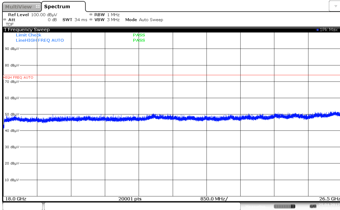
Plot 7-39. Radiated Spurious Plot, 18GHz – 26GHz (2.4GHz – 5GHz, Ant. Pol. H)
