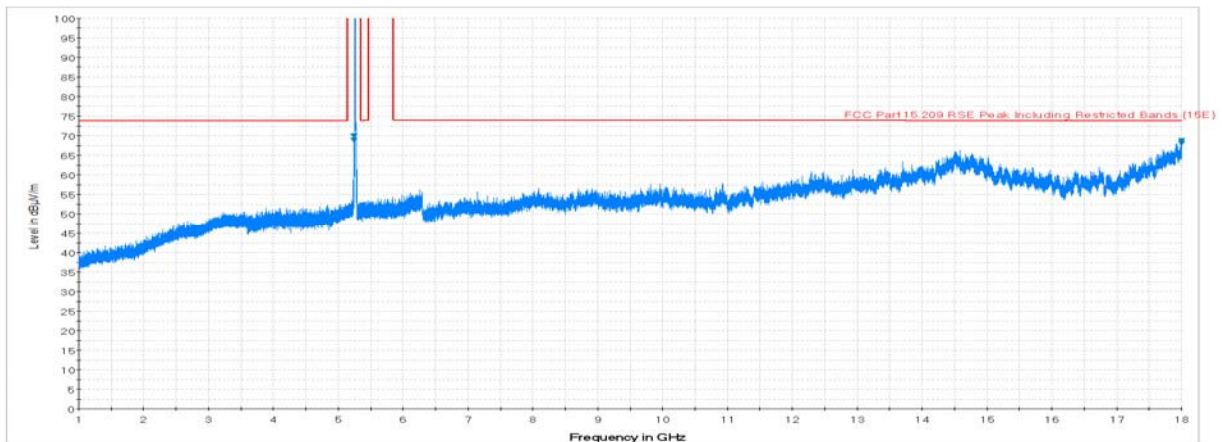
Plot 7-15. Radiated Spurious Plot above 1GHz (802.11a – U2A Ch. 56, Ant. Pol. H)
