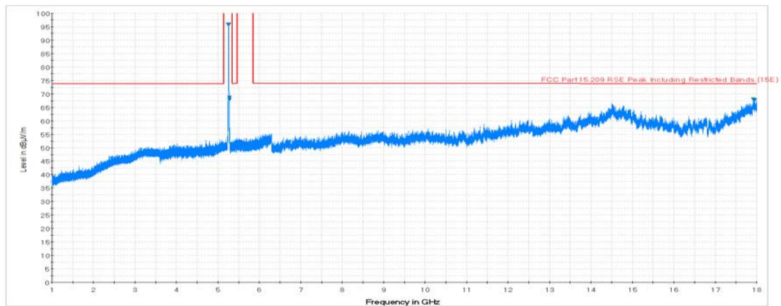
Plot 7-3. Radiated Spurious Plot above 1GHz (802.11a – U2A Ch. 56, Ant. Pol. H)
