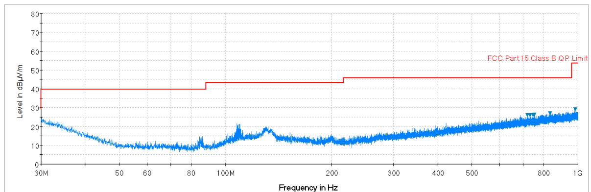
Plot 7-57. Radiated Spurious Plot below 1GHz (802.11a – U3 Ch. 157, Ant. Pol. V)
