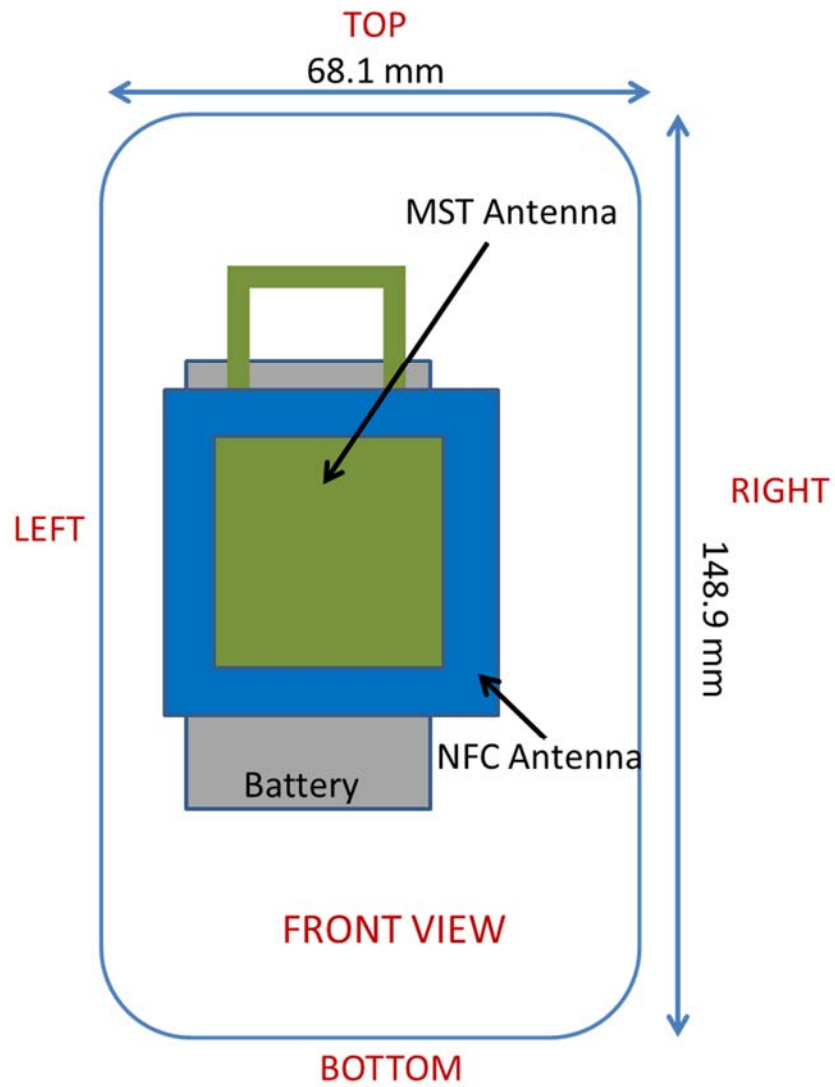
Figure F-2 NFC and MST Antenna Locations
