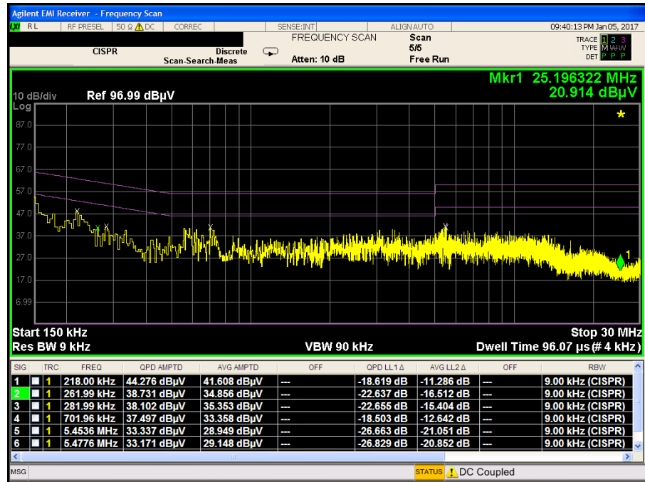
Plot 7-56. Line-Conducted Test Plot (L1)
