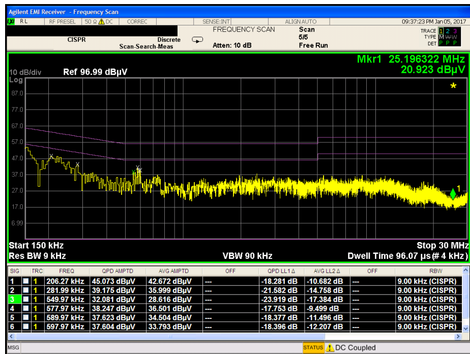
Plot 7-57. Line-Conducted Test Plot (N)
