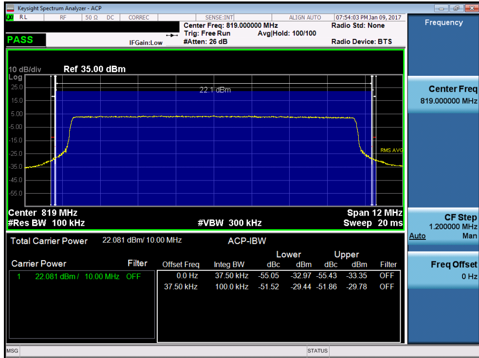
Plot 7-35. Channel Edge Plot (10MHz QPSK – RB Size 50)
