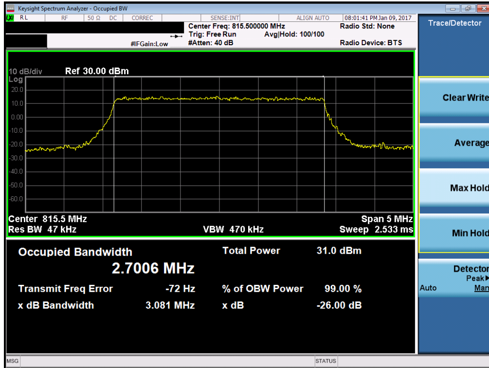
Plot 7-7. Occupied Bandwidth Plot (3MHz QPSK – RB Size 15– Low Channel)
