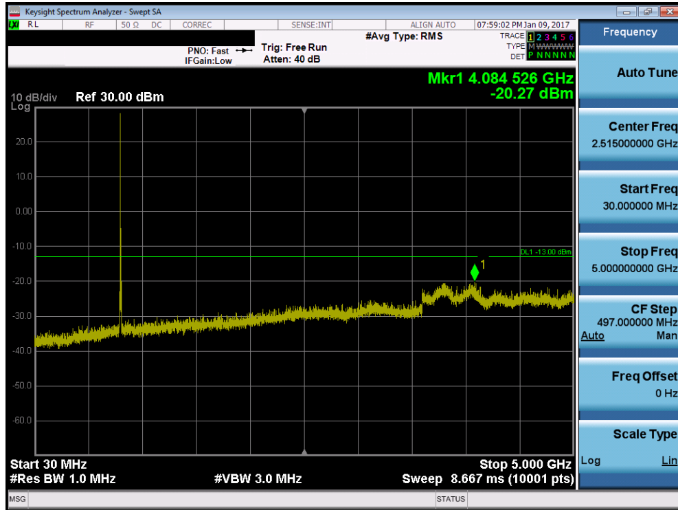
Plot 7-27. Conducted Spurious Plot (5MHz QPSK – RB Size 1, RB Offset 0 – High Channel)
