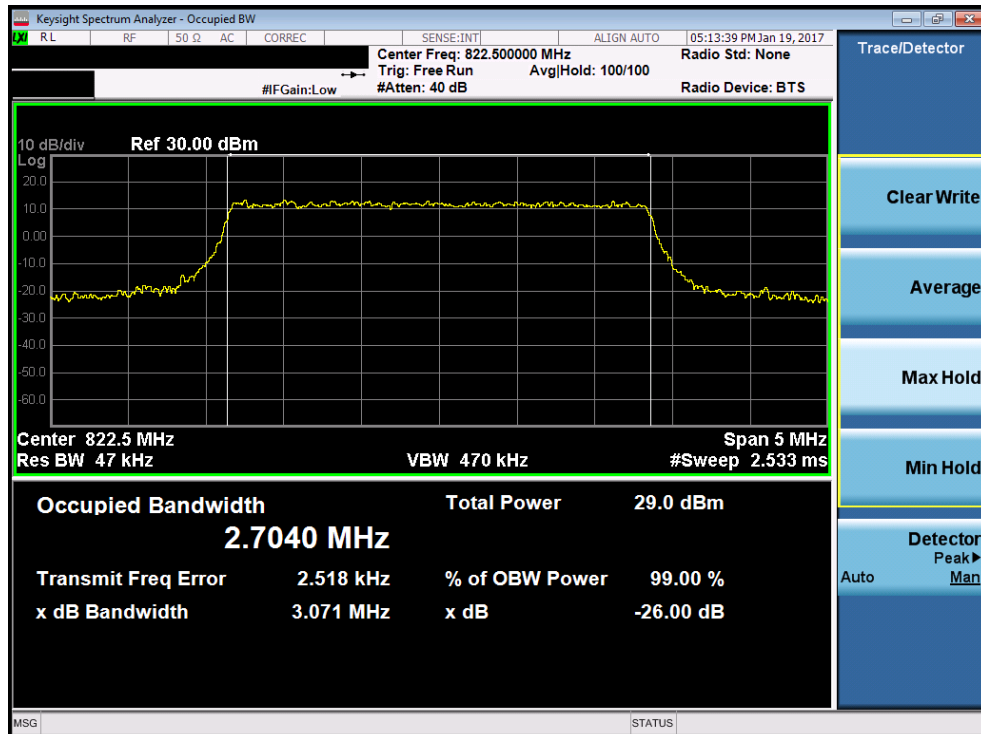
Plot 7-12. Occupied Bandwidth Plot (3MHz 64-QAM – RB Size 15– High Channel)
