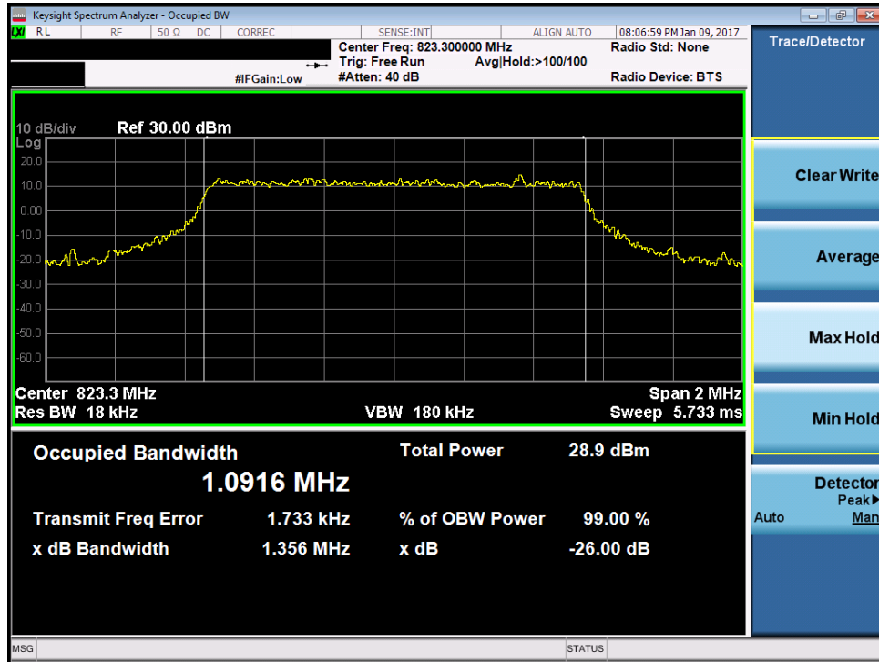
Plot 7-5. Occupied Bandwidth Plot (1.4MHz 16-QAM – RB Size 6– High Channel)
