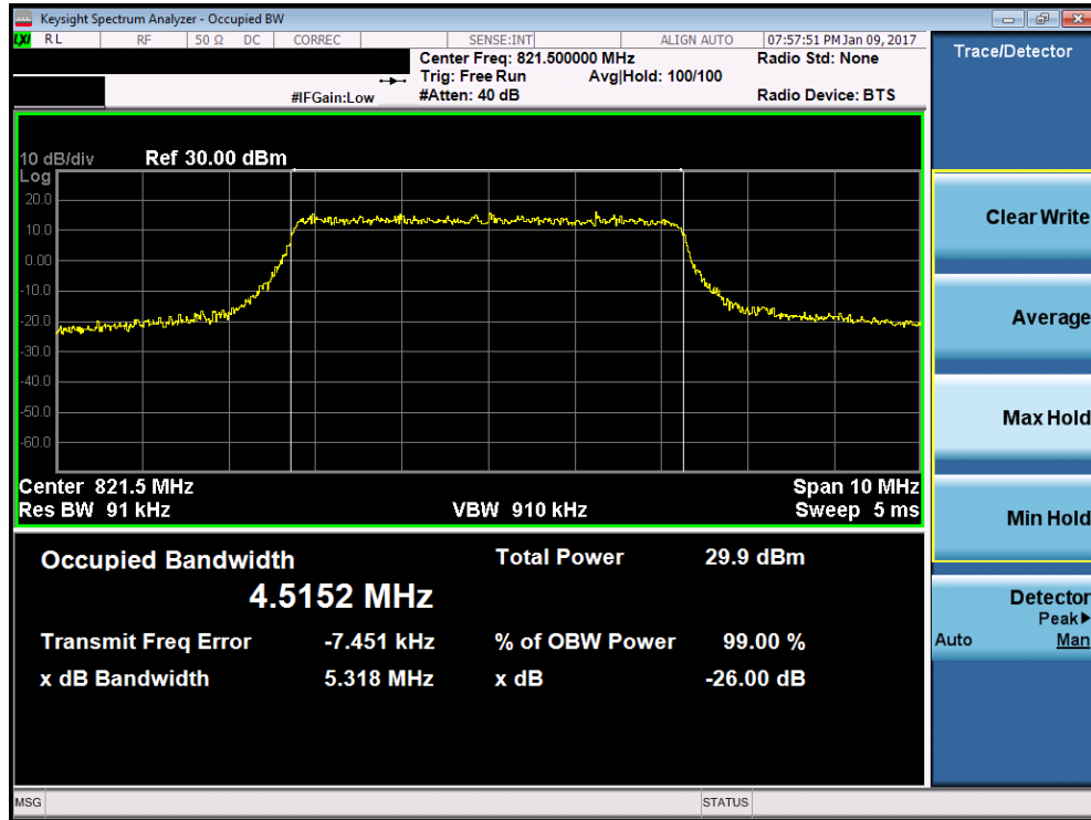
Plot 7-17. Occupied Bandwidth Plot (5MHz 16-QAM – RB Size 25– High Channel)
