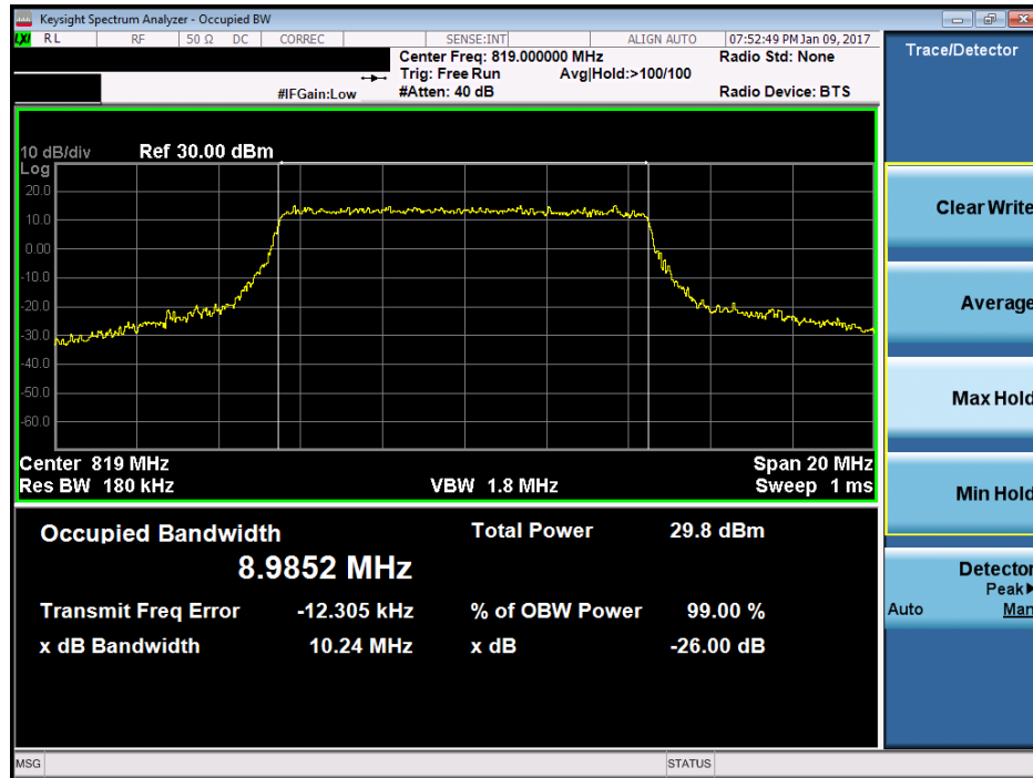
Plot 7-20. Occupied Bandwidth Plot (10MHz 16-QAM – RB Size 50)
