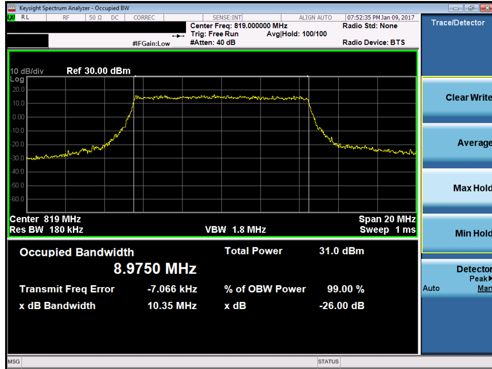
Plot 7-19. Occupied Bandwidth Plot (10MHz QPSK – RB Size 50)
