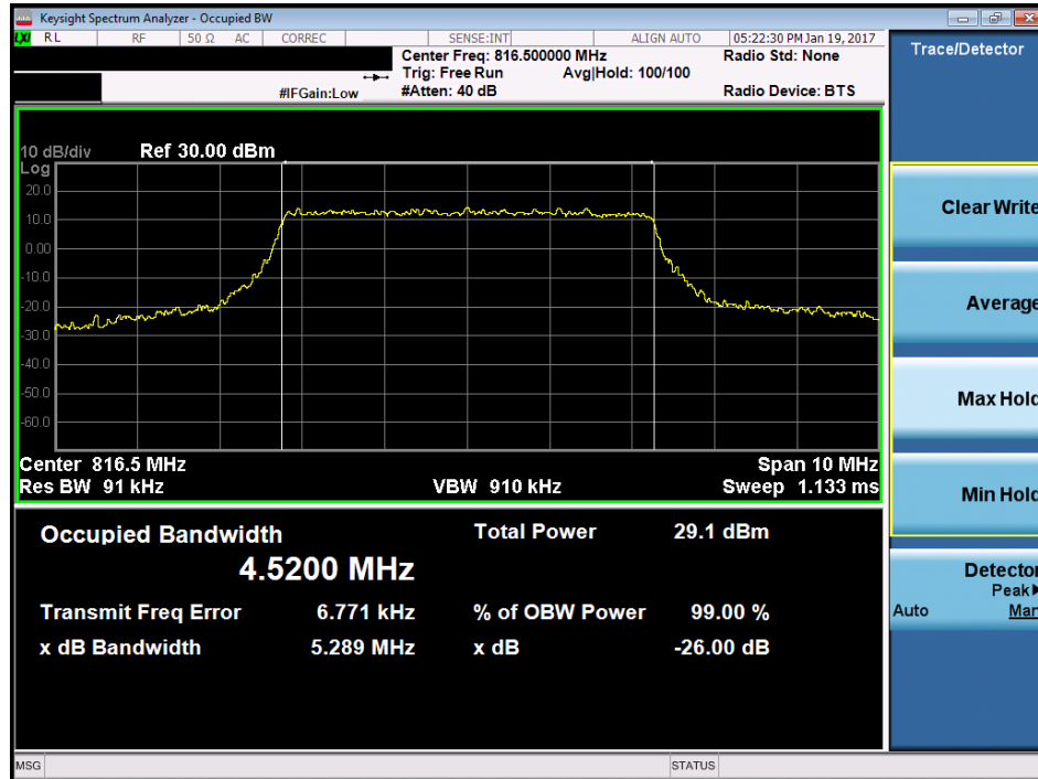
Plot 7-15. Occupied Bandwidth Plot (5MHz 64-QAM – RB Size 25– Low Channel)
