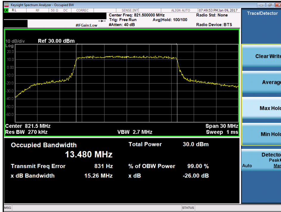
Plot 7-23. Occupied Bandwidth Plot (15MHz 16-QAM – RB Size 75)
