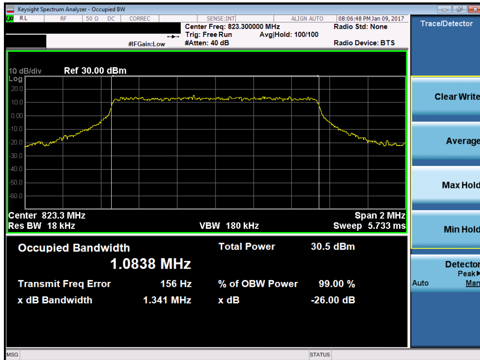
Plot 7-4. Occupied Bandwidth Plot (1.4MHz QPSK – RB Size 6– High Channel)
