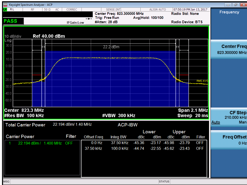
Plot 7-30. Channel Edge Plot (1.4MHz QPSK – RB Size 6 – High Channel)
