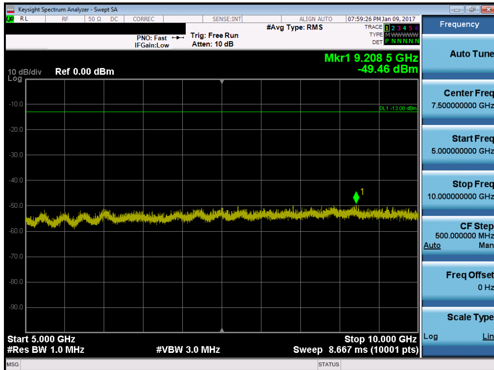
Plot 7-28. Conducted Spurious Plot (5MHz QPSK – RB Size 1, RB Offset 0 – High Channel)
