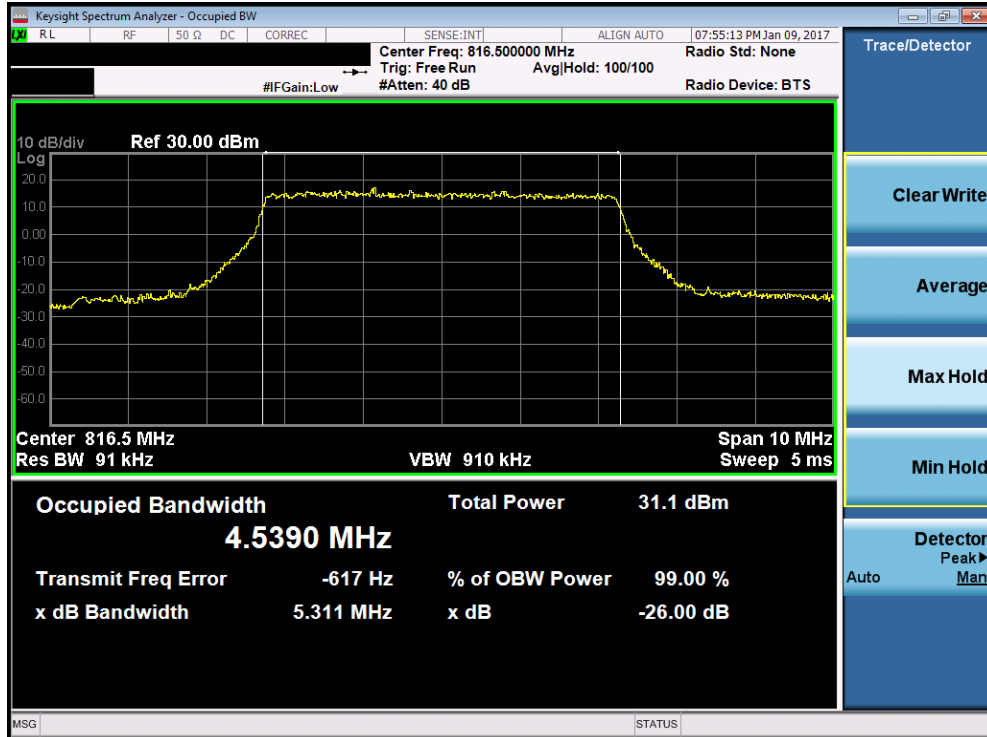
Plot 7-13. Occupied Bandwidth Plot (5MHz QPSK – RB Size 25– Low Channel)
