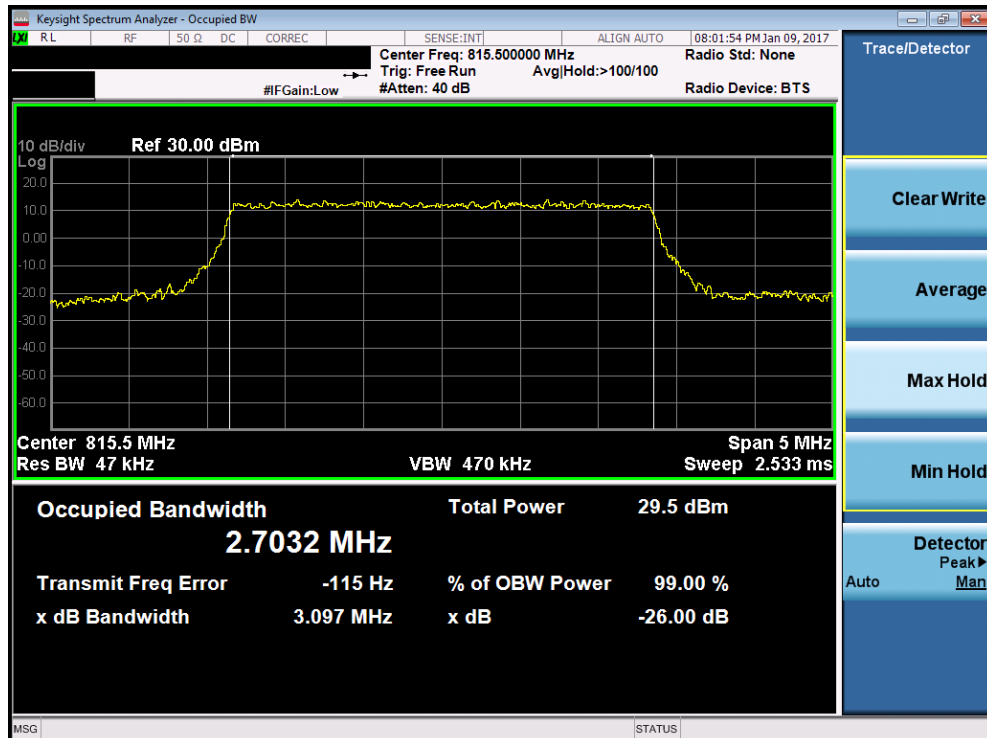
Plot 7-8. Occupied Bandwidth Plot (3MHz 16-QAM – RB Size 15– Low Channel)
