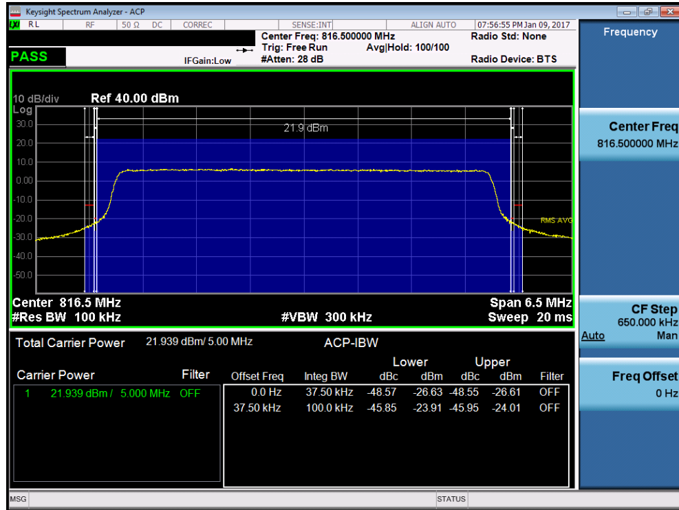
Plot 7-33. Channel Edge Plot (5MHz QPSK – RB Size 25– Low Channel)
