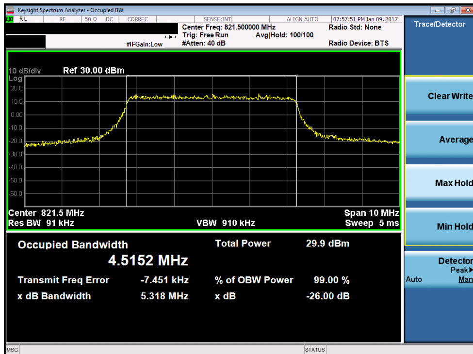
Plot 7-14. Occupied Bandwidth Plot (5MHz 16-QAM – RB Size 25– Low Channel)
