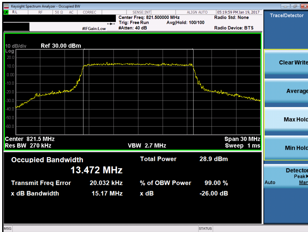
Plot 7-24. Occupied Bandwidth Plot (15MHz 64-QAM – RB Size 75)
