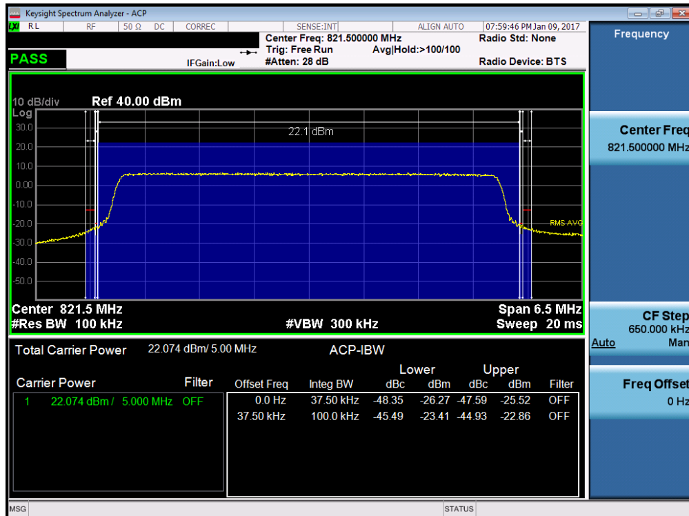
Plot 7-34. Channel Edge Plot (5MHz QPSK – RB Size 25 – High Channel)
