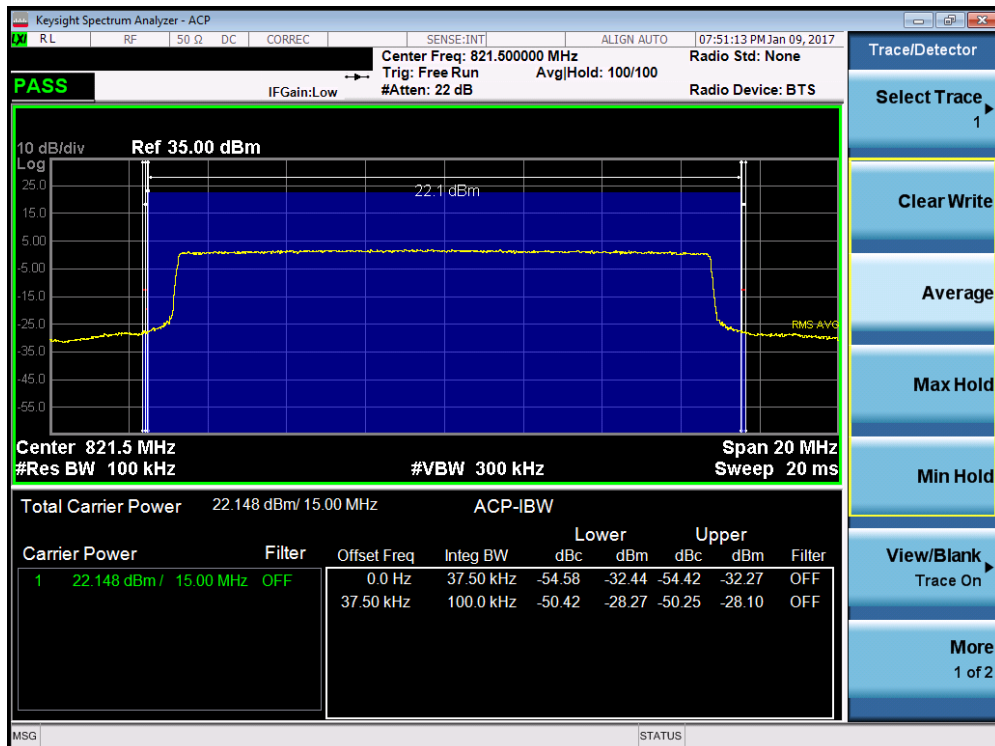
Plot 7-36. Channel Edge Plot (15MHz QPSK – RB Size 75)
