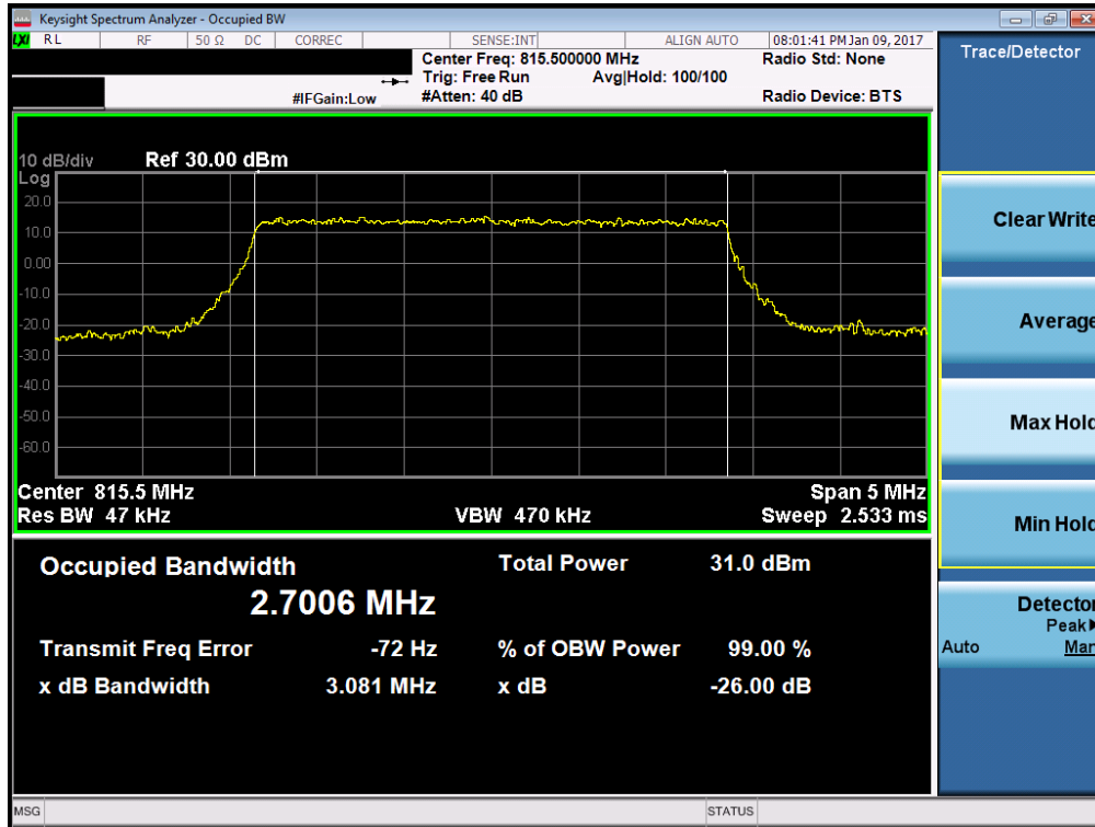
Plot 7-9. Occupied Bandwidth Plot (3MHz 64-QAM – RB Size 15– Low Channel)
