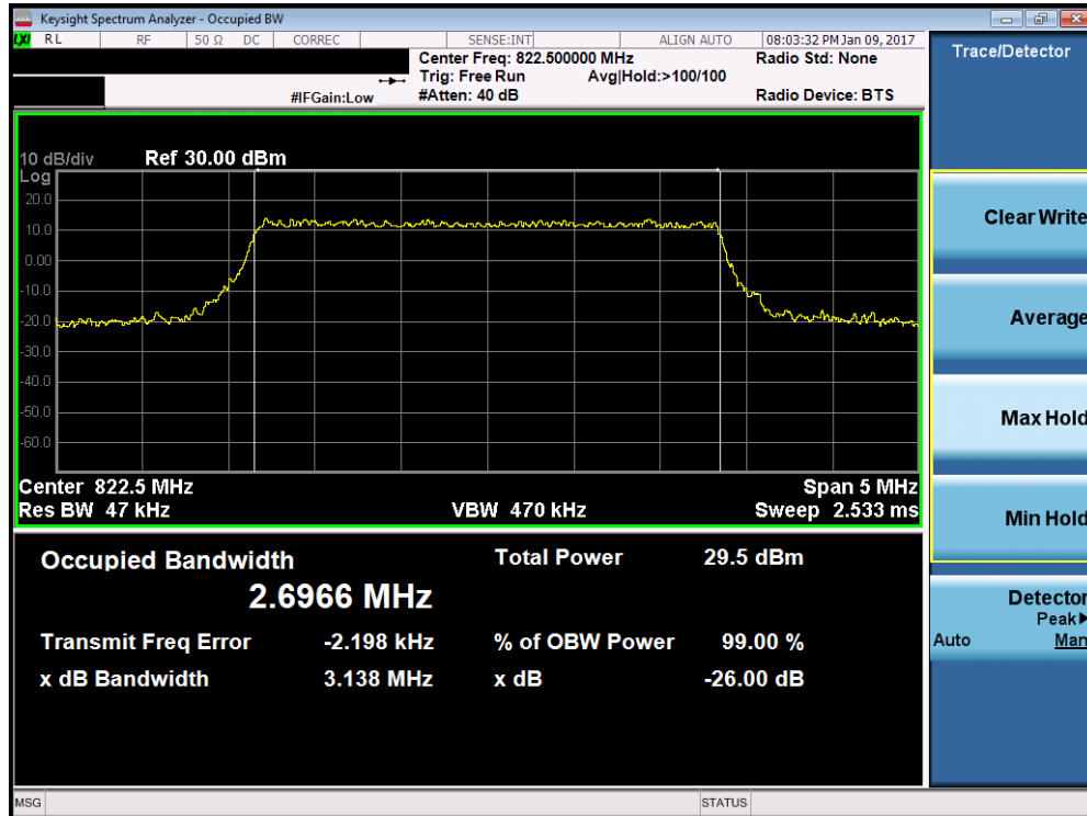
Plot 7-11. Occupied Bandwidth Plot (3MHz 16-QAM – RB Size 15– High Channel)
