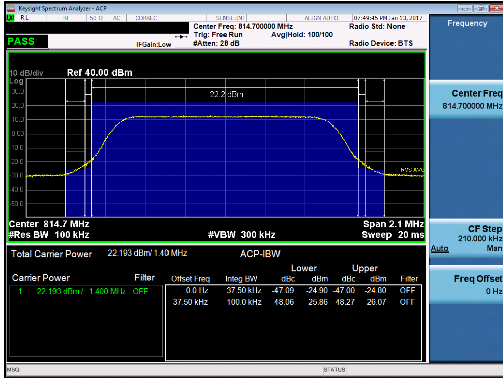
Plot 7-29. Channel Edge Plot (1.4MHz QPSK – RB Size 6– Low Channel)
