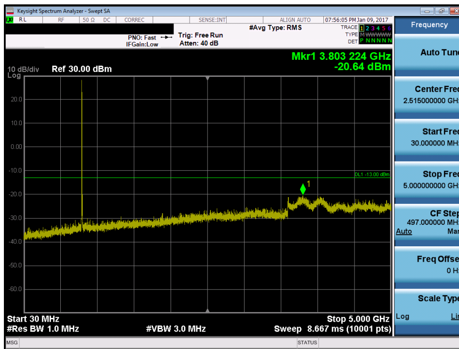
Plot 7-25. Conducted Spurious Plot (5MHz QPSK – RB Size 1, RB Offset 0 – Low Channel)
