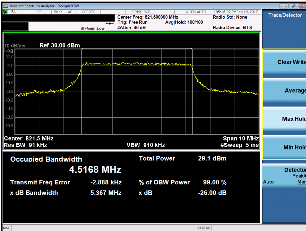
Plot 7-18. Occupied Bandwidth Plot (5MHz 64-QAM – RB Size 25– High Channel)
