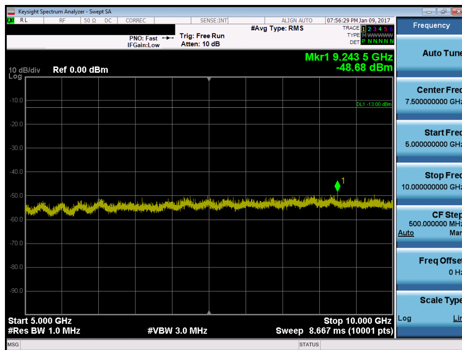
Plot 7-26. Conducted Spurious Plot ( 5MHz QPSK – RB Size 1, RB Offset 0 – Low Channel)
