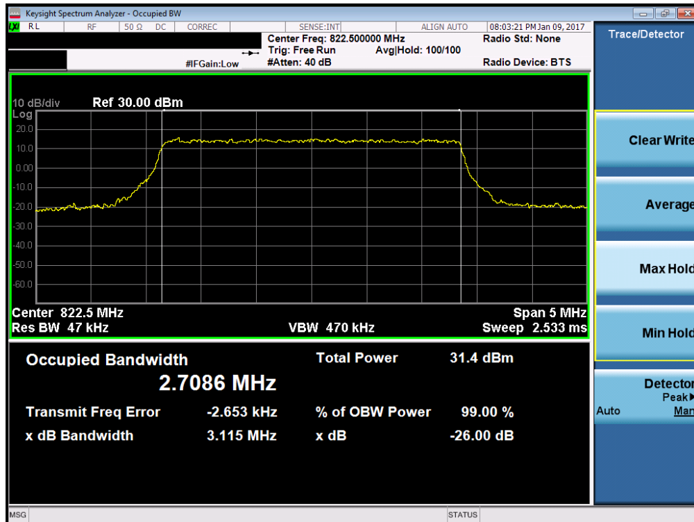
Plot 7-10. Occupied Bandwidth Plot (3MHz QPSK – RB Size 15– High Channel)
