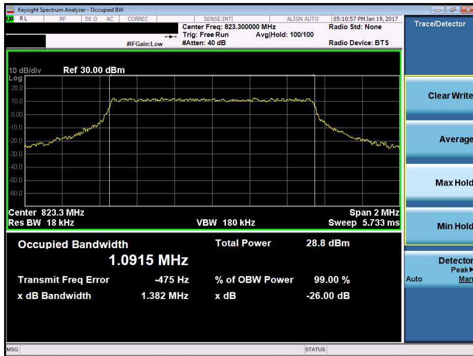
Plot 7-6. Occupied Bandwidth Plot (1.4MHz 64-QAM – RB Size 6– High Channel)
