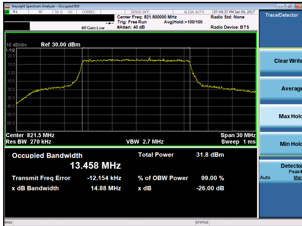
Plot 7-22. Occupied Bandwidth Plot (15MHz QPSK – RB Size 75)
