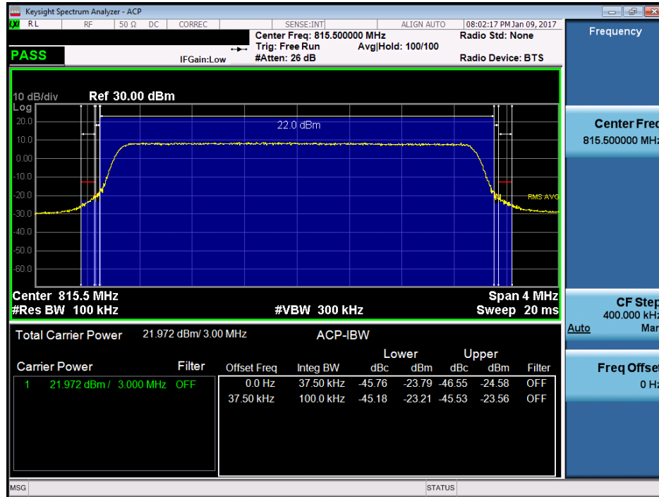
Plot 7-31. Channel Edge Plot (3MHz QPSK – RB Size 15– Low Channel)
