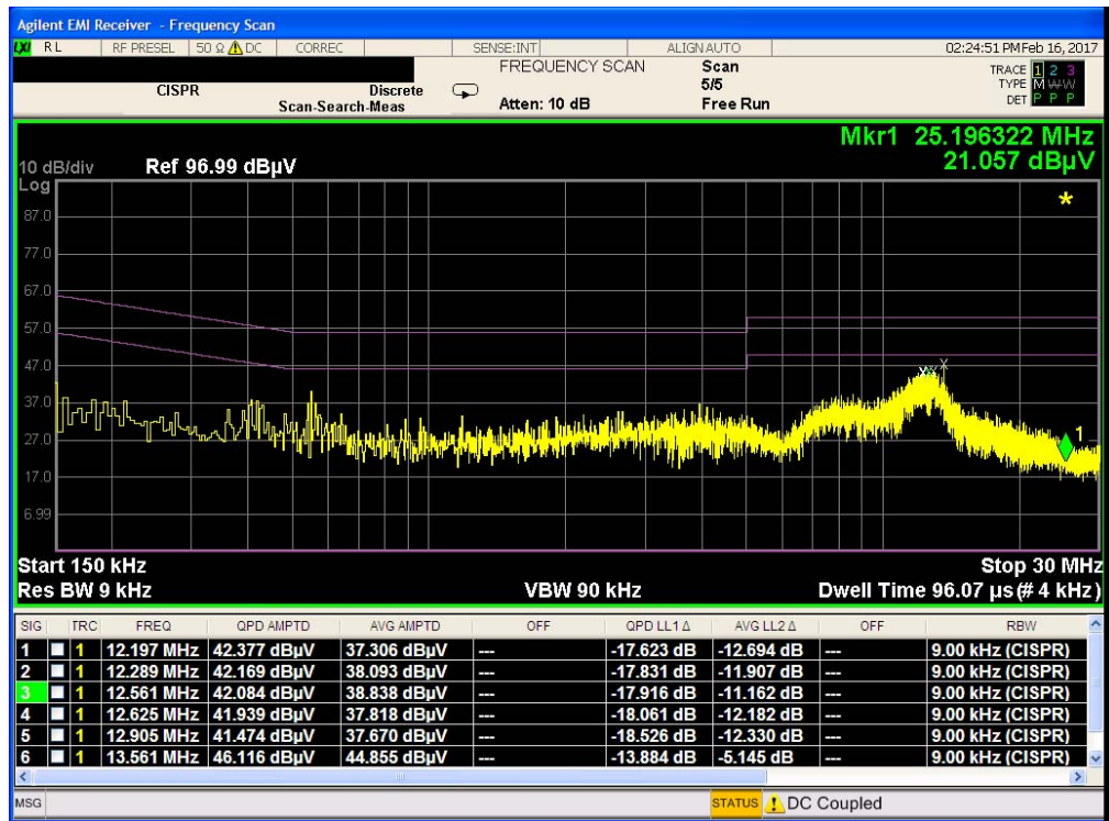
Plot 8-3. Line-Conducted Test Plot (L1)
