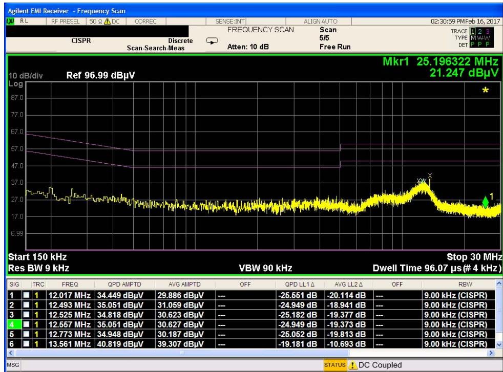
Plot 8-4. Line-Conducted Test Plot (N)
