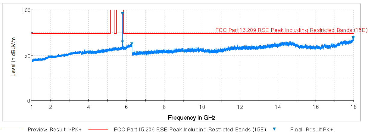
Plot 7-163. Radiated Spurious Plot above 1GHz (802.11a – U3 Ch. 157, Ant. Pol. H)
