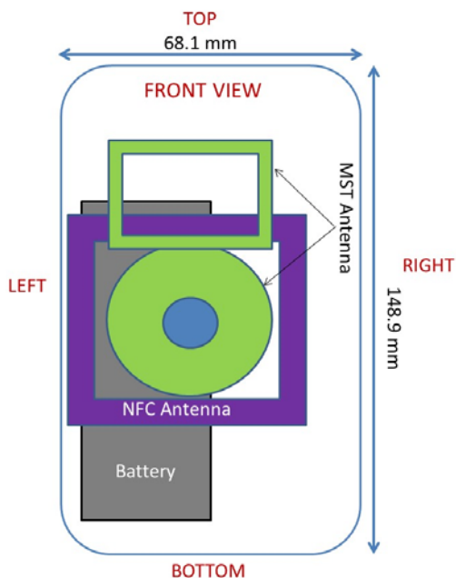
Figure F-2 MST and NFC Antenna Locations
