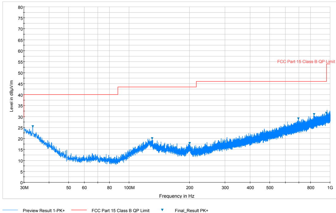
Plot 7-13. Radiated Spurious Plot below 1GHz (Pol. H)
