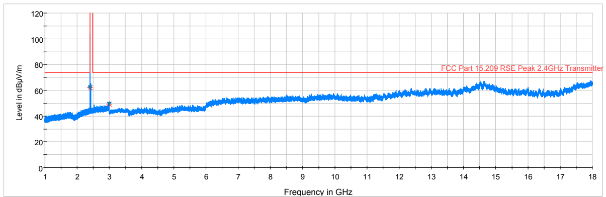
Plot 7-2. Radiated Spurious Plot above 1GHz (BT – Ch. 0, Ant. Pol. V)
