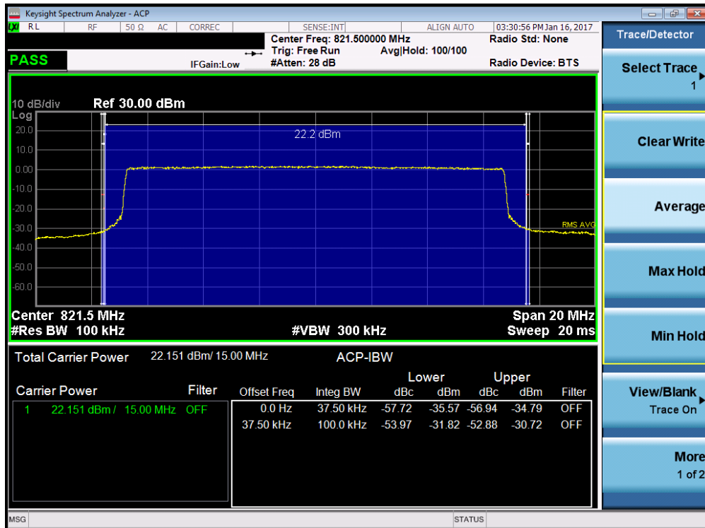
Plot 7-20. Channel Edge Plot (15MHz QPSK – RB Size 75)
