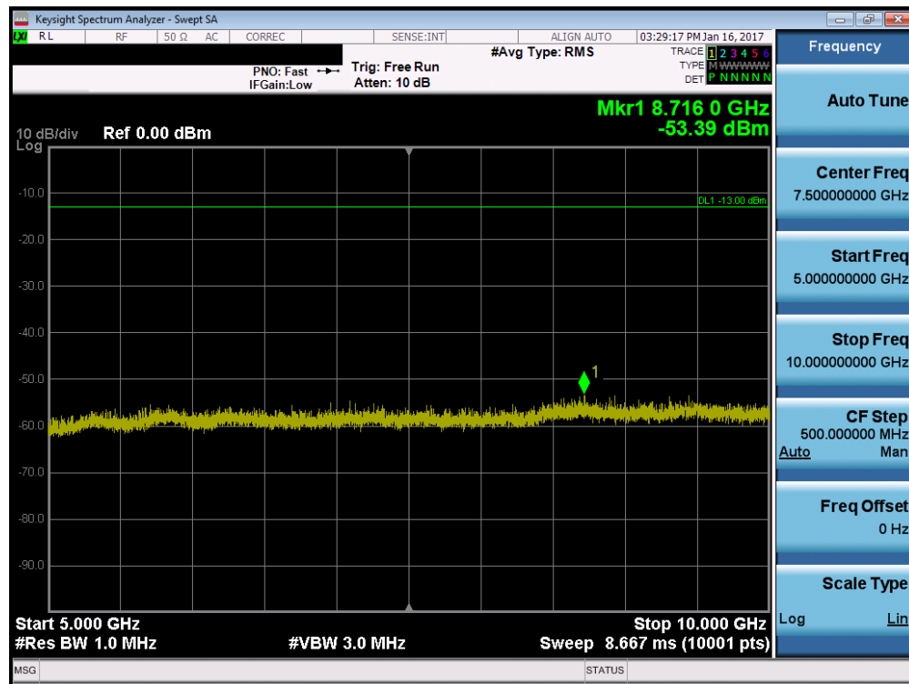
Plot 7-12. Conducted Spurious Plot (10MHz QPSK – RB Size 1, RB Offset 0)
