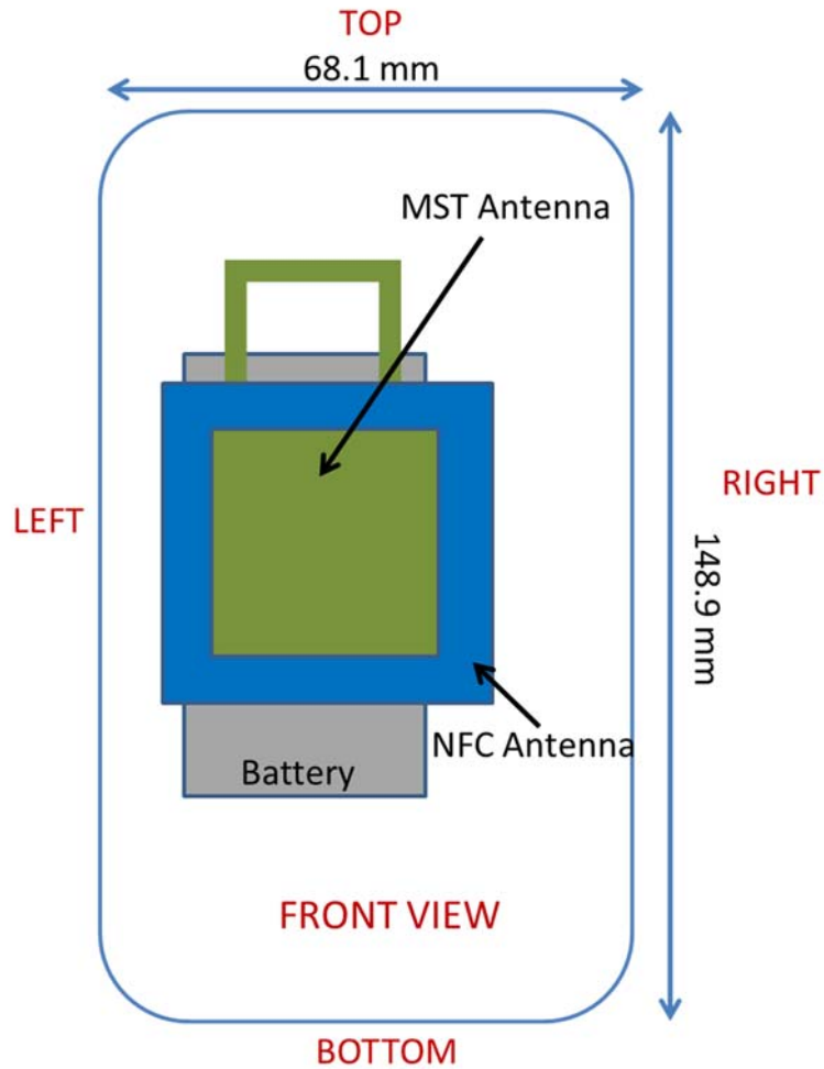
Figure F-2 MST and NFC Antenna Locations
