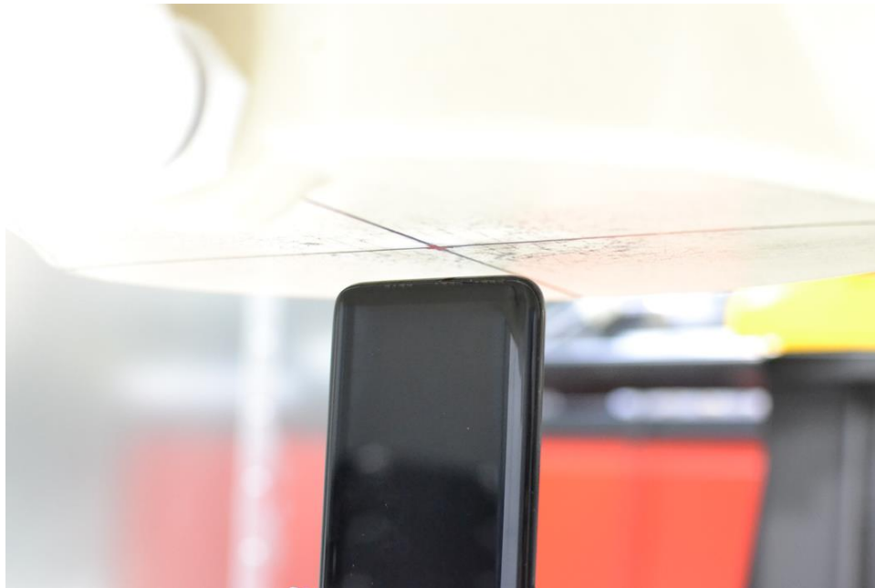
SAR Test Setup Photo 9 – Bottom Edge at 1.0 cm
