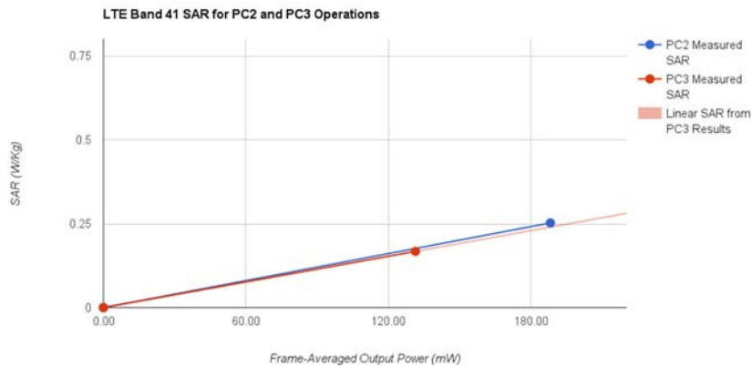
Figure 14-A LTE Band 41 Linearity
