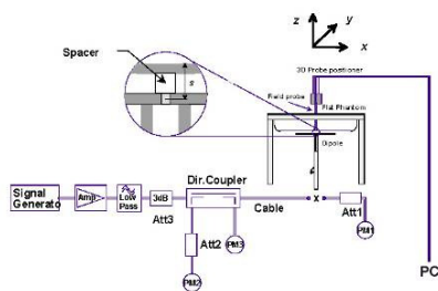
Figure 10-A System Verification Setup Diagram
