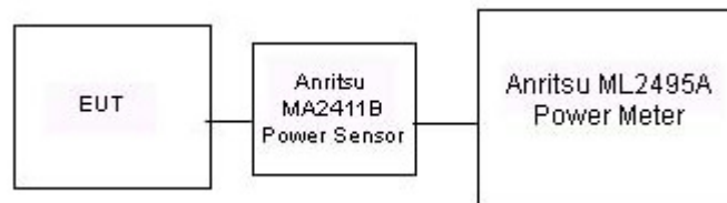
Figure 9-F Power Measurement Setup
