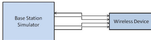
Figure G-2 Power Measurement Setup
