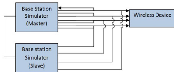
Figure G-3 Power Measurement Setup
