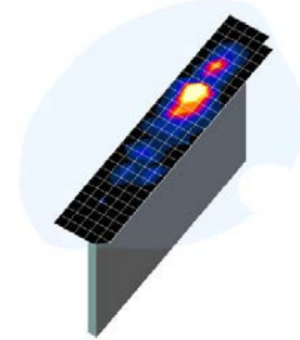
Figure 3-A Sample SAR Area Scan
