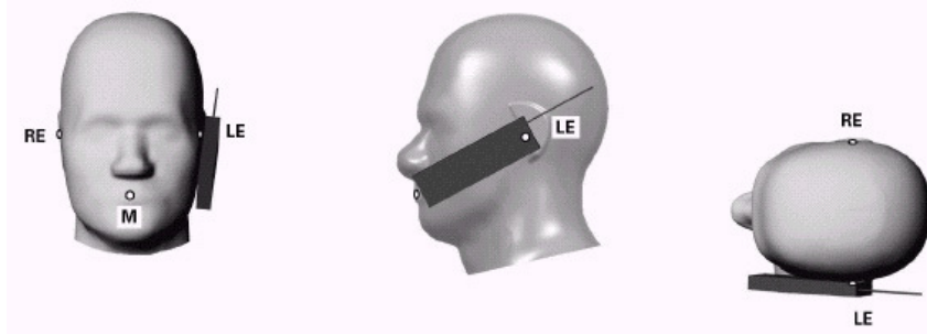
Figure 5-A Front, Side and Top View of Cheek Position
