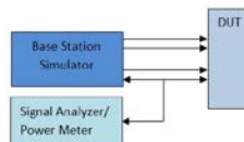
Figure 4-1 Power Measurement Setup
