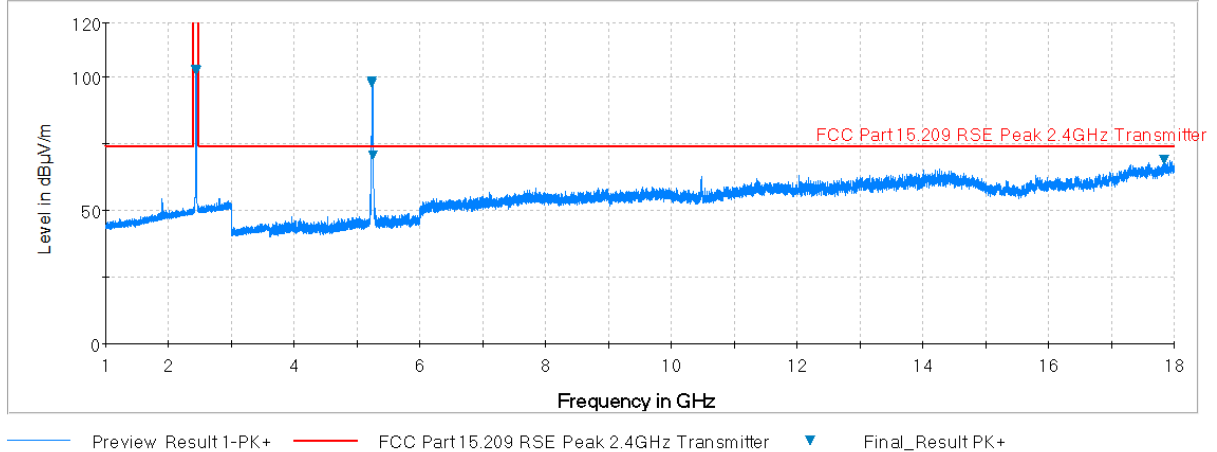
Plot 7-29. Radiated Spurious Plot above 1GHz (Ant1: 2.4 - 5GHz Ant2: 2.4 - 5GHz, Ant. Pol. H)
