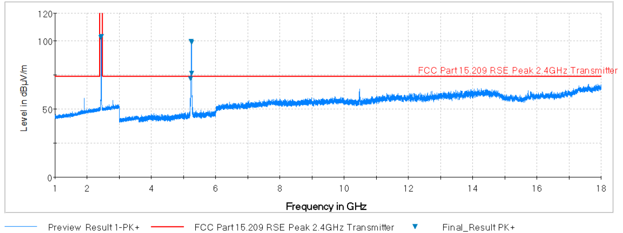
Plot 7-27. Radiated Spurious Plot above 1GHz (5GHz – 2.4 GHz, Ant. Pol. H)
