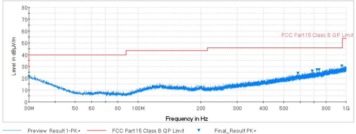
Plot 7-37. Radiated Spurious Plot below 1GHz (802.11a – U3 Ch. 157, Ant. Pol. H)
