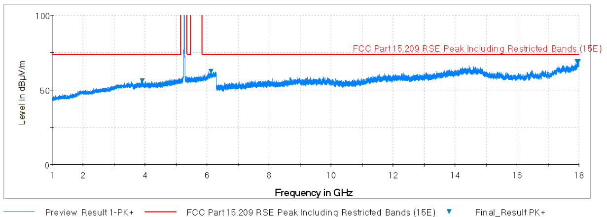
Plot 7-15. Radiated Spurious Plot above 1GHz (802.11a – U2A Ch. 56, Ant. Pol. H)
