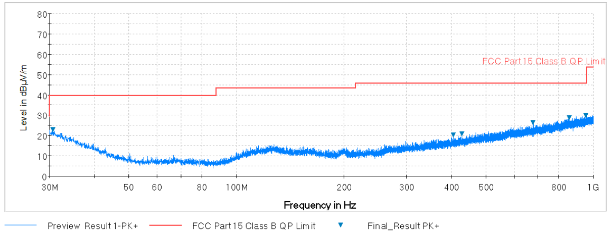
Plot 7-40. Radiated Spurious Plot below 1GHz (802.11a – U3 Ch. 157, Ant. Pol. V)
