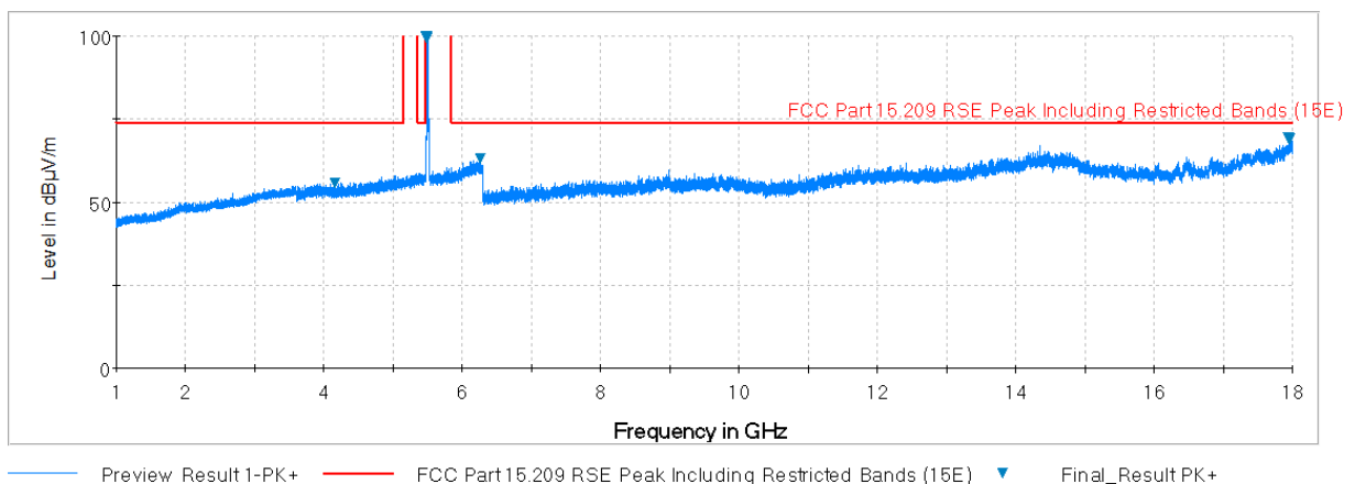
Plot 7-18. Radiated Spurious Plot above 1GHz (802.11a – U2C Ch. 116, Ant. Pol. V)
