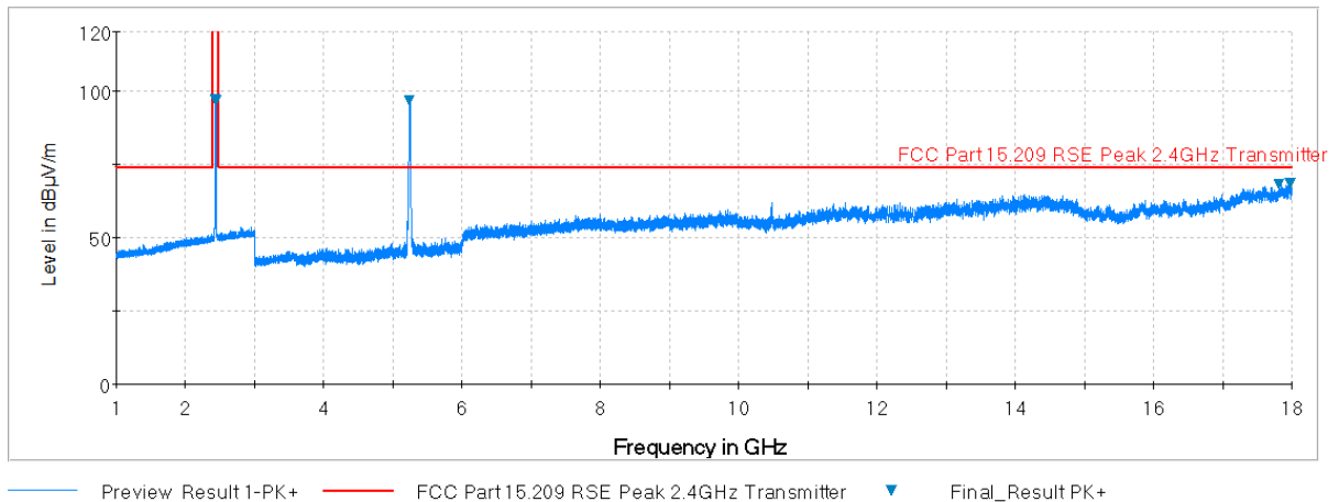
Plot 7-30. Radiated Spurious Plot above 1GHz (Ant1: 2.4 - 5GHz Ant2: 2.4 - 5GHz, Ant. Pol. V)
