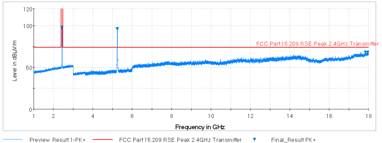
Plot 7-28. Radiated Spurious Plot above 1GHz (5GHz – 2.4 GHz, Ant. Pol. V)
