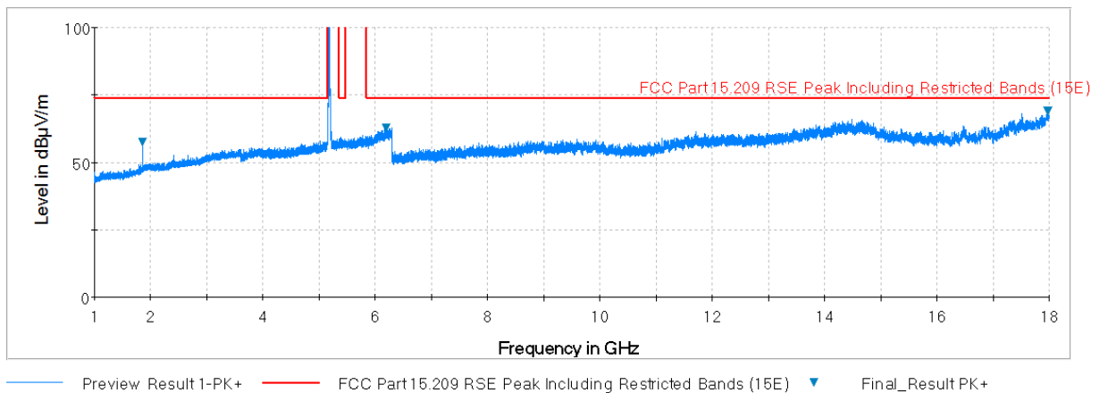
Plot 7-14. Radiated Spurious Plot above 1GHz (802.11a – U1 Ch. 40, Ant. Pol. V)
