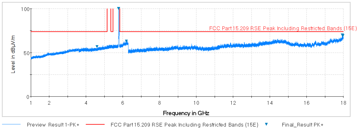
Plot 7-20. Radiated Spurious Plot above 1GHz (802.11a – U3 Ch. 157, Ant. Pol. V)
