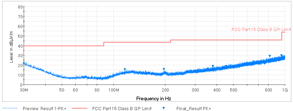
Plot 7-38. Radiated Spurious Plot below 1GHz (802.11a – U3 Ch. 157, Ant. Pol. V)
