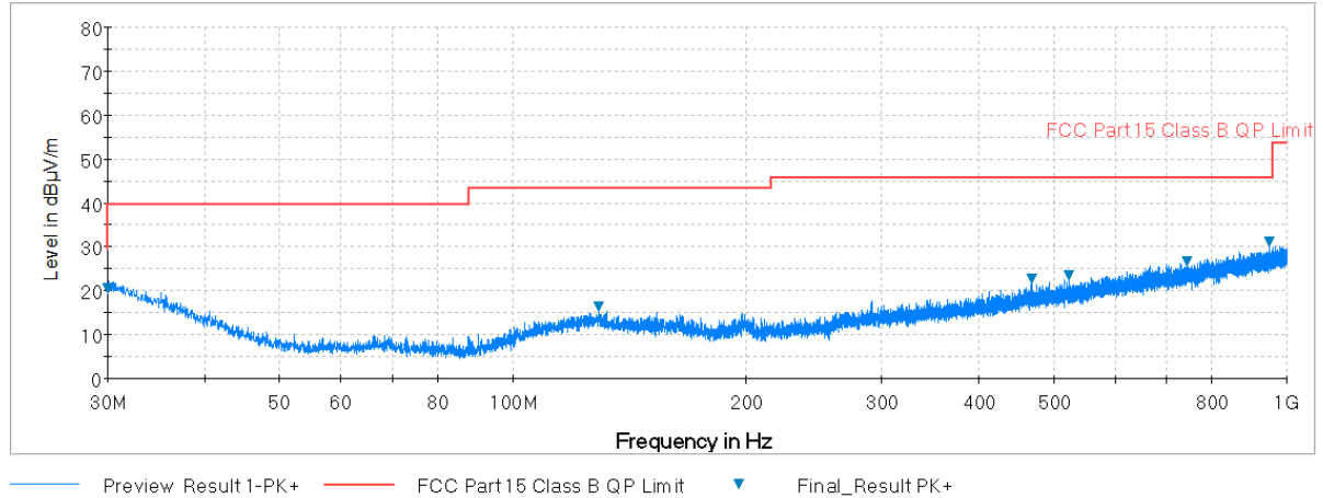
Plot 7-39. Radiated Spurious Plot below 1GHz (802.11a – U3 Ch. 157, Ant. Pol. H)
