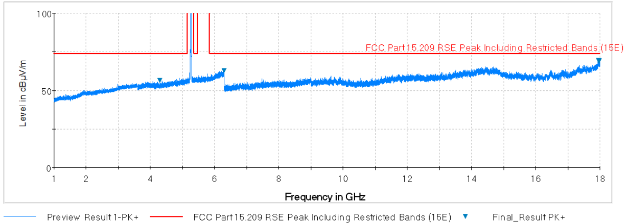
Plot 7-16. Radiated Spurious Plot above 1GHz (802.11a – U2A Ch. 56, Ant. Pol. V)
