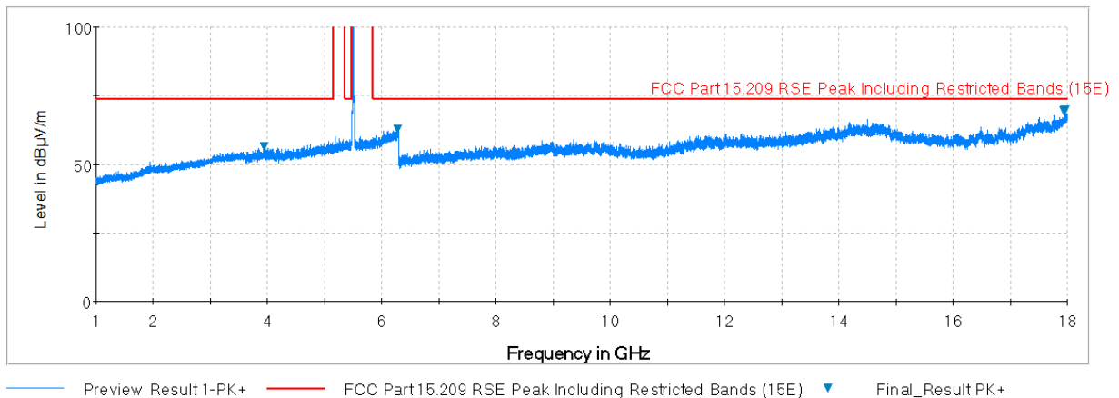
Plot 7-17. Radiated Spurious Plot above 1GHz (802.11a – U2C Ch. 116, Ant. Pol. H)
