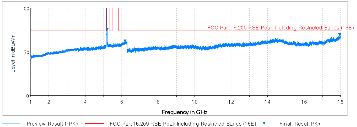
Plot 7-13. Radiated Spurious Plot above 1GHz (802.11a – U1 Ch. 40, Ant. Pol. H)
