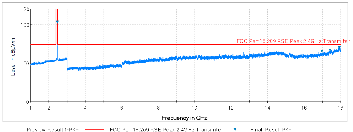
Plot 7-74. Radiated Spurious Plot above 1GHz (802.11b – Ch. 11, Ant. Pol. V)
