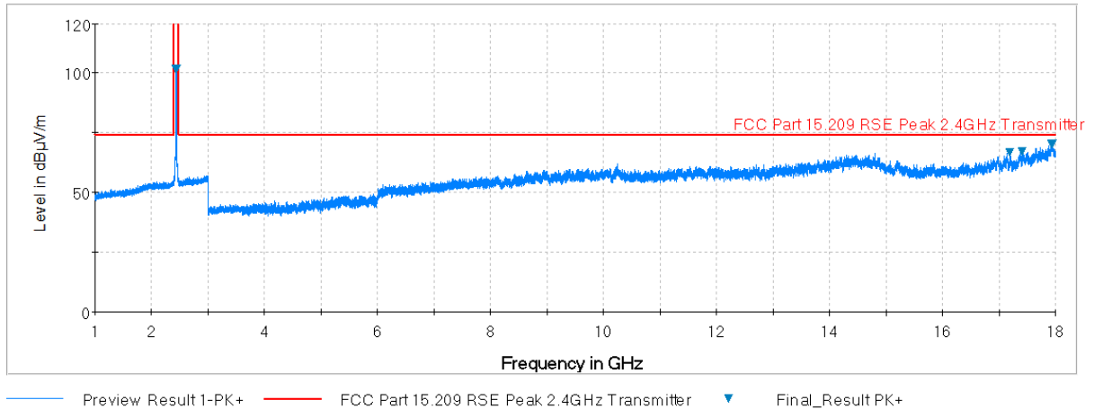
Plot 7-72. Radiated Spurious Plot above 1GHz (802.11b – Ch. 6, Ant. Pol. V)
