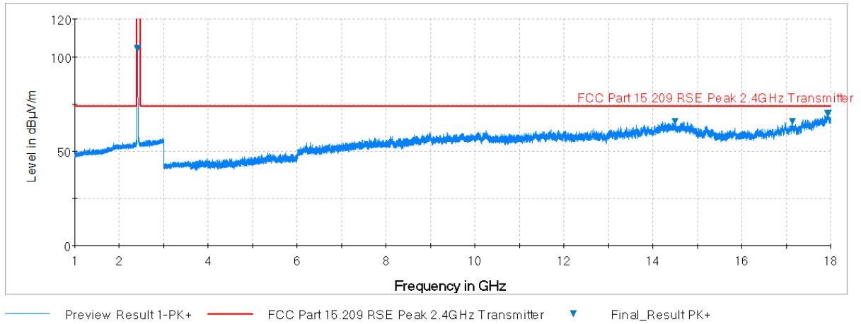
Plot 7-69. Radiated Spurious Plot above 1GHz (802.11b – Ch. 1, Ant. Pol. H)
