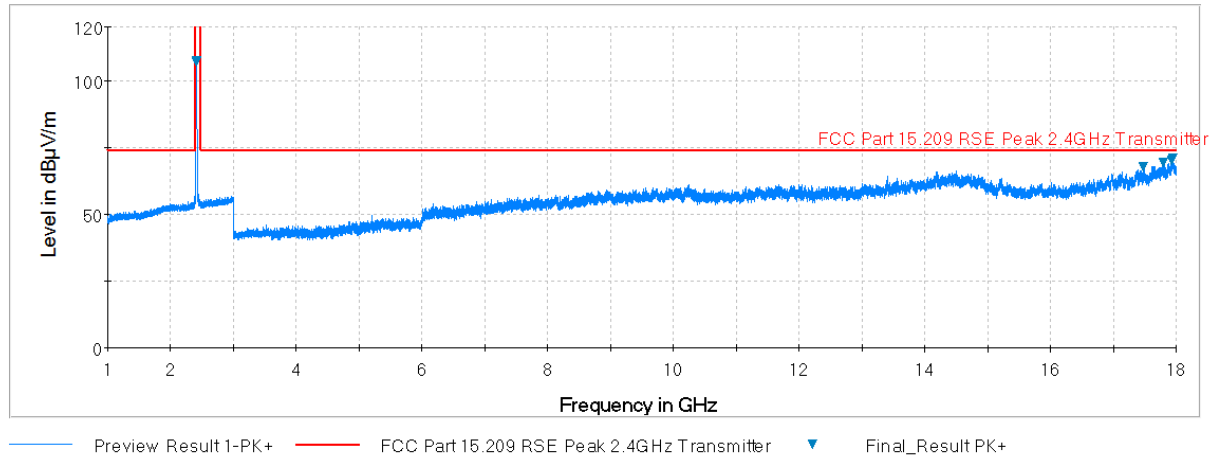
Plot 7-61. Radiated Spurious Plot above 1GHz (802.11b – Ch. 1, Ant. Pol. H)
