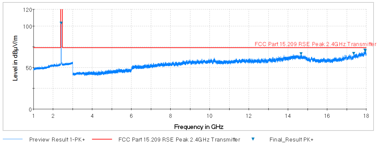
Plot 7-62. Radiated Spurious Plot above 1GHz (802.11b – Ch. 1, Ant. Pol. V)
