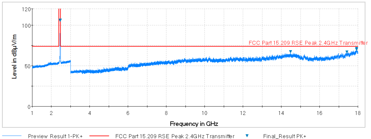
Plot 7-65. Radiated Spurious Plot above 1GHz (802.11b – Ch. 11, Ant. Pol. H)
