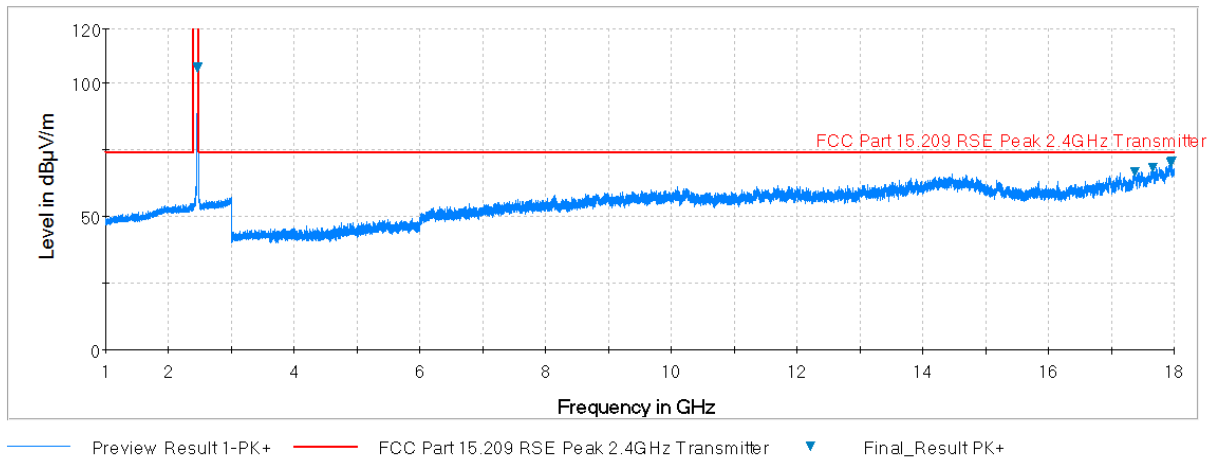
Plot 7-73. Radiated Spurious Plot above 1GHz (802.11b – Ch. 11, Ant. Pol. H)
