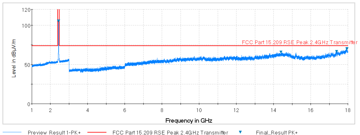
Plot 7-63. Radiated Spurious Plot above 1GHz (802.11b – Ch. 6, Ant. Pol. H)
