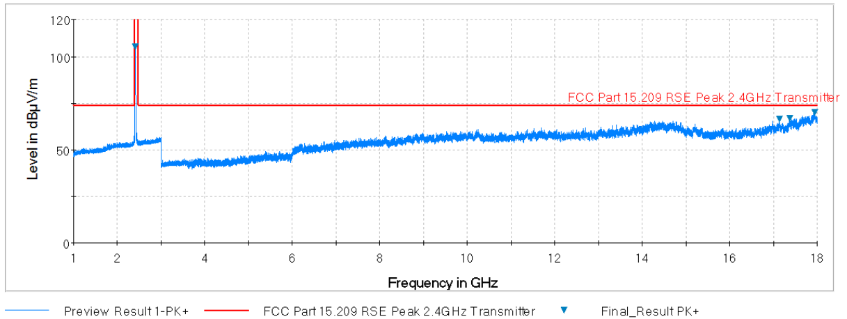
Plot 7-70. Radiated Spurious Plot above 1GHz (802.11b – Ch. 1, Ant. Pol. V)
