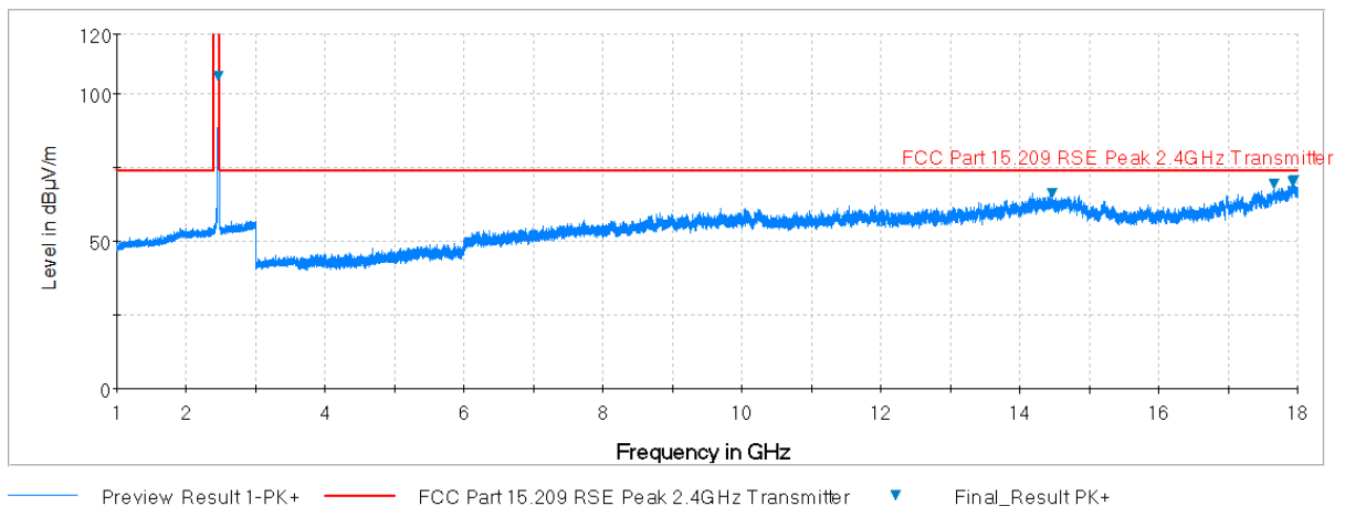
Plot 7-66. Radiated Spurious Plot above 1GHz (802.11b – Ch. 11, Ant. Pol. V)
