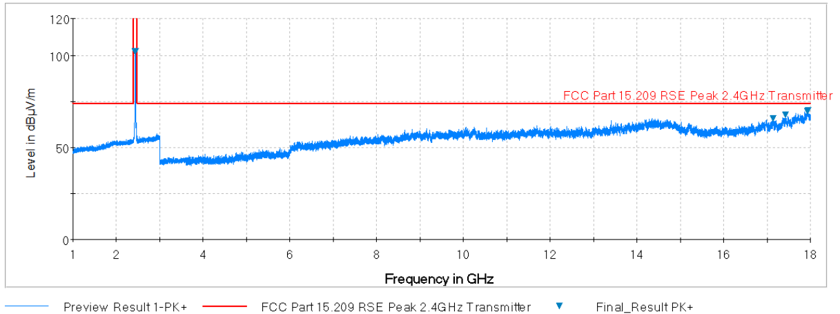
Plot 7-64. Radiated Spurious Plot above 1GHz (802.11b – Ch. 6, Ant. Pol. V)
