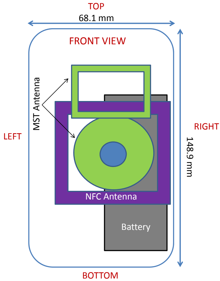
Figure F-2 NFC and MST Antenna Locations
