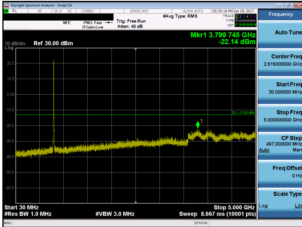
Plot 7-18. Conducted Spurious Plot (10MHz QPSK – RB Size 1, RB Offset 0 – High Channel)
