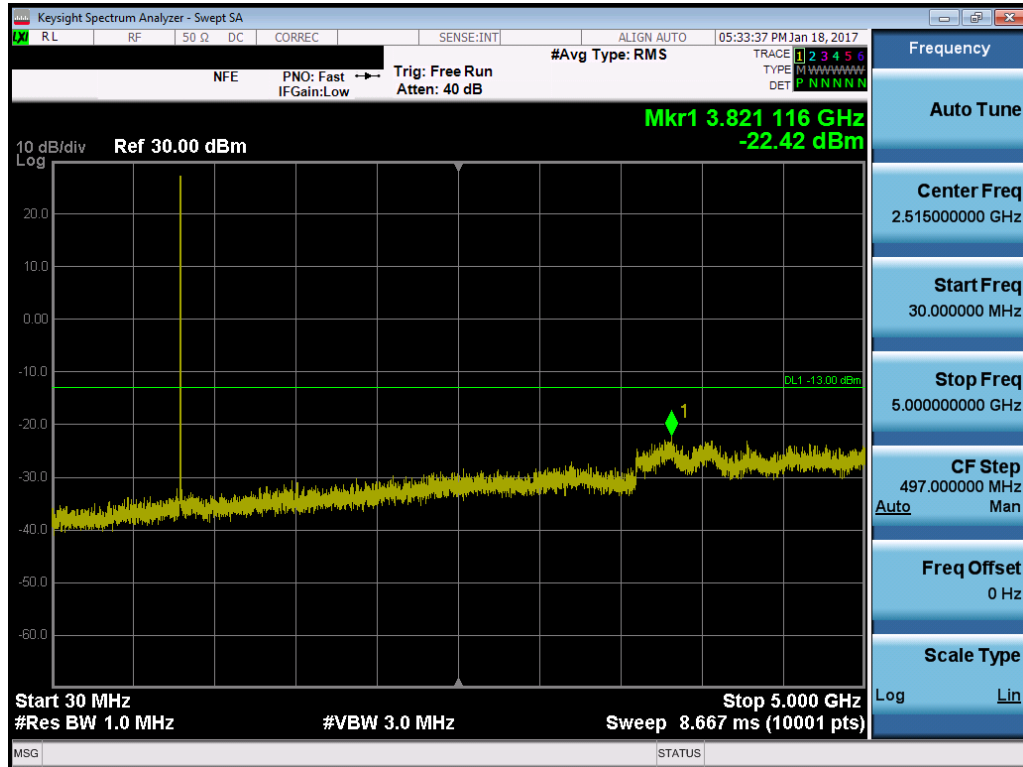
Plot 7-16. Conducted Spurious Plot (10MHz QPSK – RB Size 1, RB Offset 0 – Low Channel)
