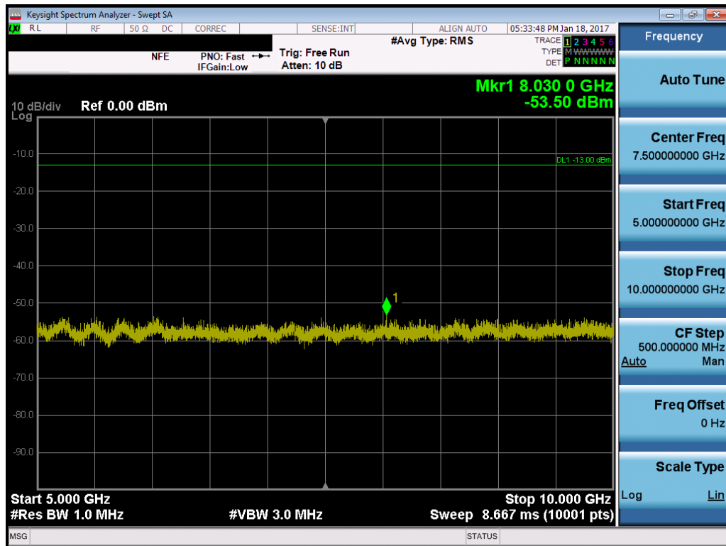
Plot 7-17. Conducted Spurious Plot (10MHz QPSK – RB Size 1, RB Offset 0 – Low Channel)
