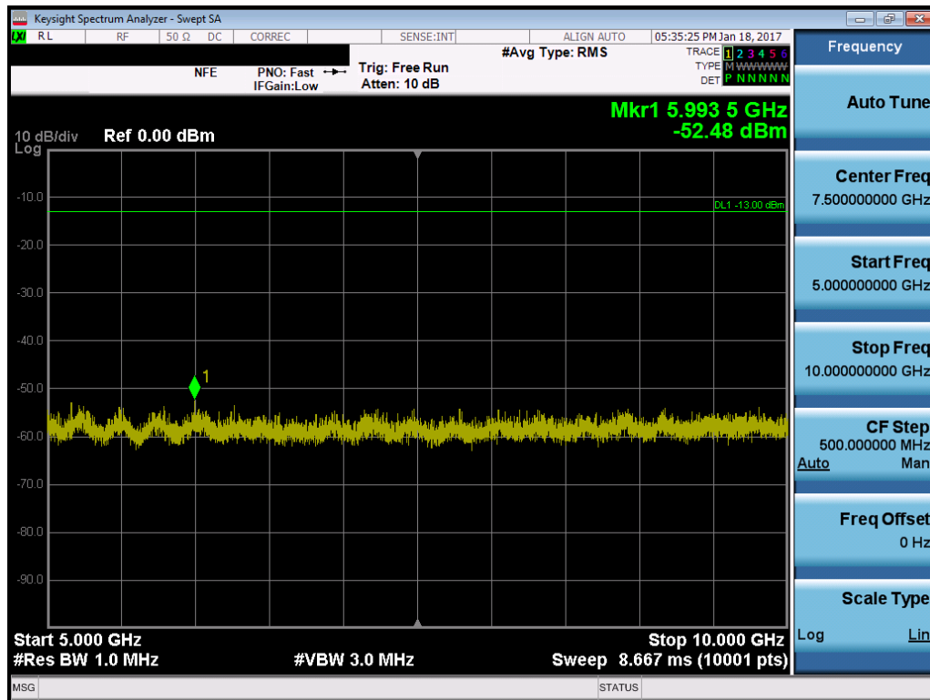
Plot 7-19. Conducted Spurious Plot (10MHz QPSK – RB Size 1, RB Offset 0 – High Channel)
