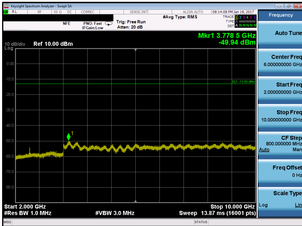
Plot 7-37. Conducted Spurious Plot (Cellular WCDMA Mode – Ch. 4132)
