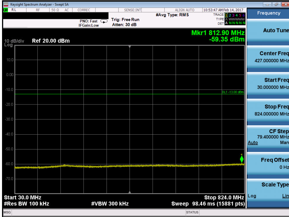
Plot 7-32. Conducted Spurious Plot (Cellular CDMA Mode – Ch. 777)
