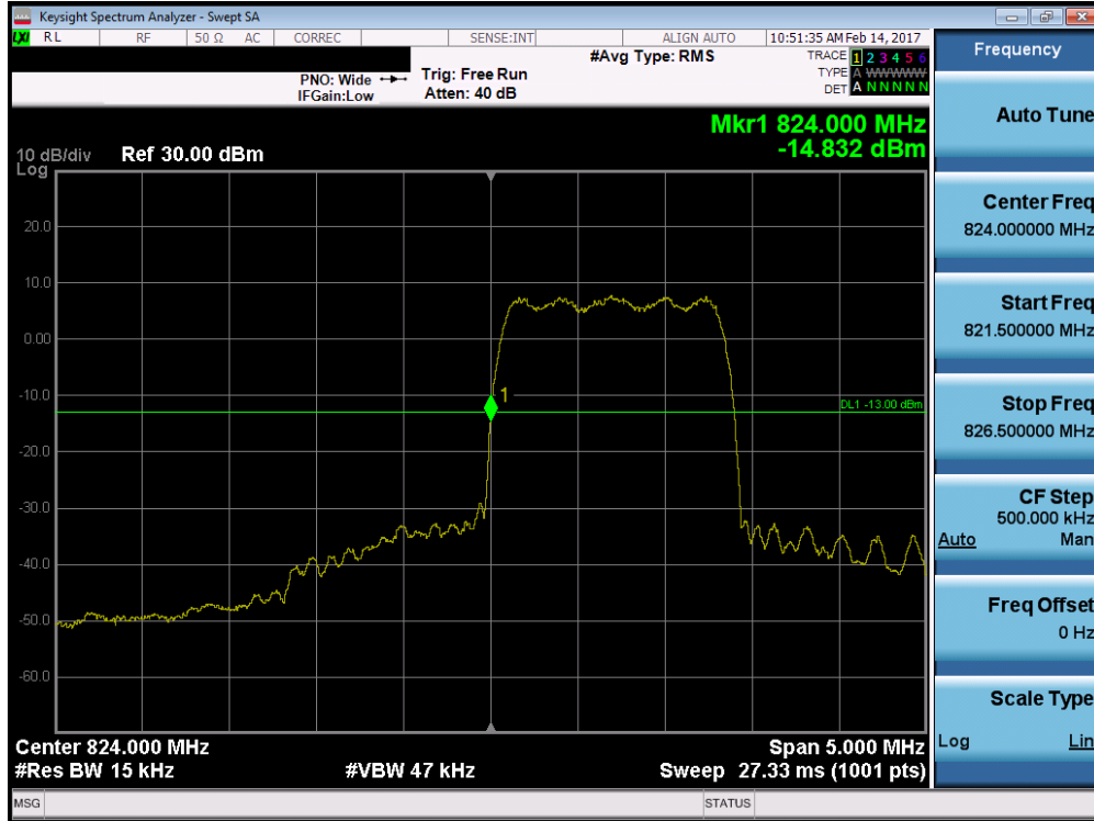
Plot 7-59. Band Edge Plot (Cellular CDMA Mode – Ch. 1013)
