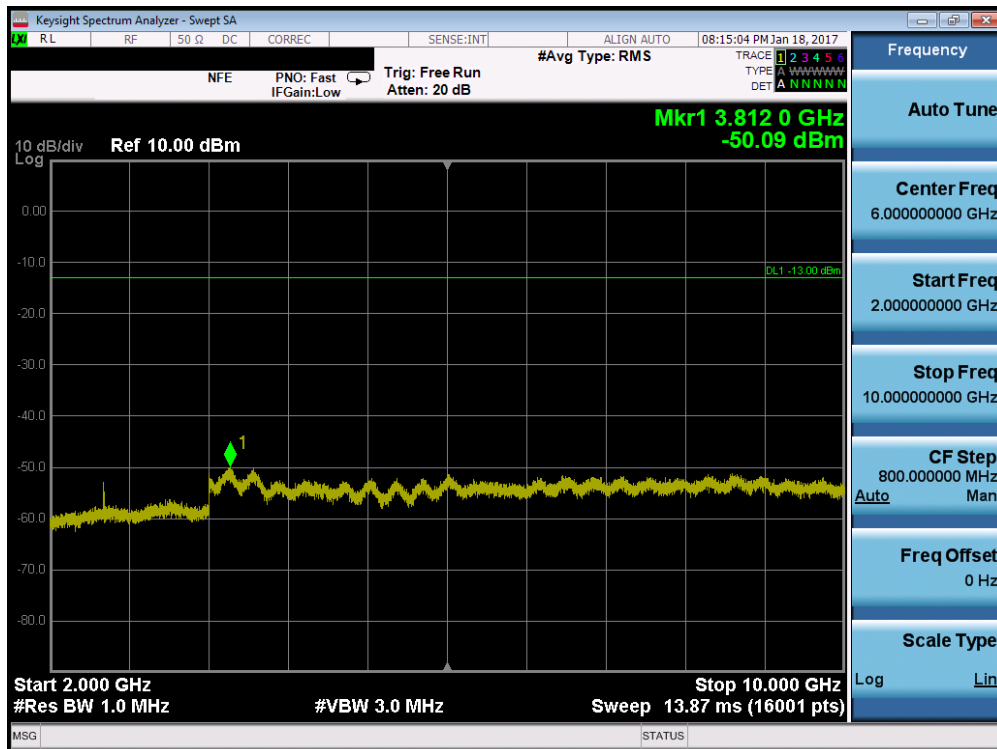
Plot 7-43. Conducted Spurious Plot (Cellular WCDMA Mode – Ch. 4233)
