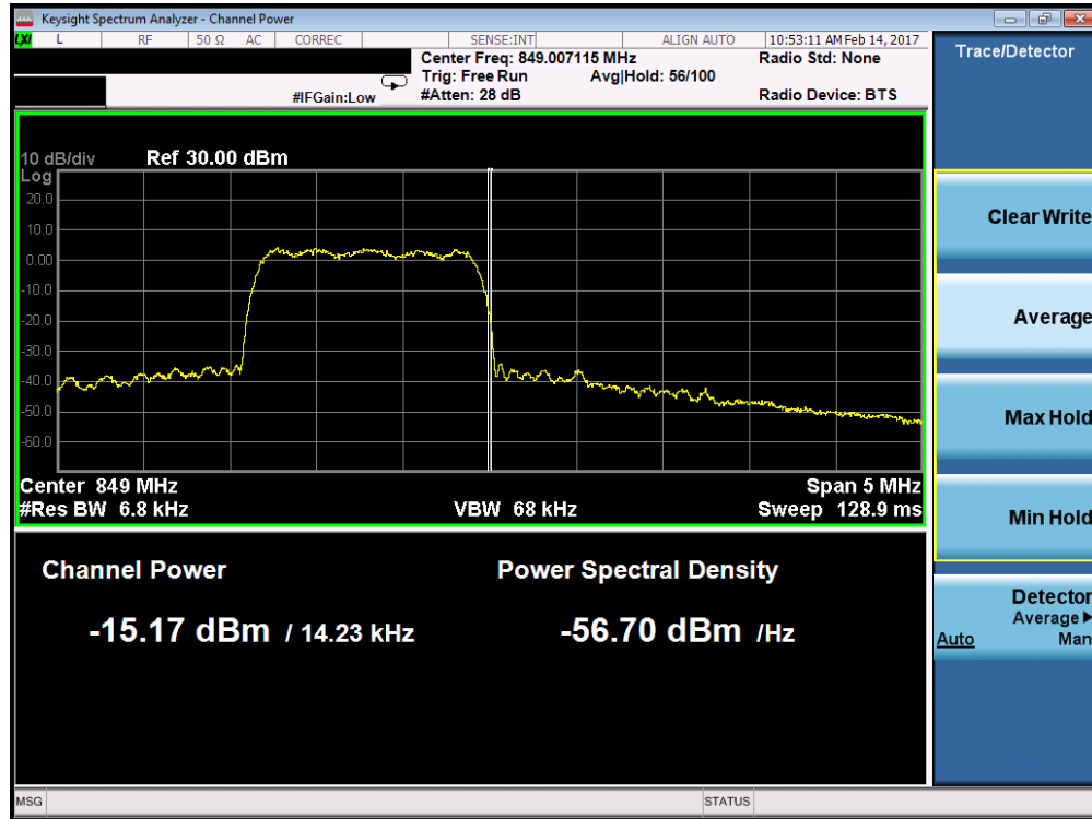
Plot 7-61. Band Edge Plot (Cellular CDMA Mode – Ch. 777)
