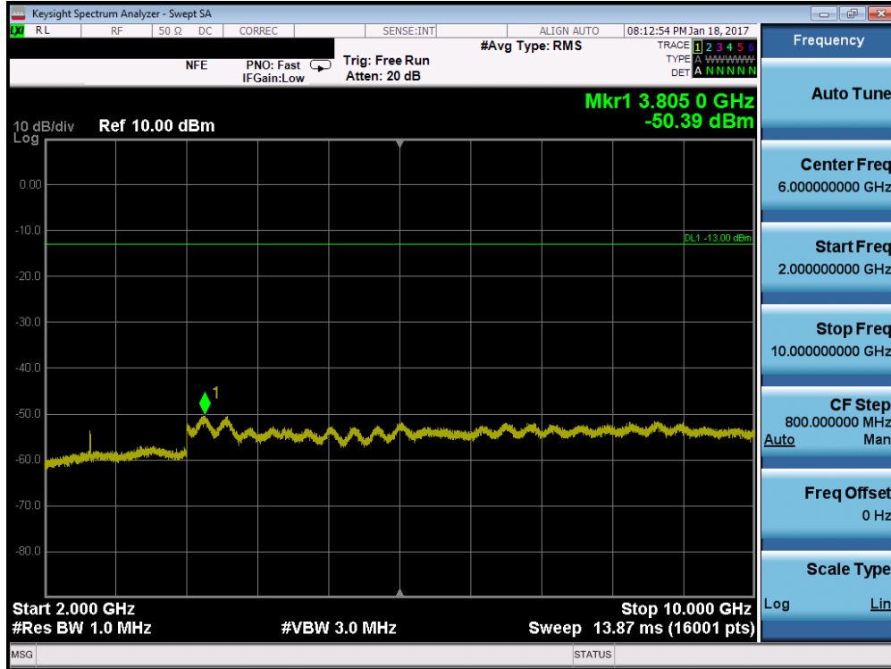
Plot 7-40. Conducted Spurious Plot (Cellular WCDMA Mode – Ch. 4183)
