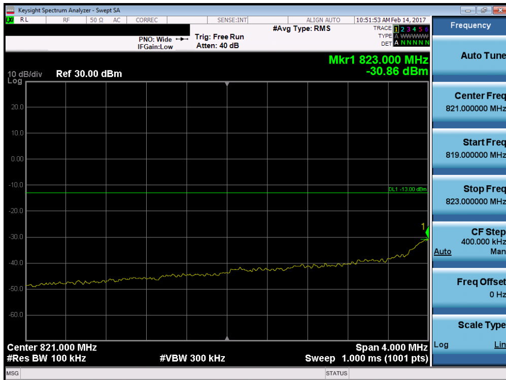
Plot 7-60. 4MHz Span Plot (Cellular CDMA Mode – Ch. 1013)
