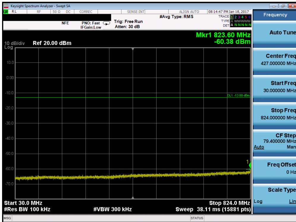
Plot 7-41. Conducted Spurious Plot (Cellular WCDMA Mode – Ch. 4233)
