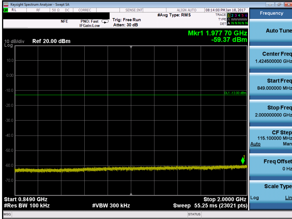
Plot 7-36. Conducted Spurious Plot (Cellular WCDMA Mode – Ch. 4132)
