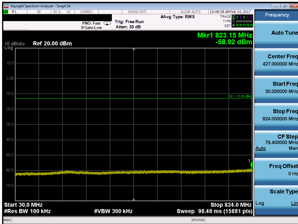
Plot 7-29. Conducted Spurious Plot (Cellular CDMA Mode – Ch. 384)
