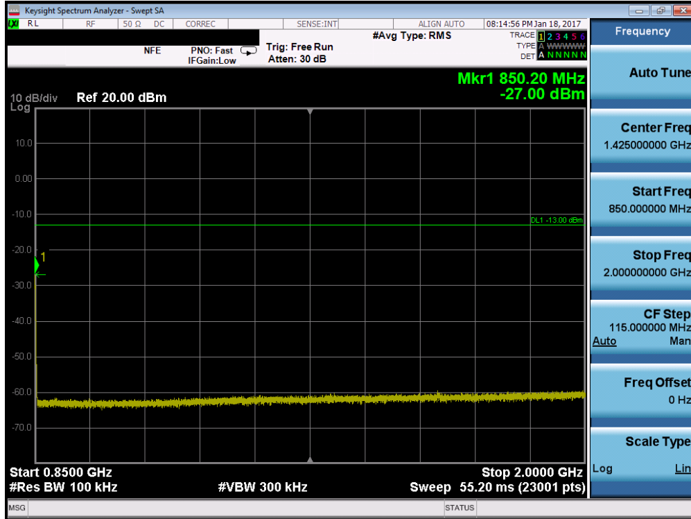
Plot 7-42. Conducted Spurious Plot (Cellular WCDMA Mode – Ch. 4233)
