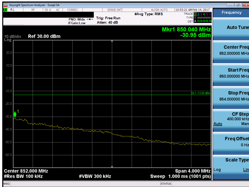
Plot 7-62. 4MHz Span Plot (Cellular CDMA Mode – Ch. 777)
