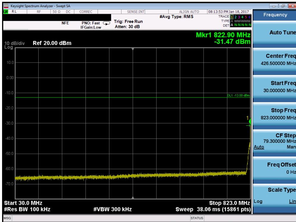
Plot 7-35. Conducted Spurious Plot (Cellular WCDMA Mode – Ch. 4132)
