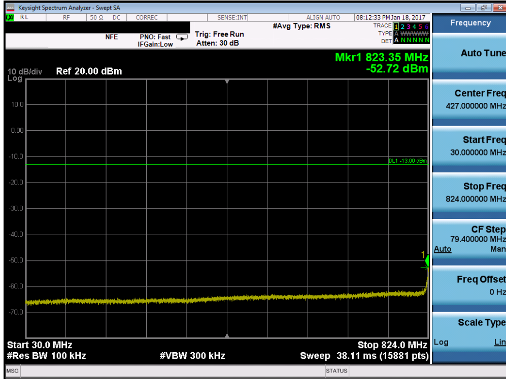
Plot 7-38. Conducted Spurious Plot (Cellular WCDMA Mode – Ch. 4183)
