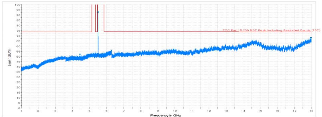
Plot 7-17. Radiated Spurious Plot above 1GHz (802.11a – U2C Ch. 116, Ant. Pol. H)
