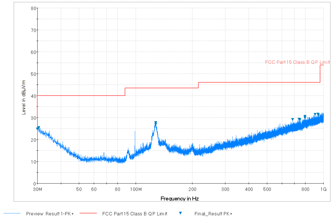
Plot 7-43. Radiated Spurious Plot below 1GHz (802.11a – U3 Ch. 157, Ant. Pol. H)
