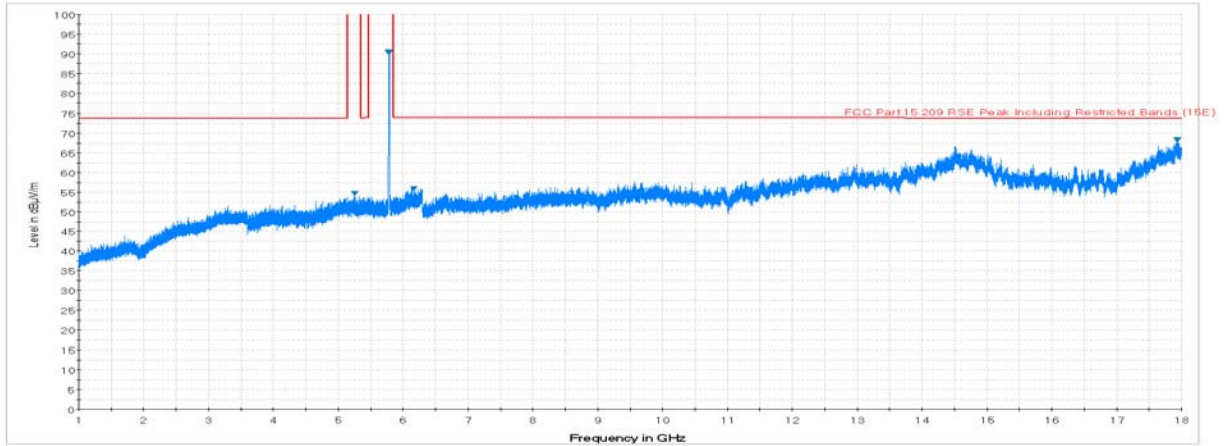
Plot 7-19. Radiated Spurious Plot above 1GHz (802.11a – U3 Ch. 157, Ant. Pol. H)
