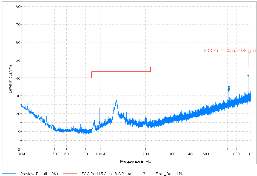
Plot 7-46. Radiated Spurious Plot below 1GHz (802.11a – U3 Ch. 157, Ant. Pol. V)
