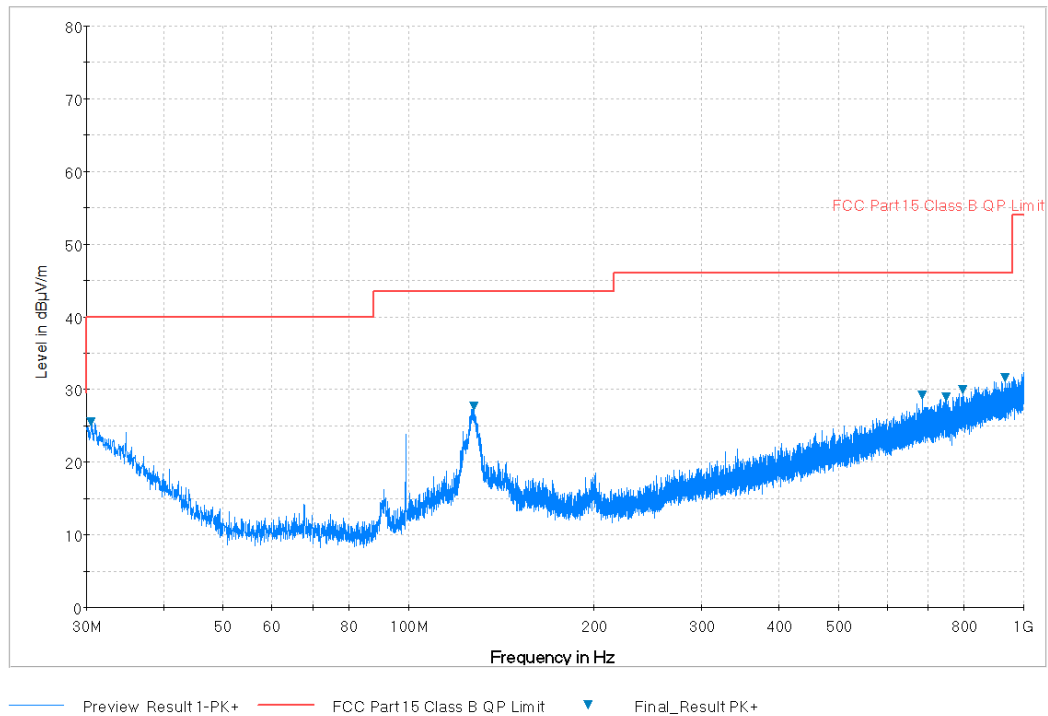
Plot 7-44. Radiated Spurious Plot below 1GHz (802.11a – U3 Ch. 157, Ant. Pol. V)
