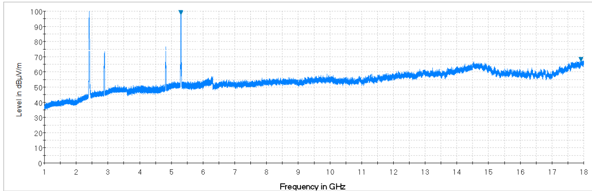
Plot 7-29. Radiated Spurious Plot above 1GHz (Ant1: 2.4 - 5GHz Ant2: 2.4 - 5GHz, Ant. Pol. H)
