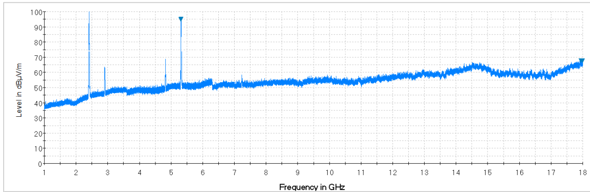
Plot 7-28. Radiated Spurious Plot above 1GHz (5GHz – 2.4 GHz, Ant. Pol. V)
