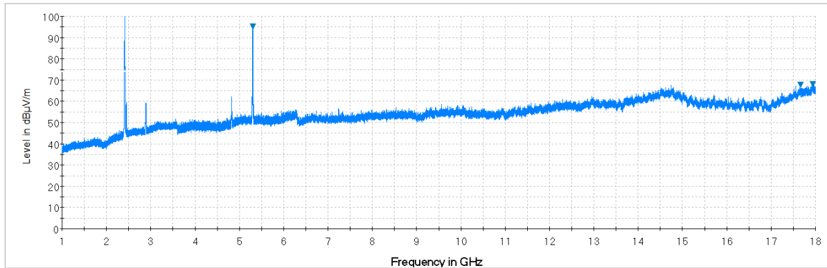
Plot 7-30. Radiated Spurious Plot above 1GHz (Ant1: 2.4 - 5GHz Ant2: 2.4 - 5GHz, Ant. Pol. V)
