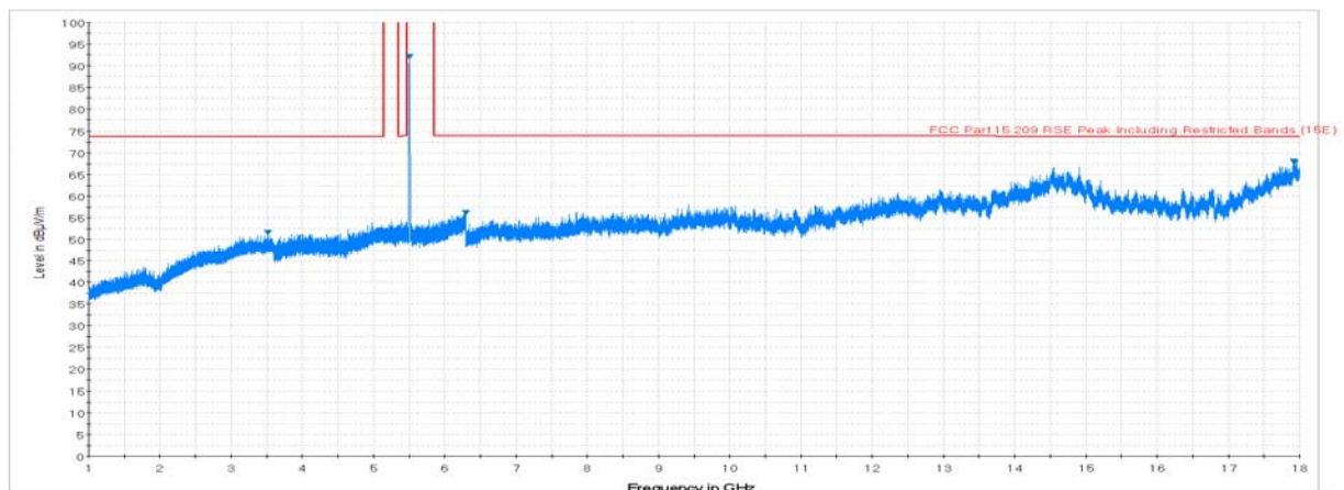
Plot 7-18. Radiated Spurious Plot above 1GHz (802.11a – U2C Ch. 116, Ant. Pol. V)
