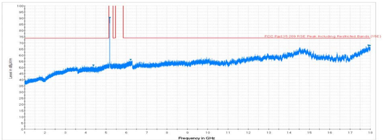
Plot 7-14. Radiated Spurious Plot above 1GHz (802.11a – U1 Ch. 40, Ant. Pol. V)
