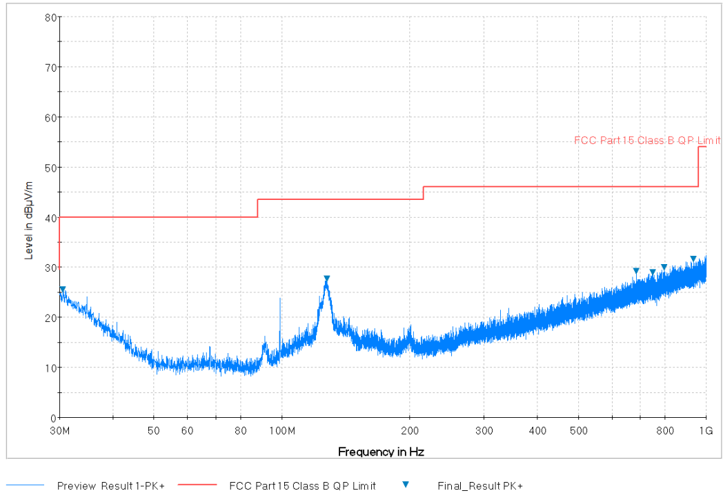
Plot 7-45. Radiated Spurious Plot below 1GHz (802.11a – U3 Ch. 157, Ant. Pol. H)
