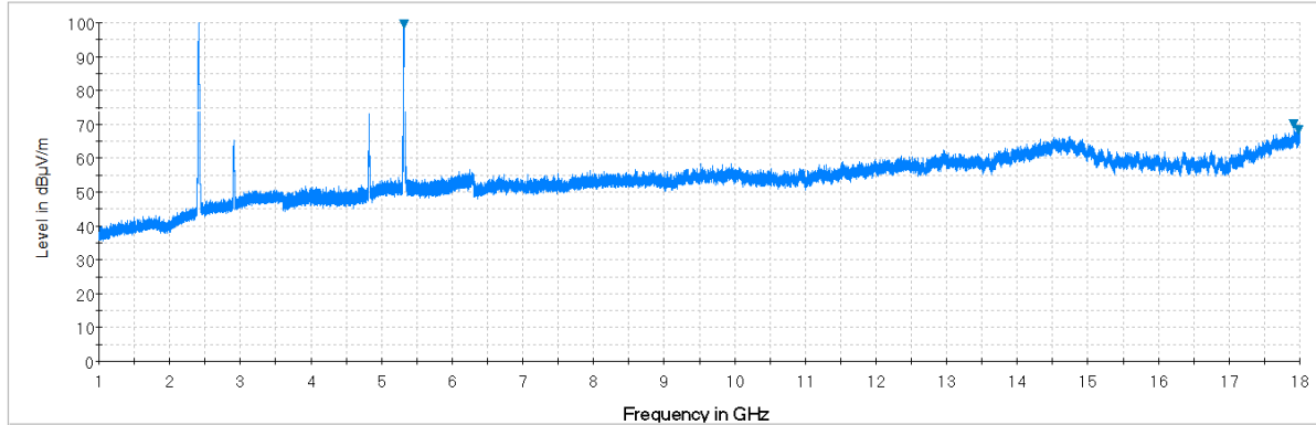
Plot 7-27. Radiated Spurious Plot above 1GHz (5GHz – 2.4 GHz, Ant. Pol. H)
