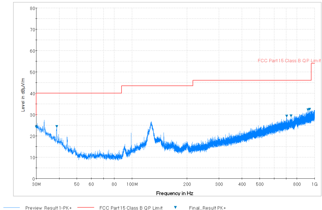
Plot 7-14. Radiated Spurious Plot below 1GHz (Pol. V)
