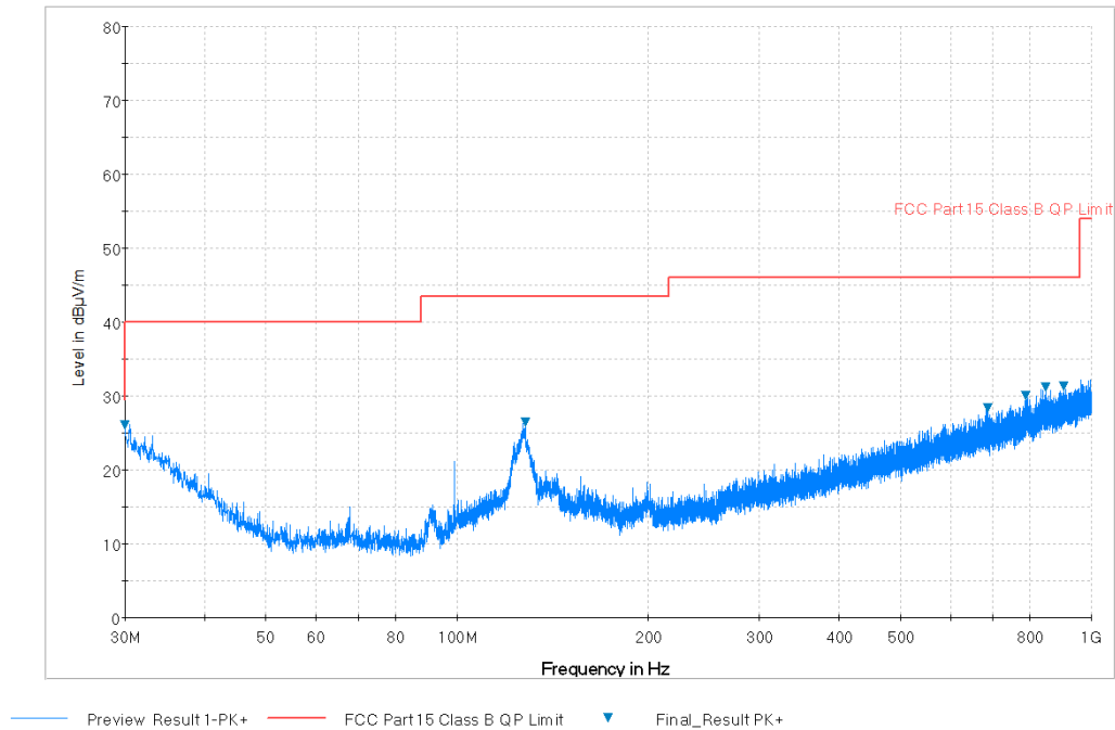
Plot 7-13. Radiated Spurious Plot below 1GHz (Pol. H)
