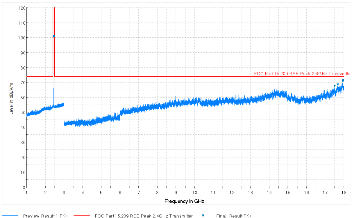
Plot 7-78. Radiated Spurious Plot above 1GHz (802.11b – Ch. 11, Ant. Pol. V)
