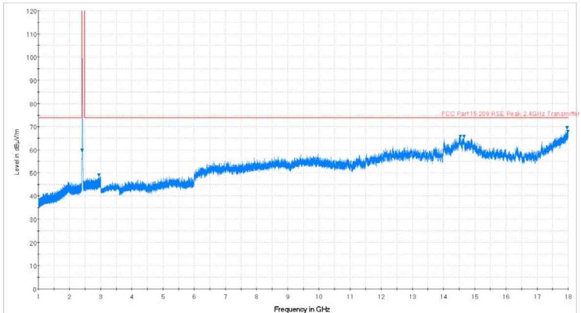
Plot 7-81. Radiated Spurious Plot above 1GHz (802.11b – Ch. 1, Ant. Pol. H)
