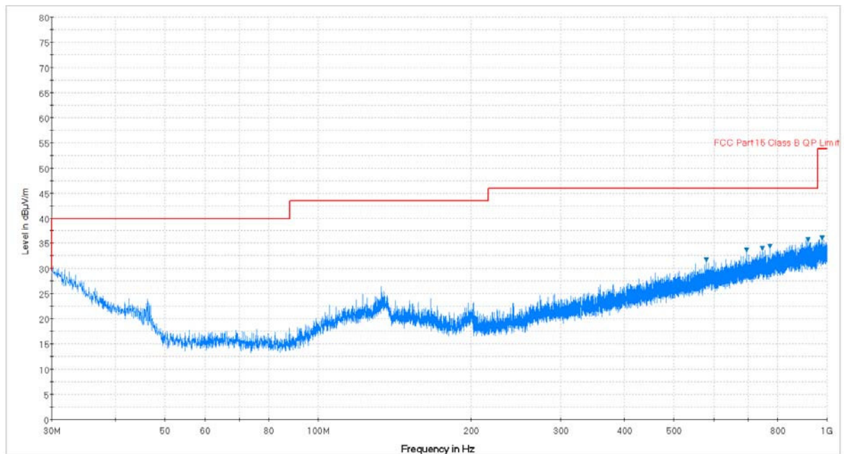
Plot 7-120. Radiated Spurious Plot below 1GHz (Pol. V)
