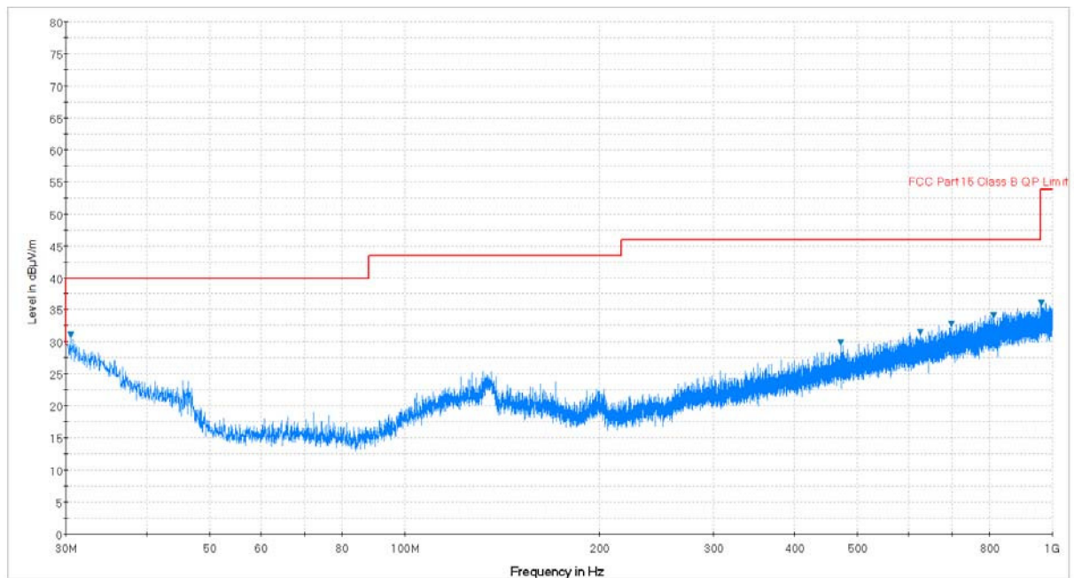
Plot 7-122. Radiated Spurious Plot below 1GHz (Pol. V)
