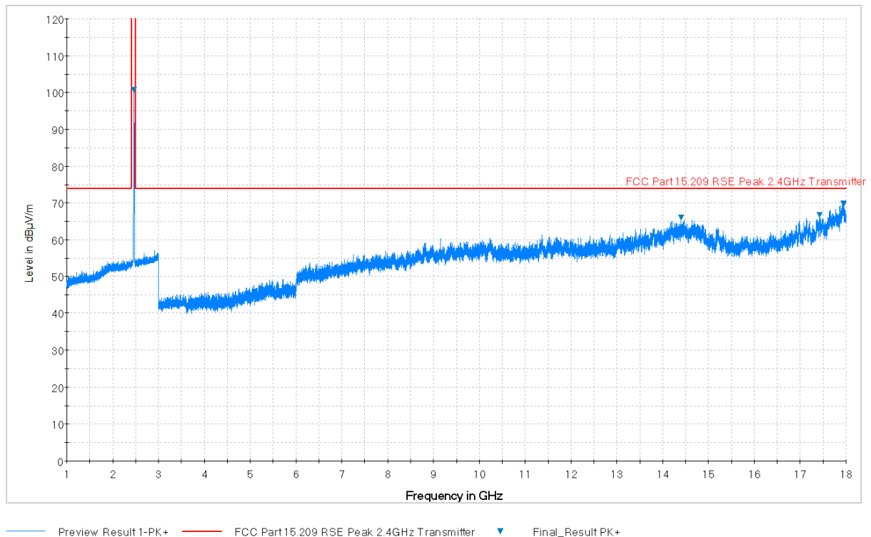
Plot 7-86. Radiated Spurious Plot above 1GHz (802.11b – Ch. 11, Ant. Pol. V)
