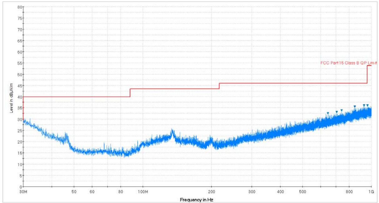
Plot 7-121. Radiated Spurious Plot below 1GHz (Pol. H)
