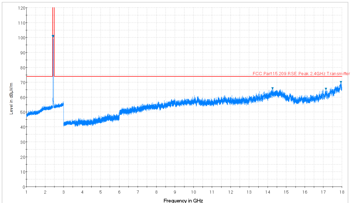
Plot 7-76. Radiated Spurious Plot above 1GHz (802.11b – Ch. 6, Ant. Pol. V)
