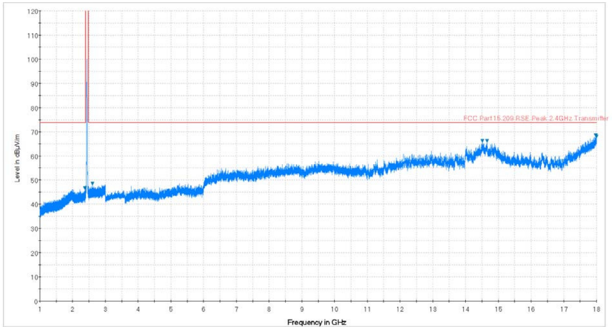
Plot 7-83. Radiated Spurious Plot above 1GHz (802.11b – Ch. 6, Ant. Pol. H)
