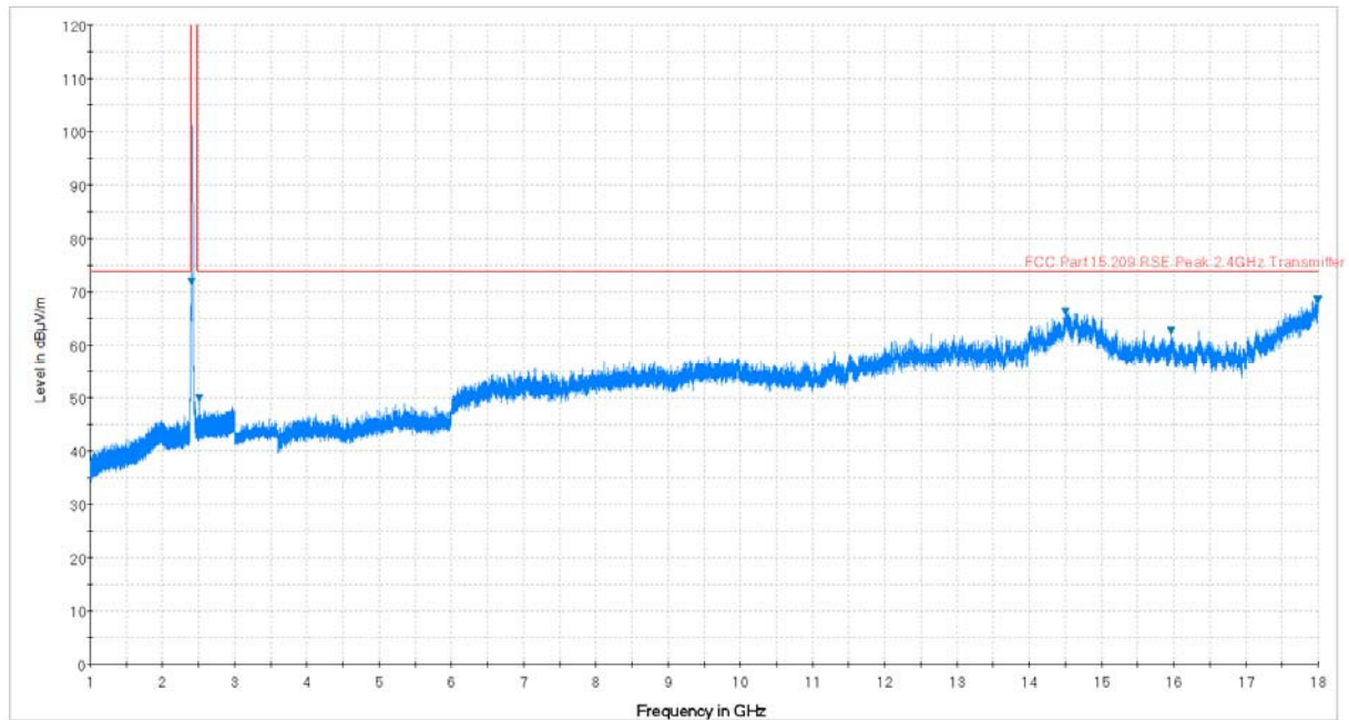
Plot 7-73. Radiated Spurious Plot above 1GHz (802.11b – Ch. 1, Ant. Pol. H)
