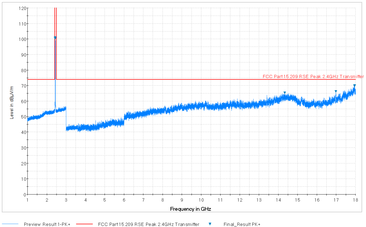
Plot 7-84. Radiated Spurious Plot above 1GHz (802.11b – Ch. 6, Ant. Pol. V)
