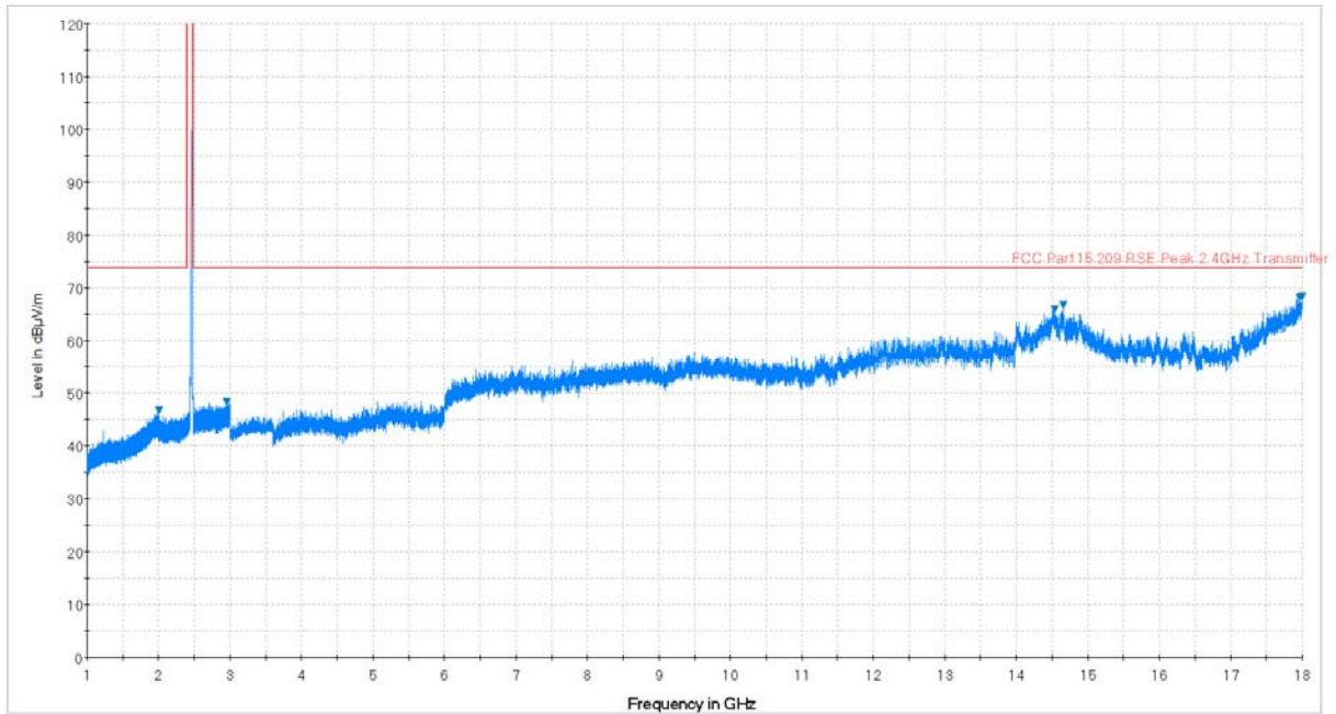
Plot 7-77. Radiated Spurious Plot above 1GHz (802.11b – Ch. 11, Ant. Pol. H)
