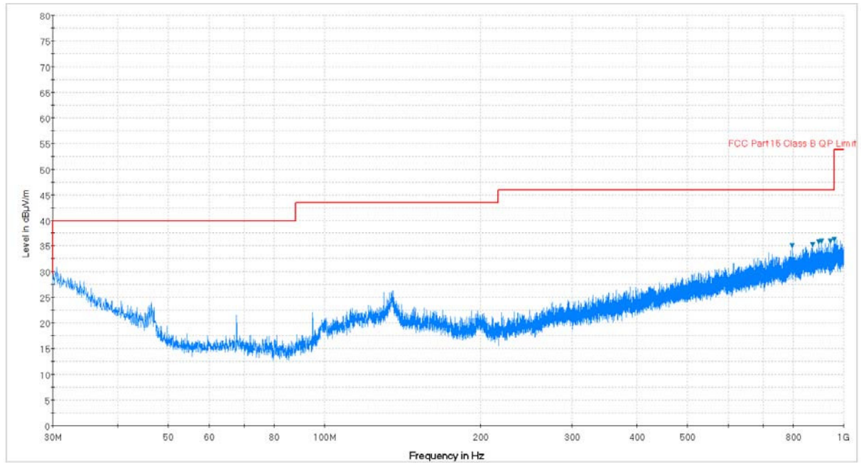
Plot 7-119. Radiated Spurious Plot below 1GHz (Pol. H)
