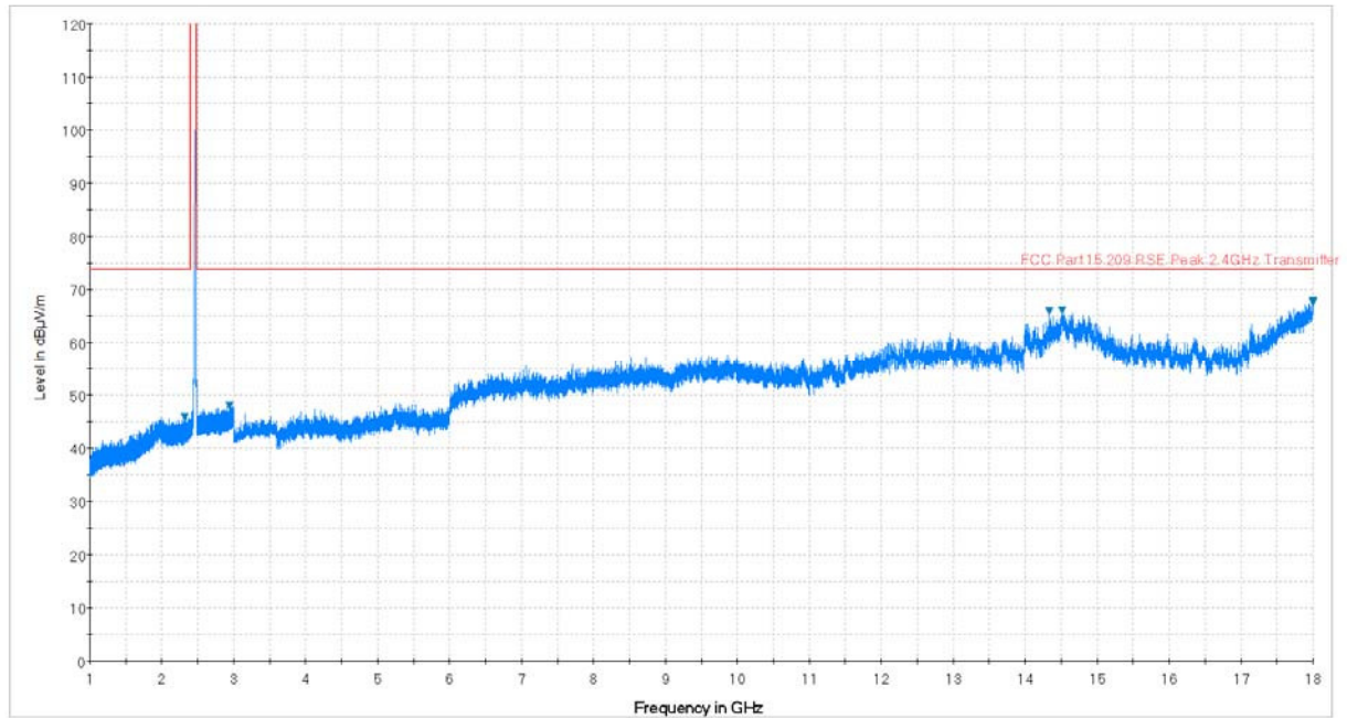
Plot 7-85. Radiated Spurious Plot above 1GHz (802.11b – Ch. 11, Ant. Pol. H)
