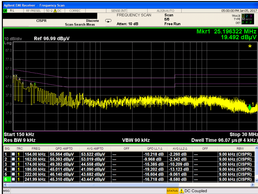
Plot 7-124. Line Conducted Plot with 802.11b (N)
