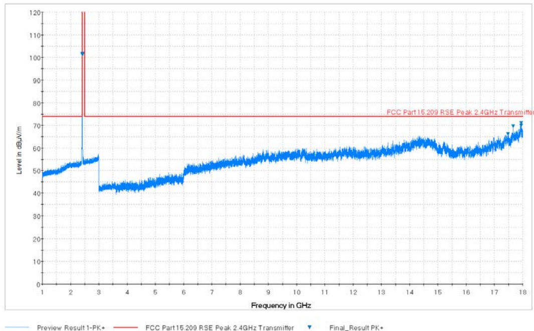
Plot 7-82. Radiated Spurious Plot above 1GHz (802.11b – Ch. 1, Ant. Pol. V)
