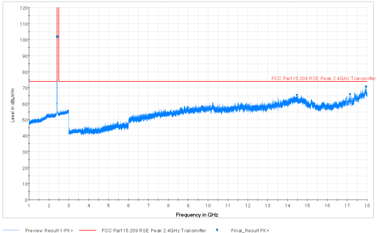
Plot 7-74. Radiated Spurious Plot above 1GHz (802.11b – Ch. 1, Ant. Pol. V)
