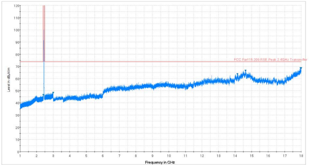
Plot 7-75. Radiated Spurious Plot above 1GHz (802.11b – Ch. 6, Ant. Pol. H)
