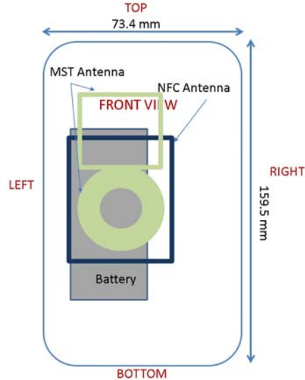
Figure F-2 MST and NFC Antenna Locations
